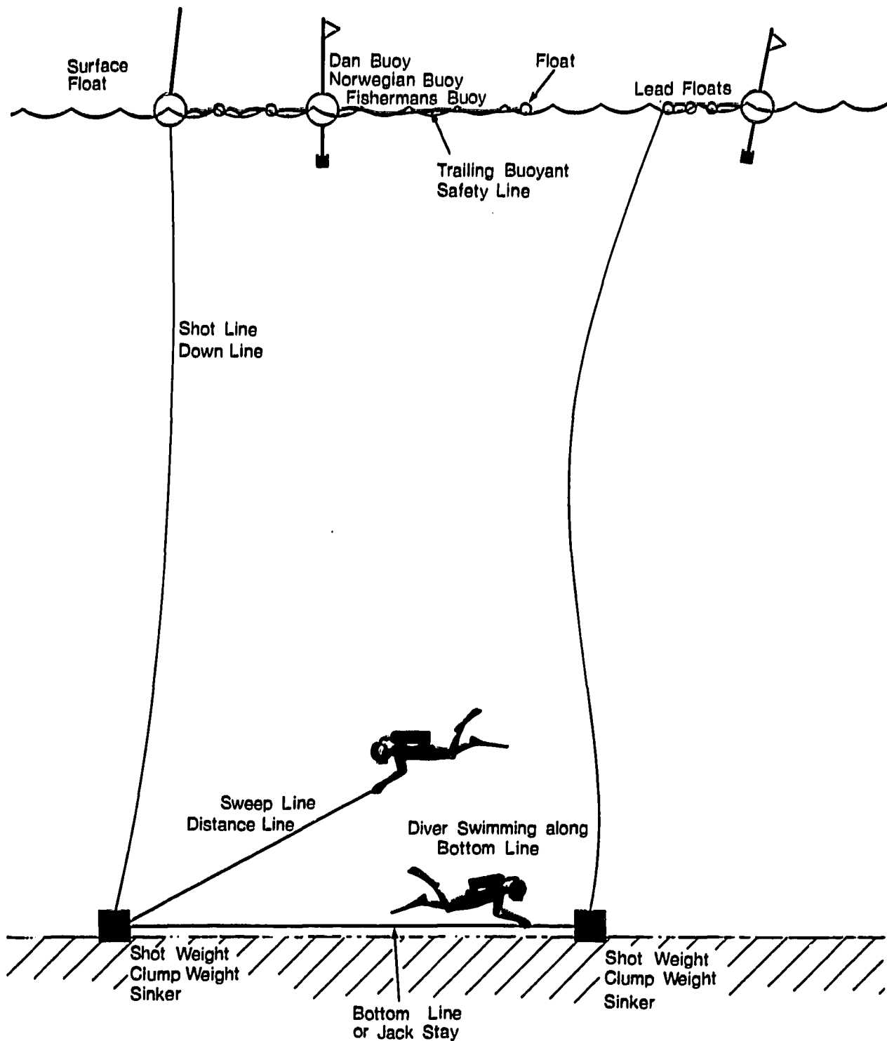
Fig. 6.2.7.a. Divers working from ropes and lines that allow the divers to work on or up from the bottom. Common names for the different types of ropes are given, with alternate names.
