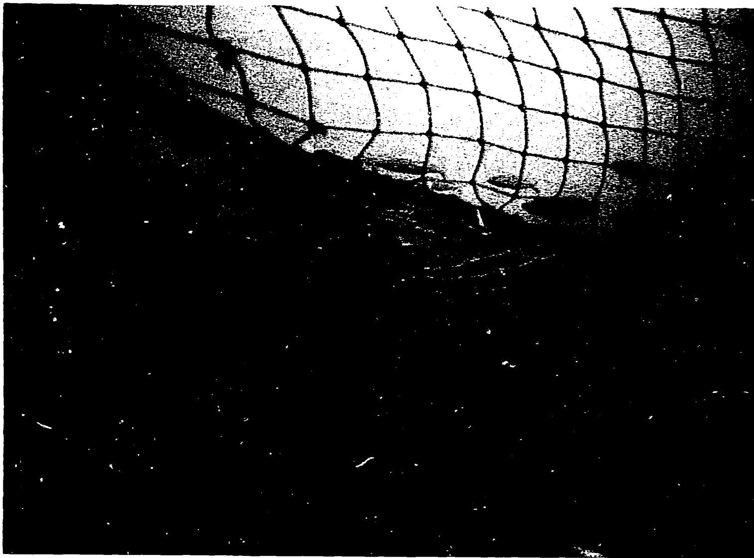
Photo 13 : This close-up picture of a trawl in action shows the behaviour of the fish in the mouth of the trawl. (Marine Laboratory, Aberdeen).
