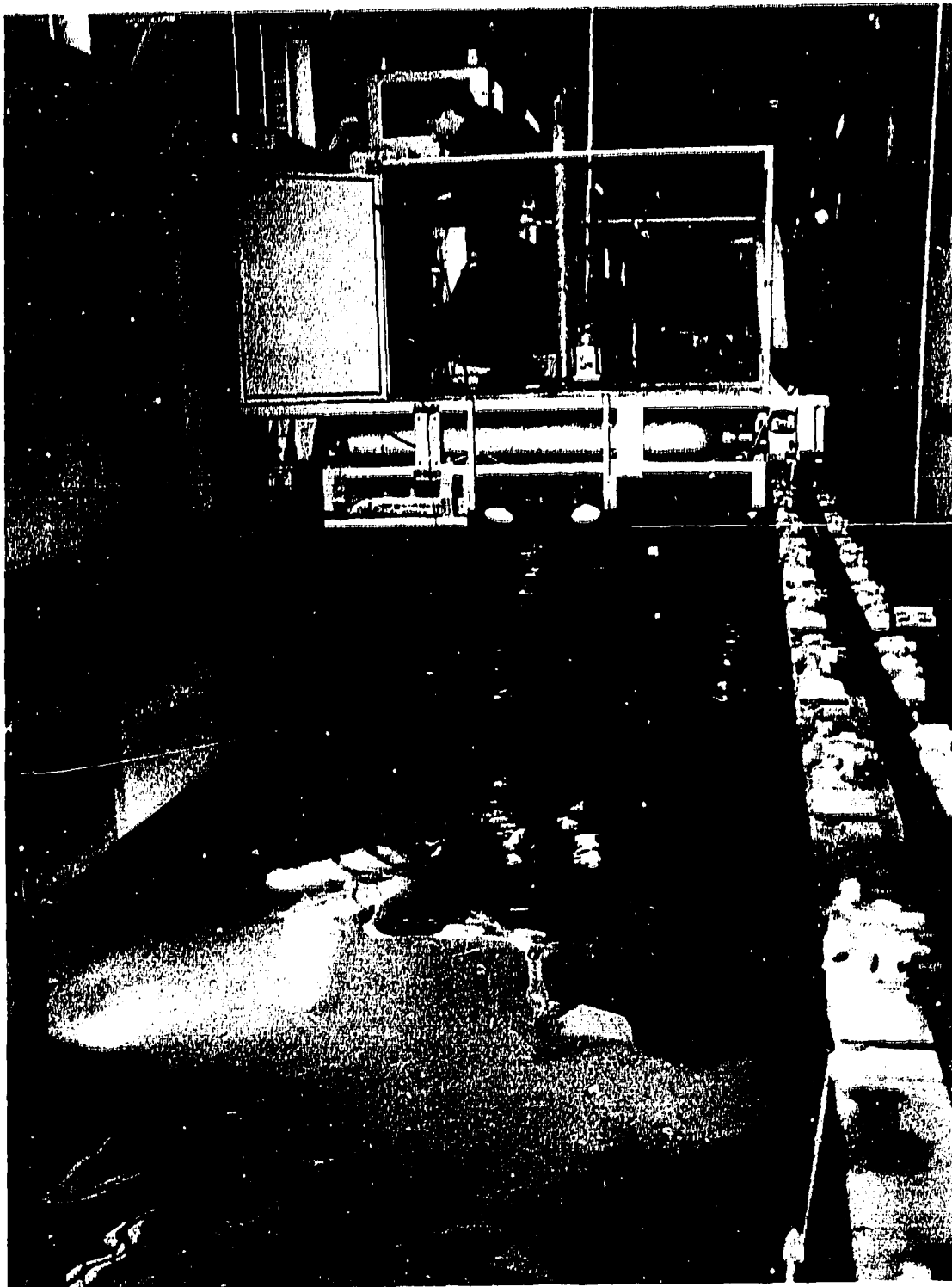
Photo 8 : In preparation for scientific work at sea it is sometimes necessary for divers to work in laboratory tanks to test equipment and procedures. In this picture the diver can be seen working underwater whilst an experimental communications and monitoring system connects him to an observer on the surface. The instrument chariot runs on rails, and for some tests the divers swam along the tank whilst the recording instruments tracked them from above. (Photo, IOSDL).
