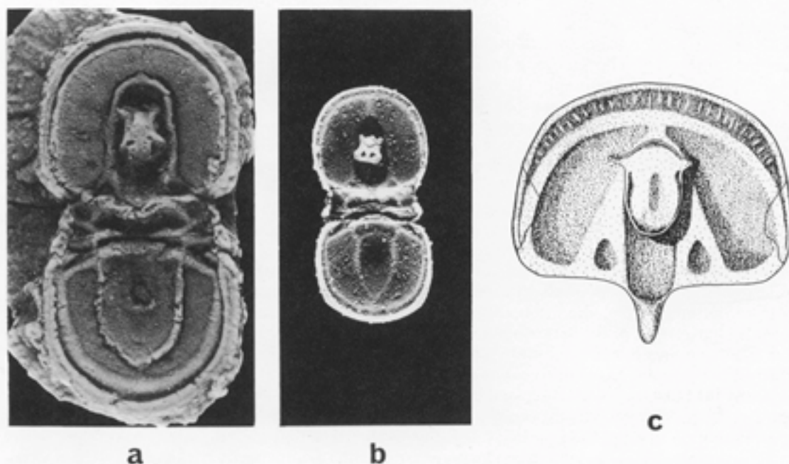
TEXT-FIG. 13. Natant hypostomal condition in Agnostida, showing no indication of rostrum. Agnostina: a , Peronopsis ferox (Tullberg) (Robison 1972a, fig. 2d) \times 21 ; b , Onymagnostus seminula (Whitehouse), (Robison 1982, pl. 4, fig. 5b), \times 10 ; photographs kindly supplied by R. A. Robison. Eodiscina: c , Pagetia cephalic shield from underside (after Jell 1980, pl. 1, fig. 1).
