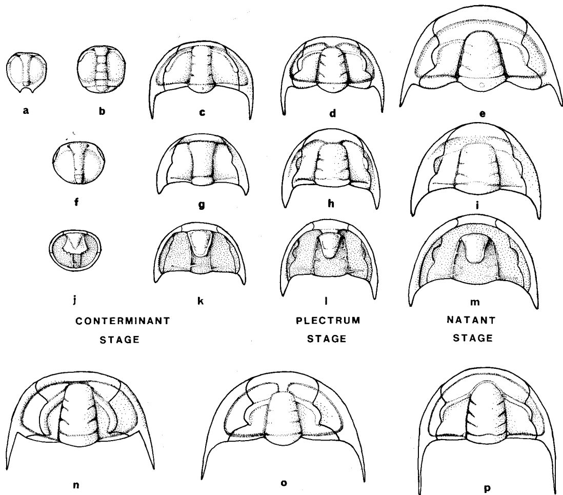
TEXT-FIG. 9. Natant hypostomal condition as a derived character. Ontogenies of typical ptychoparioids, showing change from conterminant to natant, by way of a plectrate stage. a-e , Ehmaniella waptaensis Rasetti (after Hu 1986, text-fig. 11), Middle Cambrian, Canada, dorsal views; a , small protaspis, \times 20 ; b , large protaspis, \times 16 ; c , meraspis cranidium c. \times 15 ; d , late meraspis, \times 5 ; e , holaspis, \times 5 . f-m , ontogeny of Crassifimbria (after Palmer 1958), Late Lower Cambrian, Nevada, dorsal ( f-i ) and ventral ( j-m ) views of comparable stages. The rostral form at the 'plectrum stage' is not yet described for this species, but is inferred from such specimens as that depicted by Zhang and Jell (1987, pl. 80, fig. 1 n-p ); the ontogenetic series is matched by adult cranidial morphologies among Lower Cambrian trilobites, which may record the evolutionary steps involved in the origin of natant groups; n , Redlichia (after Zhang et al. 1980); o , Dolerolenus (after Rasetti, 1972); p , Hamatolenus .
