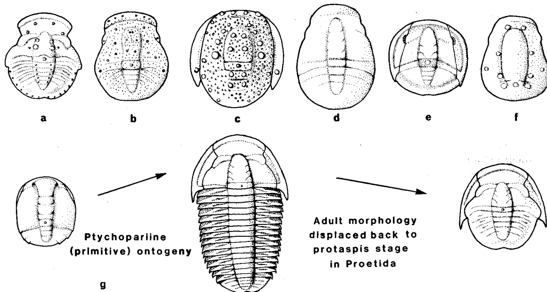
TEXT-FIG. 16. Late protaspides of various families within Proetida to show synapomorphy of tapering glabella (which falls short of border in these late protaspides); compare text-fig. 10 h-m . a , Scharyia (Scharyiinae; Aulacopleuridae) (after Šnajdr 1980, text-fig. 1 d ), \times 20 ; b , Phorocephala (Telephinidae) (after Chatterton 1980, fig. 5), \times 40 ; c , Dimeropyge (Dimeropygidae) (after Tripp and Evitt 1983, pl. 31, figs. 16–21), \times 40 ; d , Bathyurus (Bathyuridae) (after Chatterton 1980, fig. 5, and pl. 6, fig. 4), \times 25 ; e , Proetus (Proetidae) (after Chatterton 1971, fig. 15 c and d ), \times 20 ; f , Aulacopleura ? (Aulacopleurinae; Aulacopleuridae) (after Hu 1971, pl. 23, fig. 8; note: Hu assigned the species from which this protaspis is taken to the Proetidae and the genus Phaseolops ; it seems to the writer far more likely to be an aulacopleurid; also Hu's drawing of the protaspides (his text-fig. 53 a-d ) misinterprets the glabellar shape, and the illustration here is based on the photograph cited). g , heterochronic hypothesis for the origin of the proetide type protaspis from the conventional libristomate development (see text-fig. 9).
