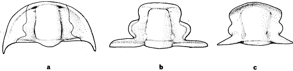
TEXT-FIG. 17. Leiosteigiacea and possible relatives. a , cranidium of Leiostegium , early Ordovician, showing prominent anterior pits at border suggesting conterminant hypostomal attachment, \times 3 ; b , cranidium of late Cambrian Peichiashania (after Shergold 1980, pl. 27, fig. 1), \times 2.5 ; c , early Ordovician Theamataspis (Scutellidae) (after Fortey 1980), \times 5 . If preoccipital muscle impressions in b and c are homologous, this may provide evidence of leiosteigiacean ancestry of Illaenacea via tsinaniids (see text).
