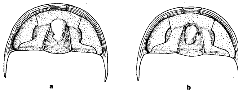
TEXT-FIG. 2. Natant hypostome in life position ( a ), and as it falls down into the glabella on death in those trilobites which died on their backs ( b ) illustrated by generalized ptychoparioid. Compare with Plate 1. Note how glabellar furrows occupy area to each side of the hypostome.
