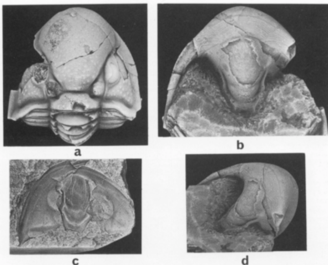
TEXT-FIG. 5. Secondarily attached hypostomes in Proetida. a, b, d , independent hypostomal condition in Griffithides acanthiceps Woodward; Dinantian, Treak Cliff, Castleton, Derbyshire: a , dorsal, and b , ventral views, \times 6 ; d , oblique ventral view, \times 5 . Note anterior pits in axial furrows well posterior to usual position in natant forms. National Museum of Wales (NMW) 86.25G.2332. c , Secondary conterminant hypostomal condition in Archegone (Phillibole) aff. aprathensis Richter and Richter, Dinantian, slopes of Pendle Hill, Lancashire. \times 3 , NMW 88.36G.10. Photographs kindly supplied by R. M. Owens.
