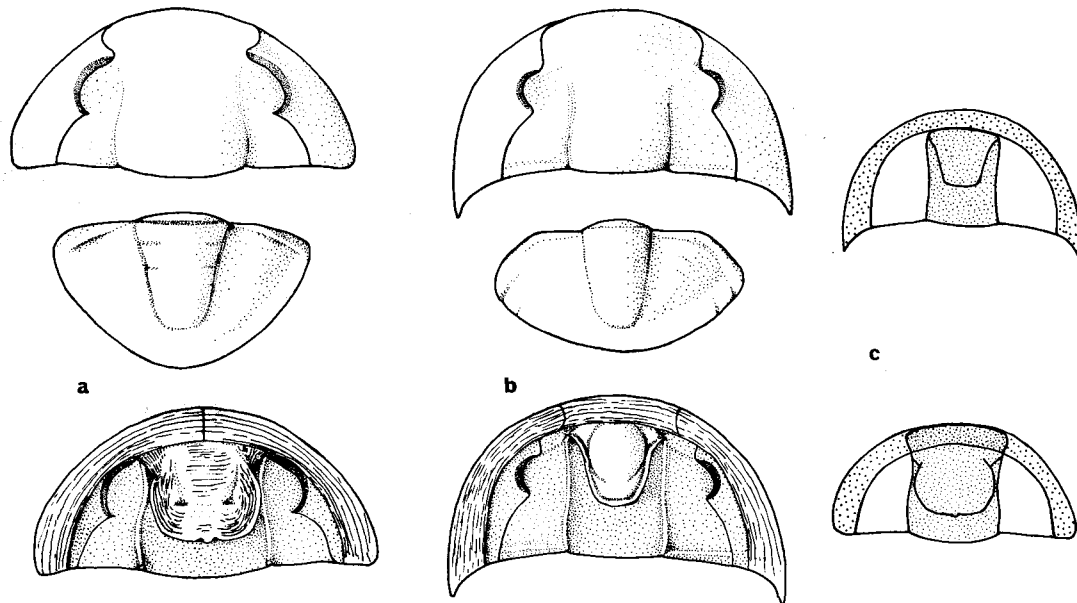
TEXT-FIG. 7. Hypostomal attachment condition as a key to revealing homoeomorphy. a and b , dorsal cephalic and pygidial morphology of the early Ordovician genus Platypeltoides , and the early Cambrian genus Giordanella (after Rasetti 1972) showing general similarity, c . \times 3 . Below, inferred ventral views of the same. c , cartoons illustrating hypostomal attachment mode using same conventions as in text-figure 1, Giordanella above, probably conterminant, Platypeltoides below, impendent.
