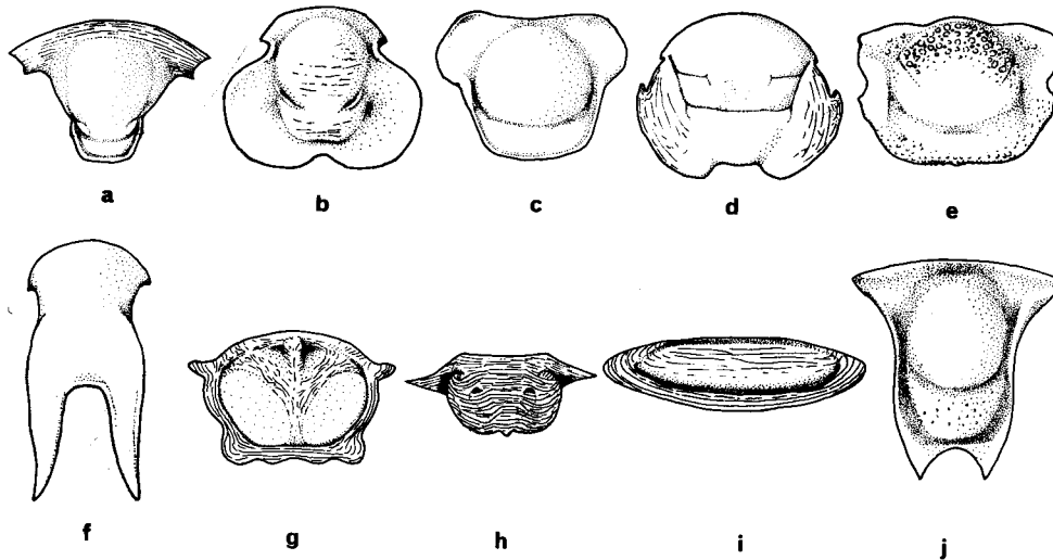
TEXT-FIG. 12. Hypostomes of trilobites in which the hypostome was attached to the doublure in either independent or conterminant mode, showing various kinds of specialization, in contrast to the natant hypostomes shown in text-fig. 11. a-e shows primary conterminant examples, as interpreted herein; f-i are secondarily conterminant hypostomes belonging to Libristoma; j may be secondarily conterminant (see discussion of Phacopida, p. 565). a , Fieldaspis (Corynexochida), Middle Cambrian (after Rasetti 1951, pl. 16, fig. 17), \times 1.5 ; b , Palaeadotes (Damesallacea), Cambrian, Mindyallan (after Öpik 1967, pl. 50, fig. 3), \times 4 ; c , illaenid (Illaenacea), Middle Ordovician (after Whittington 1963, pl. 18, fig. 4), \times 3 ; d , Amphilichas (Lichida), Middle Ordovician (after Tripp and Evitt 1981, pl. 2, fig. 28), \times 6 ; e , Primaspis (Odontopleurida), Silurian (after Chatterton and Perry 1983, pl. 5, fig. 5), \times 6 ; f , Lycophron (Asaphacea), early Ordovician (after Fortey and Shergold 1984, pl. 43, fig. 5), \times 3 ; g , Remopleurides (Remopleuridacea), Middle Ordovician (after Whittington 1959, pl. 17, fig. 18), \times 6 ; h , Symphysurus (Cyclopygacea), Middle Ordovician (after Fortey 1986, fig. 2), \times 1 ; i , Degamella (Cyclopygacea), early Ordovician (after Fortey and Owens 1987, fig. 38 d ), \times 2.5 ; j , Salterocoryphe (Calymenacea), Middle Ordovician (after Hammann 1983, pl. 11, fig. 107), \times 6 .
