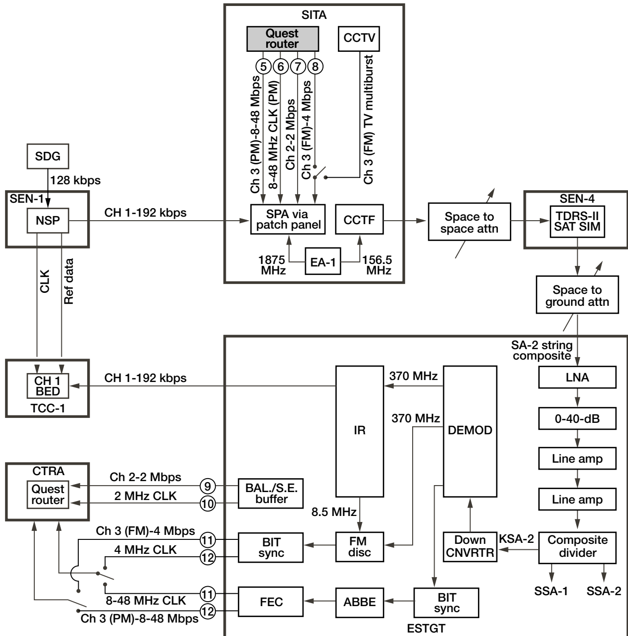
Figure 3.—Return link.
