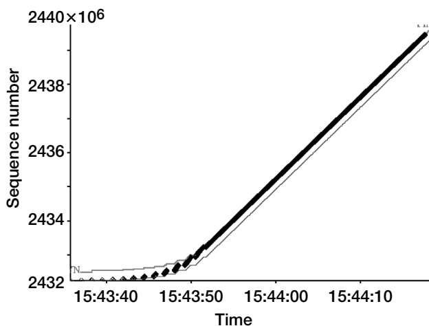
Figure 14.—Tuned TCP/BER = 0.
