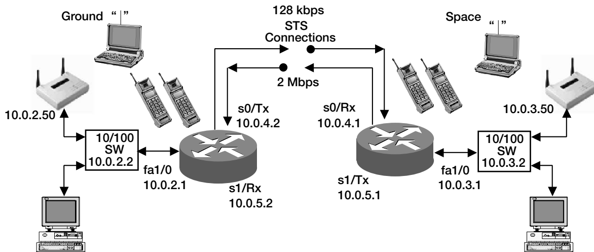
Figure 16.—Network topology supports multicast.
