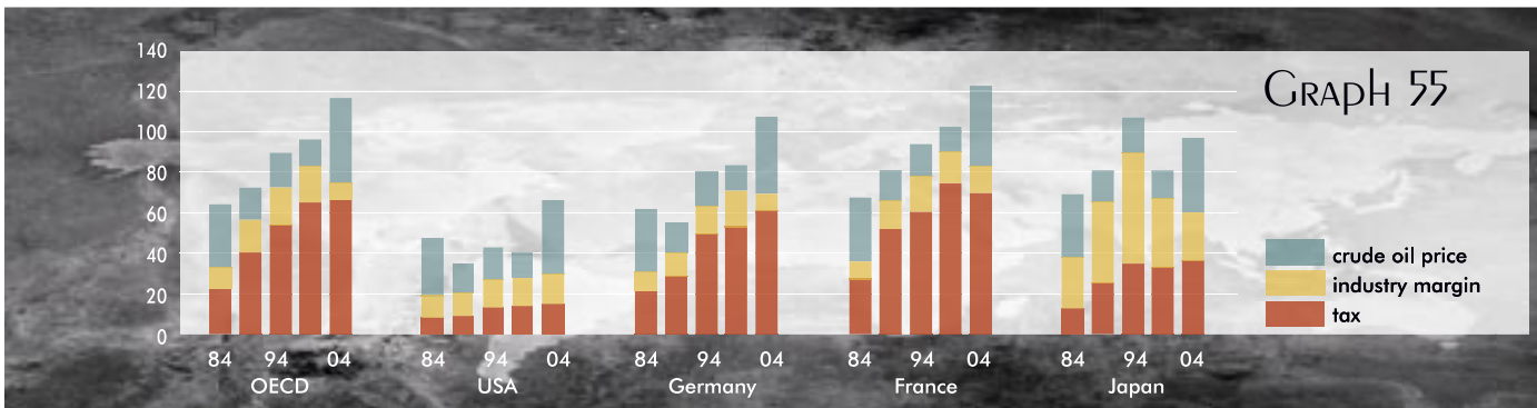
Composite barrel and its components, 1984–2004 ($/b)
