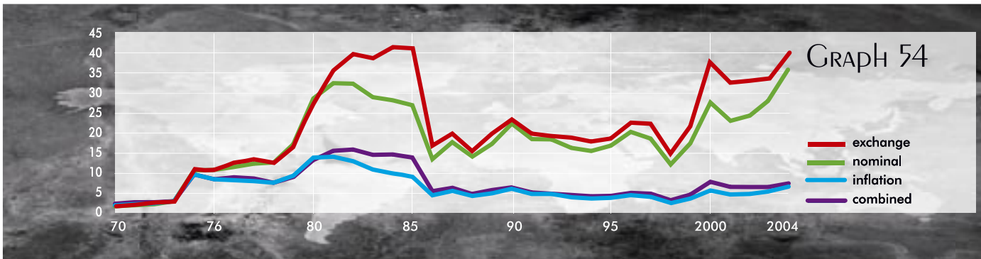
Crude oil prices in nominal and real terms, 1970–2004 ($/b) 1973=100
