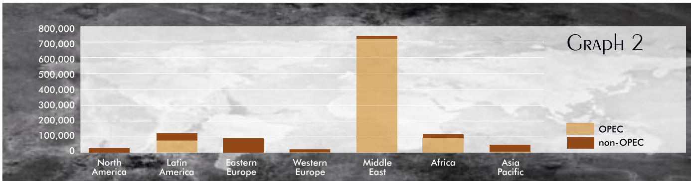
Crude oil reserves by region, 2004 (m b)
