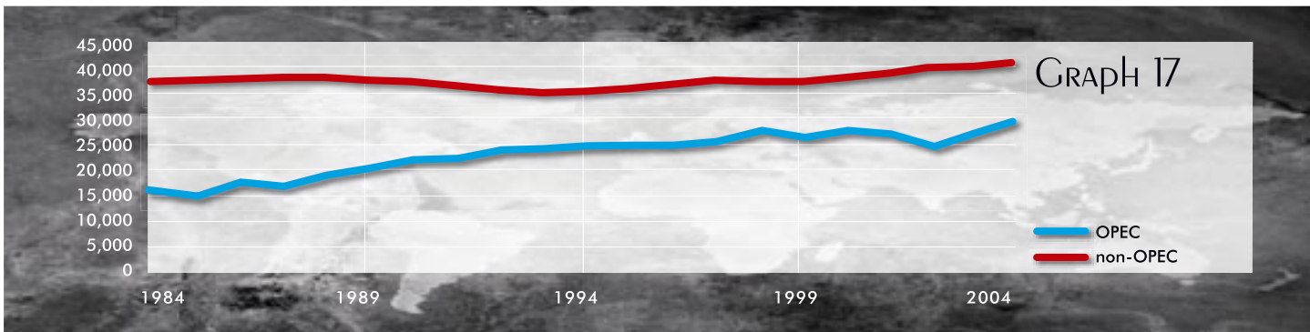
World crude oil production, 1984–2004 (1,000 b/d)
