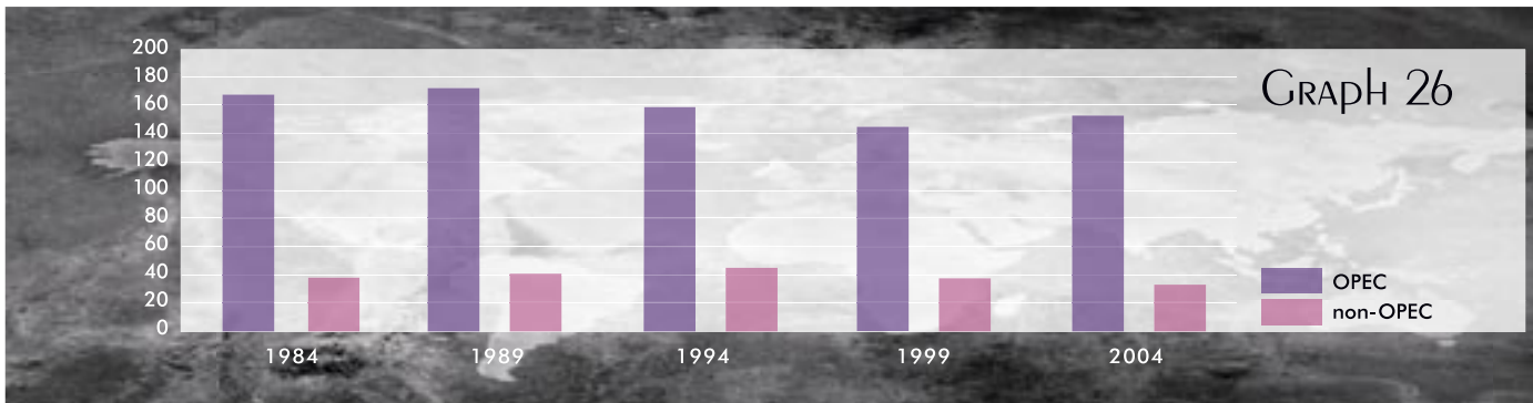
World natural gas reserves to production ratios (gross production minus re-injection) (years)
