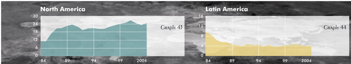
Percentage of OPEC exports to regions (m b/d)
