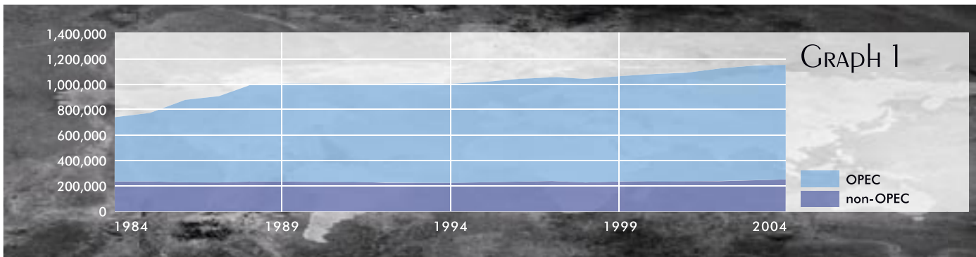
World proven crude oil reserves, 1984–2004 (m b)
