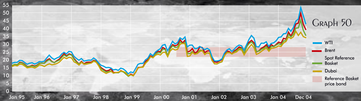
OPEC Reference Basket and other spot crude oil prices, 1995-04 ($/b)
