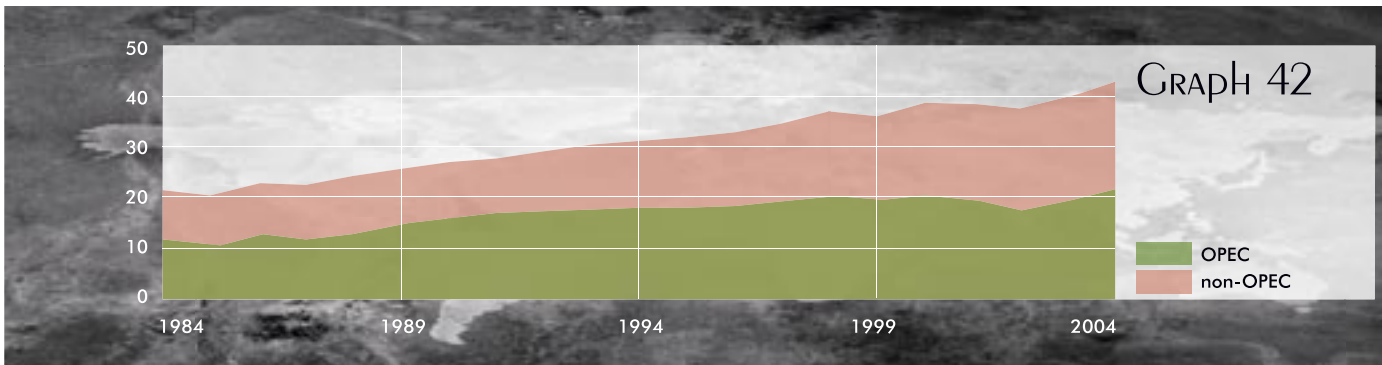
Crude oil exports, 1984–2004 (m b/d)
