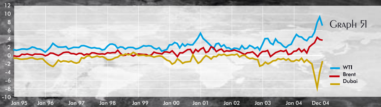
Spot price differences of WTI, Brent and Dubai to OPEC Basket, 1995-04 ($/b)
