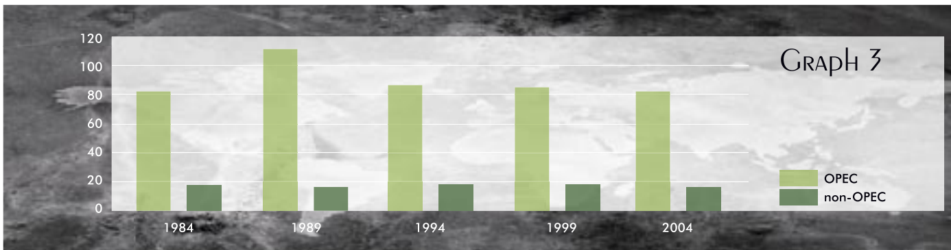
Crude oil reserves to production ratios, 1984–2004 (years)
