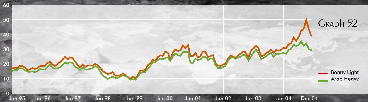
Spot prices of Bonny Light and Arab Heavy, 1995-04 ($/b)
