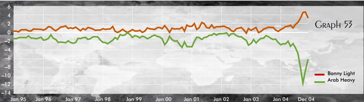
Spot price differences of Bonny Light and Arab Heavy to OPEC Basket, 1995-04 ($/b)
