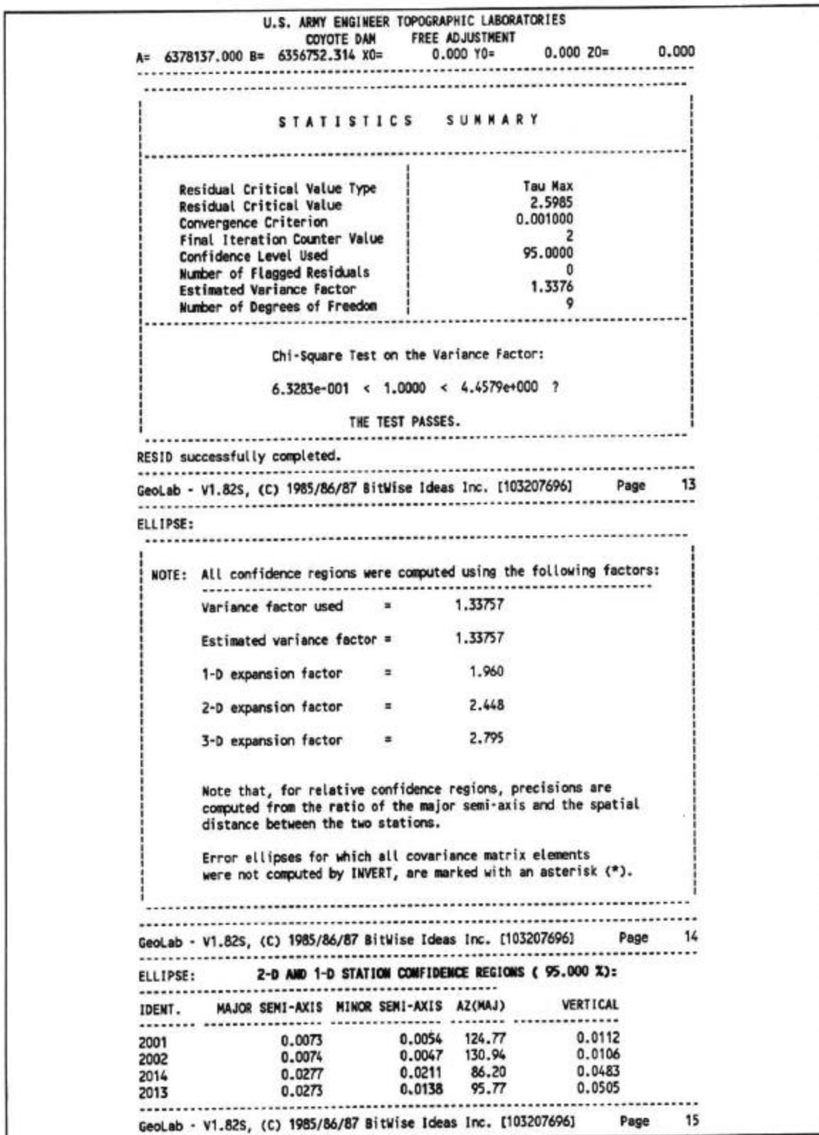
Figure F-11f. GEOLAB Adjustment Output (Free)
