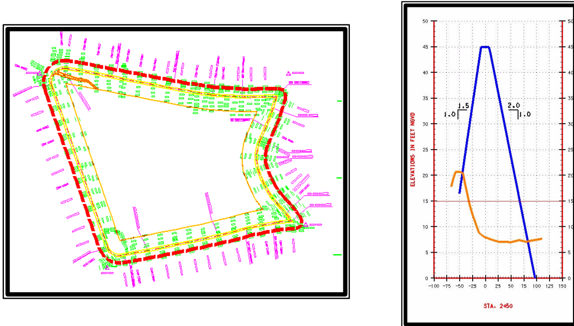
Figure D-1. Plan of confined disposal area and typical section
