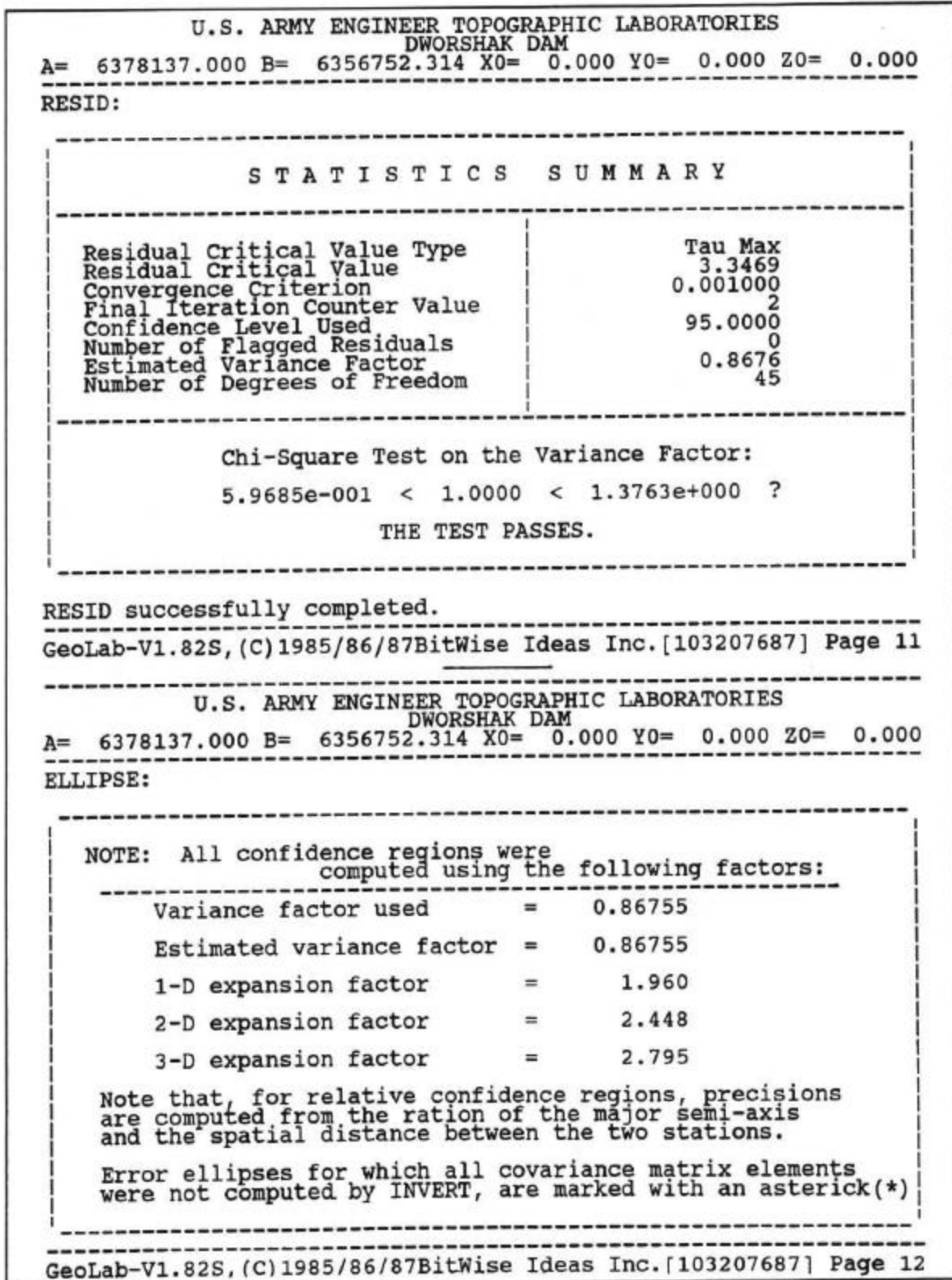
Figure G-3g. GEOLAB adjustment output (Dworshak Dam Reference Network)
