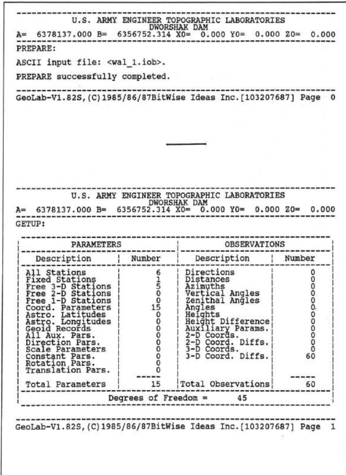
Figure G-3a. GEOLAB adjustment output (Dworshak Dam Reference Network)
