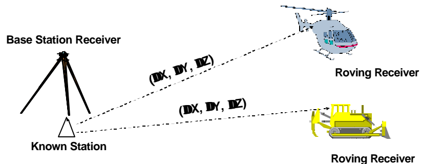
Figure 9-14. Kinematic survey techniques
