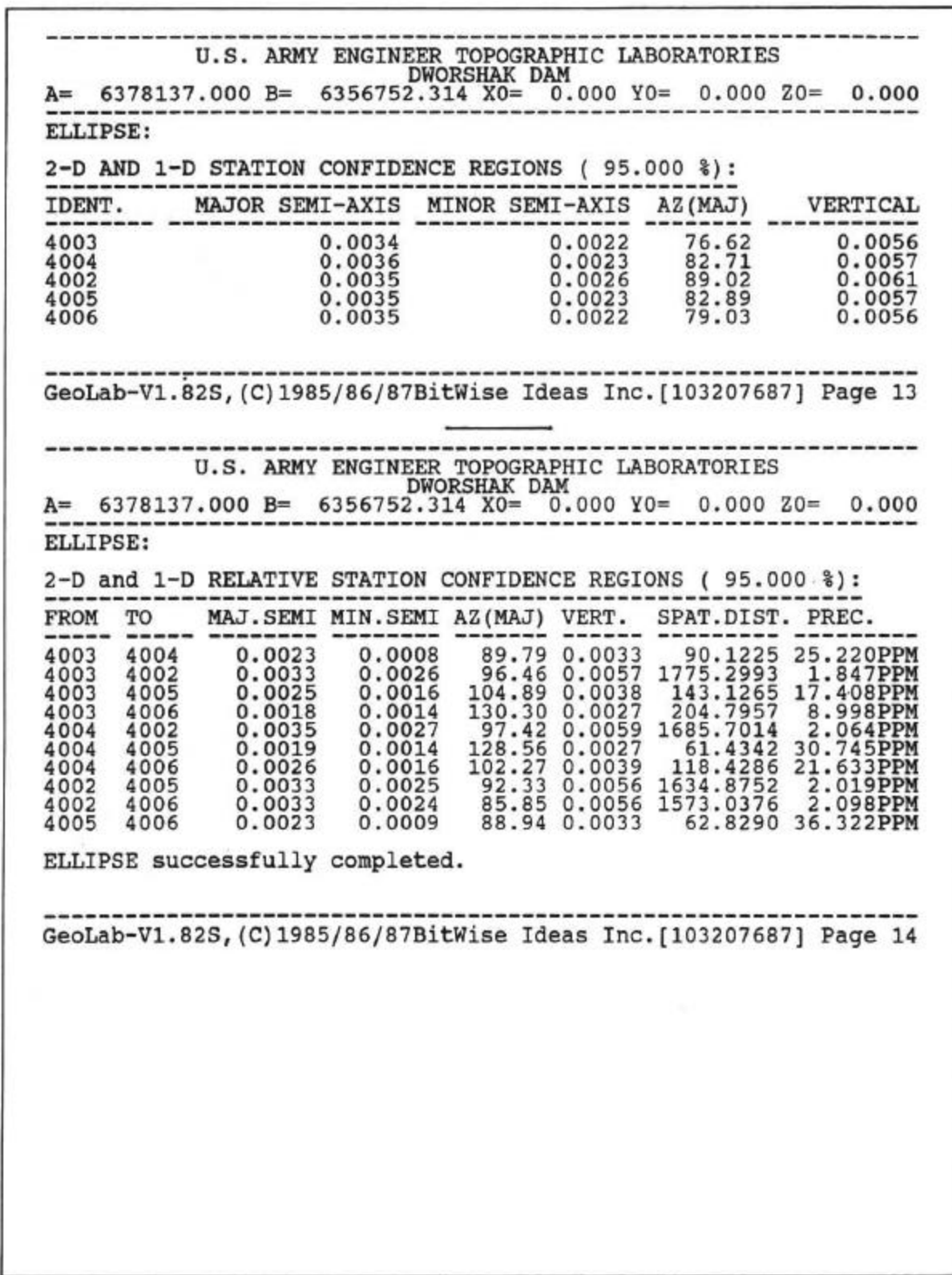
Figure G-3h. GEOLAB adjustment output (Dworshak Dam Reference Network)
