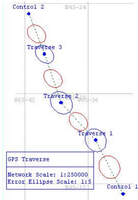
Figure 11-6. Relative accuracy ellipses for points (blue) and baselines (red). Control 1 and Control 2 are fixed points. (Microsearch GeoLab 2001 Adjustment Software)
