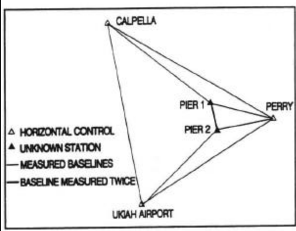
Figure F-2. GPS Project Diagram (Ukiah)
