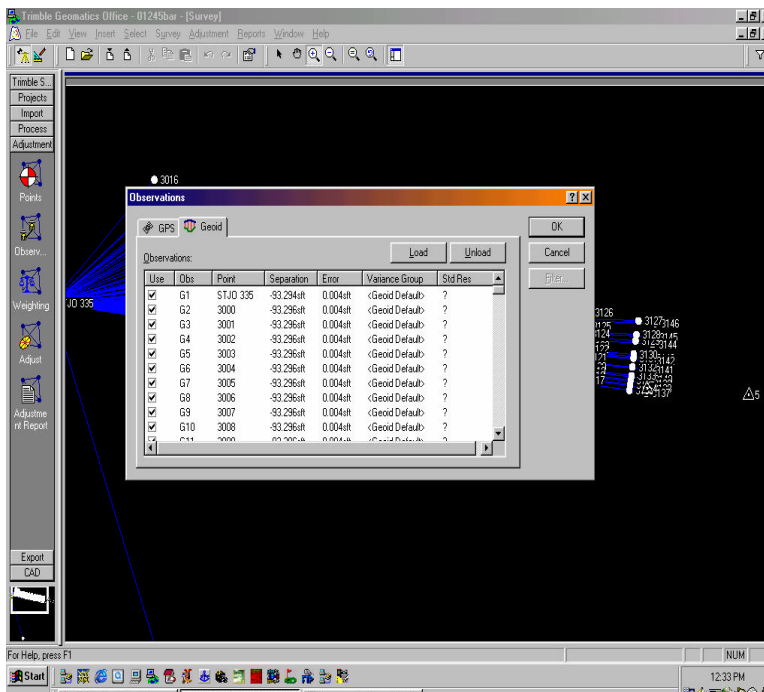
Figure D-6. Trimble Geomatics Observations windows
