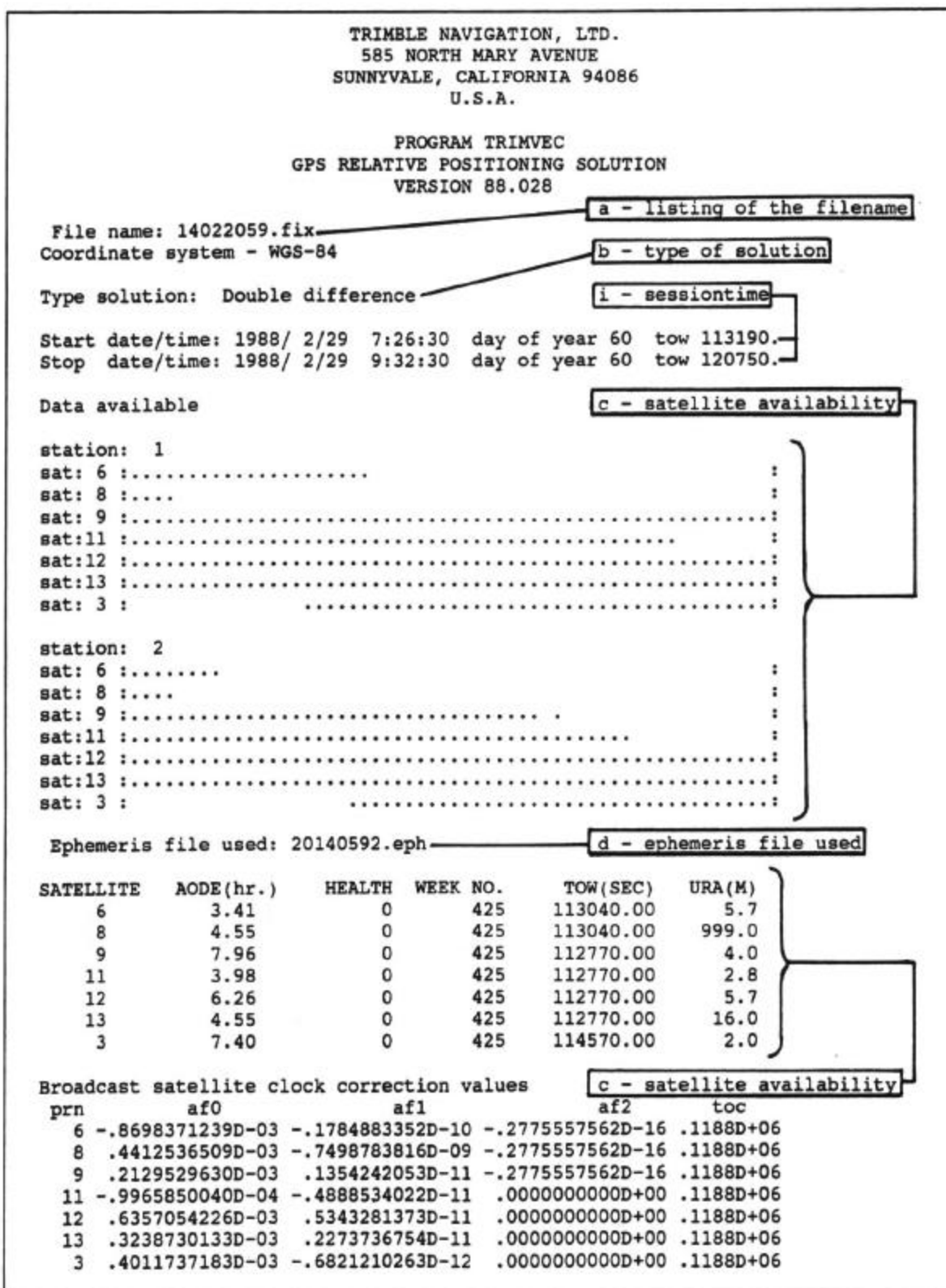
Figure F-8a. TRIMBLE Baseline Solution File (Ukiah Baseline 2014--2002)
