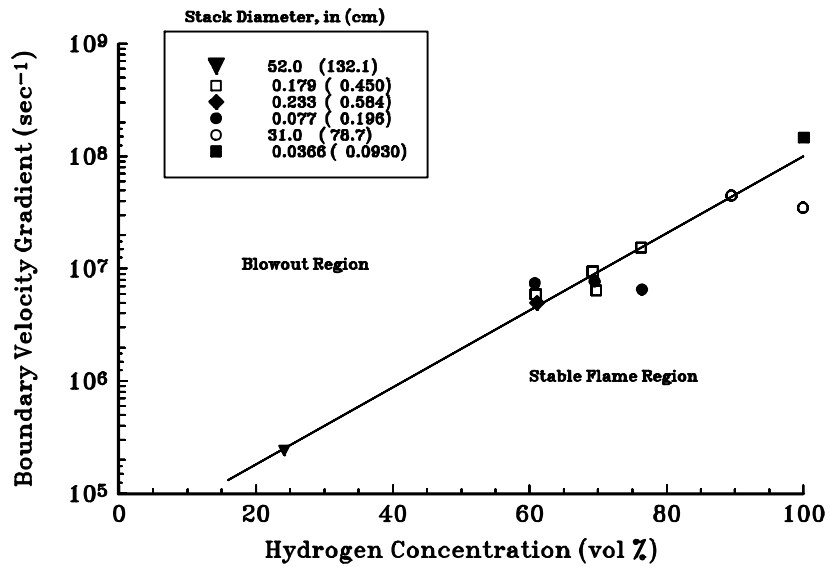
Figure A4.2 Blowout and Stable Flame Region
