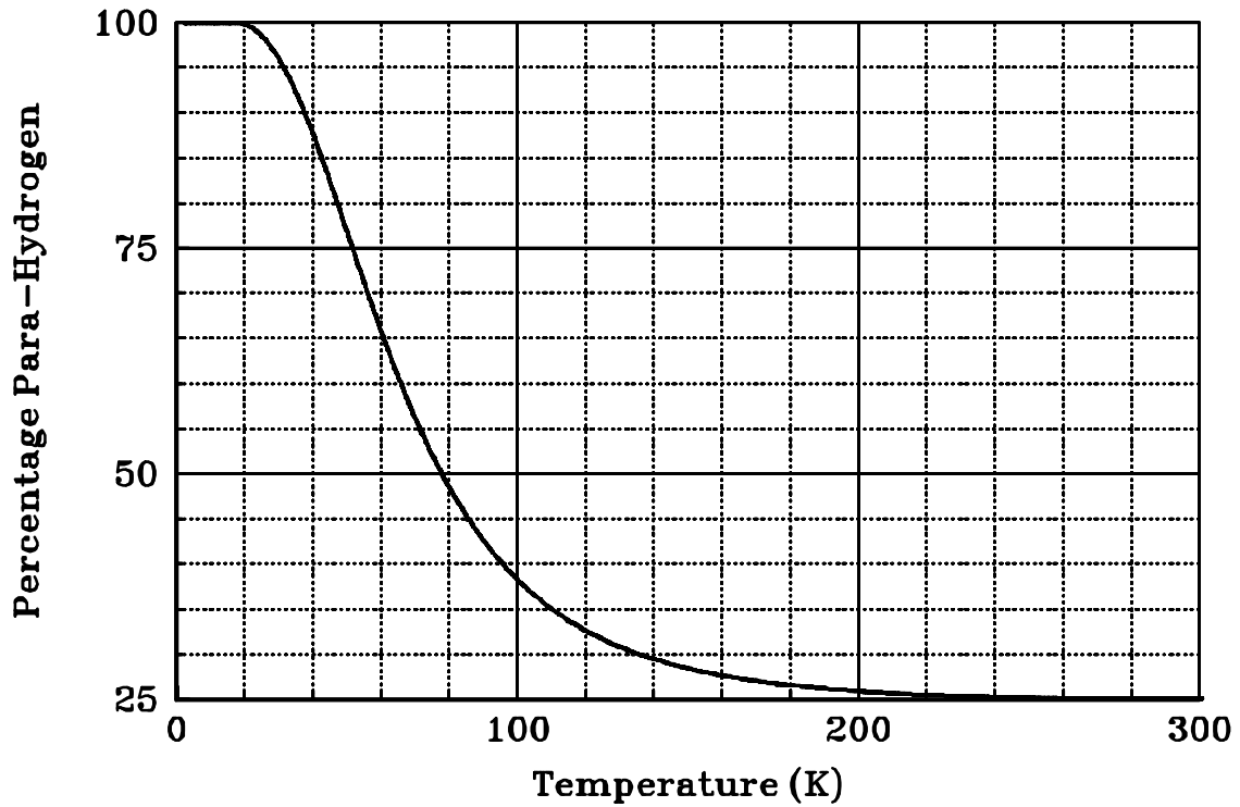
Figure A1.1 Equilibrium Percentage of Para-hydrogen vs. Temperature
