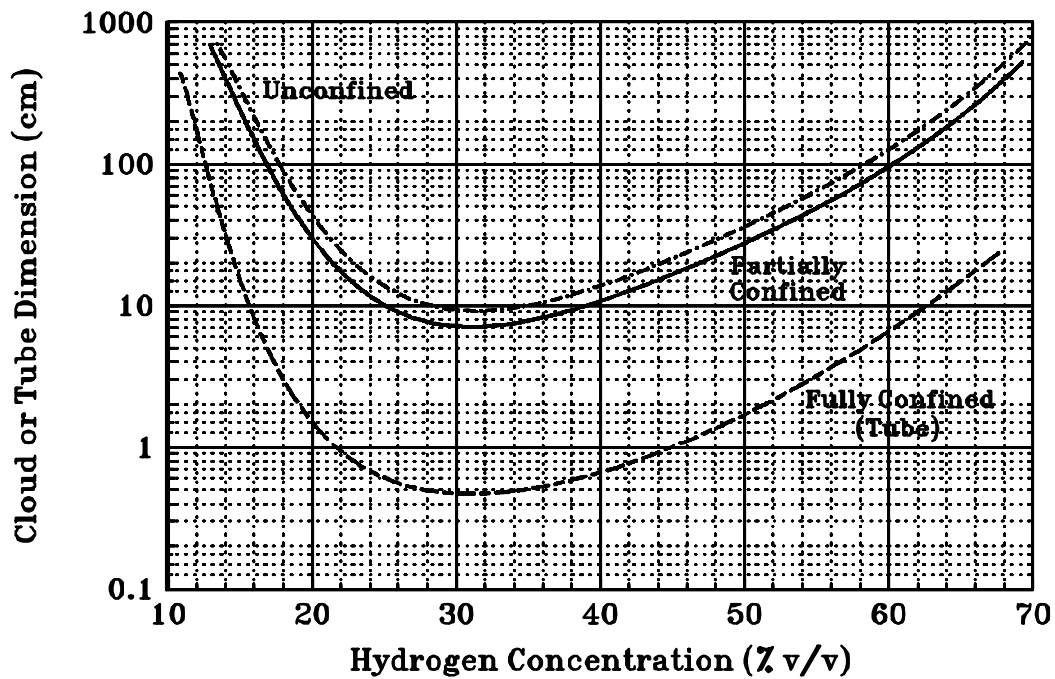
Figure A2.7 Minimum Dimensions of \text{H}_2 -Air Mixtures for Detonation at 101.3 kPa (14.7 psia) and 298 K (77 °F)
