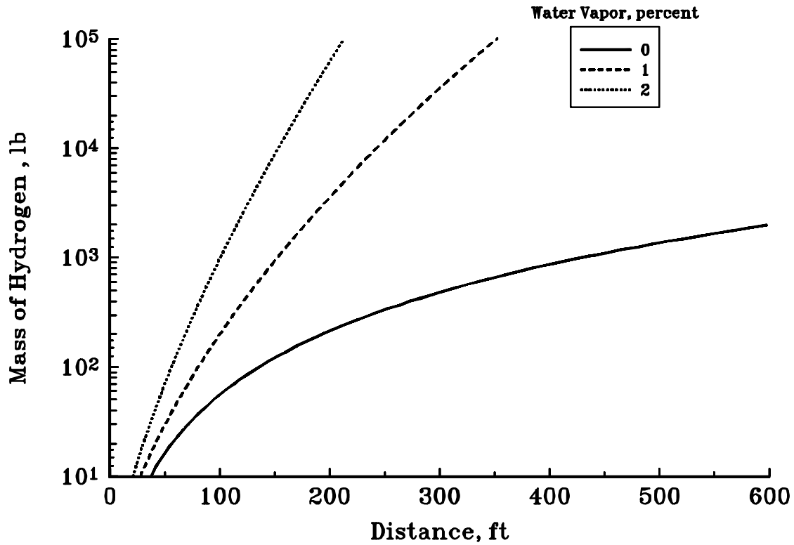
Figure A2.6 Variation in Distance from a Hydrogen Fire for a Thermal Radiation Exposure of 2 \text{ cal/cm}^2 for an Exposure Duration of 10 s
