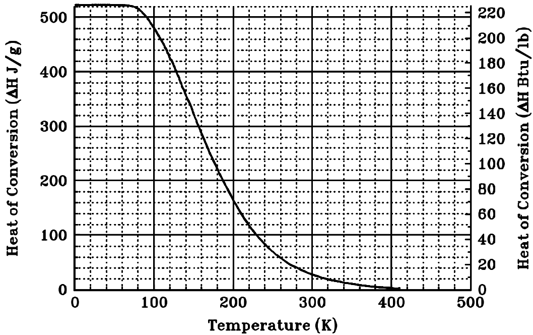
Figure A1.2 Enthalpy of Normal Hydrogen Conversion
