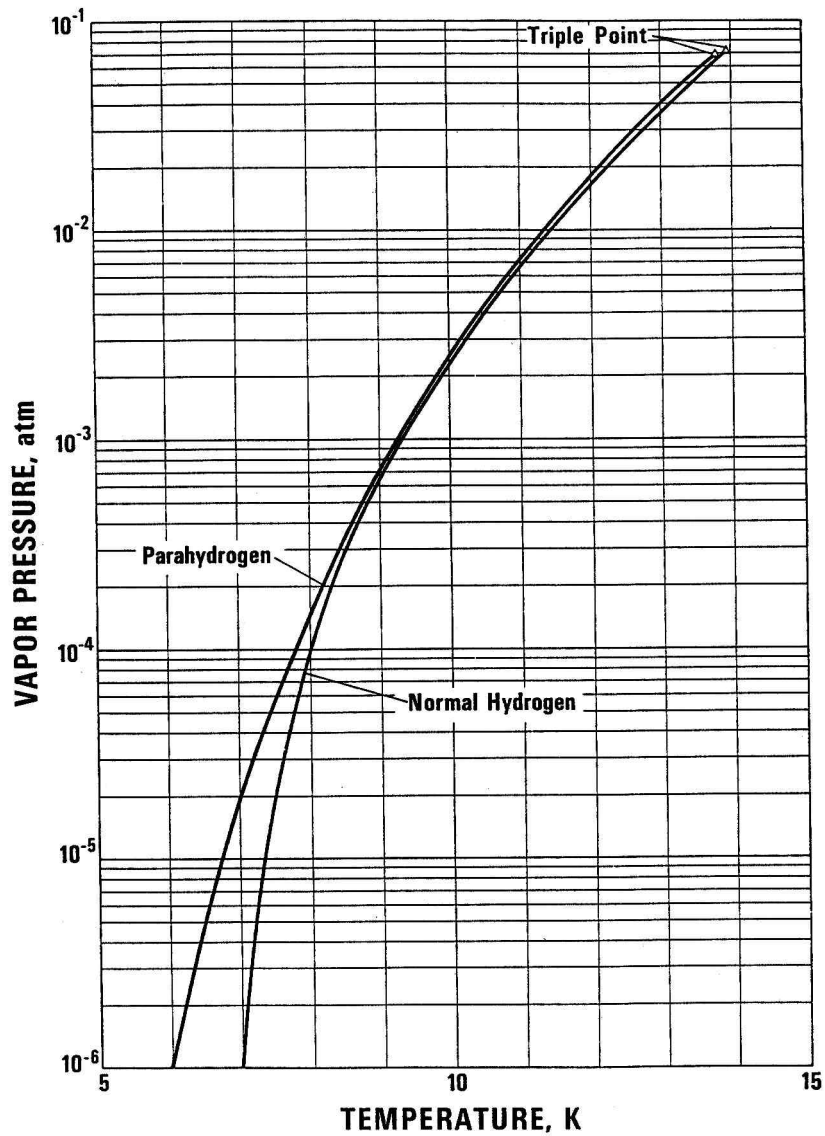
Figure A1.5 Vapor Pressures of Normal and Para-hydrogen Below the Triple Point
