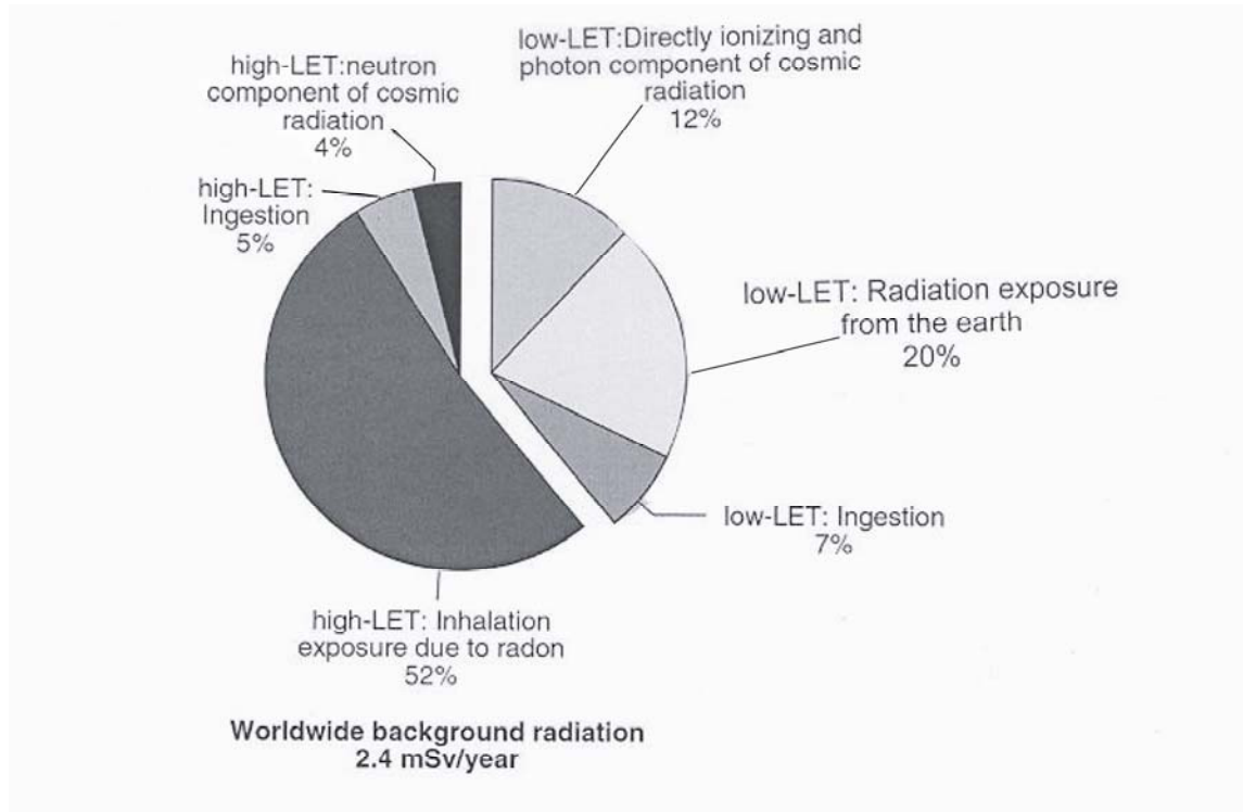
FIGURE PS-1. Sources of global "background" radiation. The pie chart above shows the relative world-wide percentage of all sources of natural "background" radiation (low- and high-LET). Because the BEIR VII report evaluates the health effects of low-LET radiation, we have separated the low-LET portion of the pie chart to illustrate the relative contributions of the three major sources of low-LET radiation exposure.
