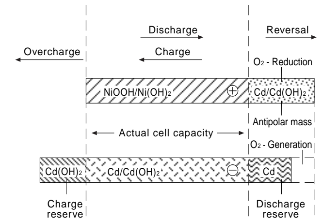
Balance of electrode capacities (cell balance) in a sealed nickel/cadmium battery with reversal protection by 'antipolar material'
