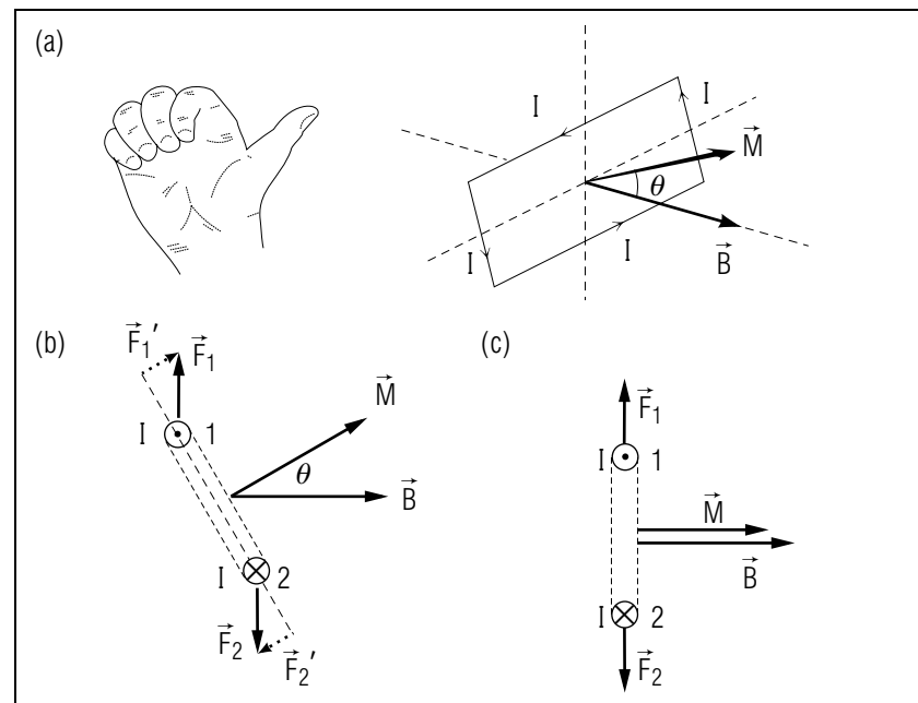
Fig. F-1: Current loop in a uniform magnetic field \vec{B} . (a) Three-dimensional view of the loop and comparison with a right hand specifying the direction of the magnetic moment \vec{M} . (b), (c) End-on views of the loop in two different orientations relative to \vec{B} .
