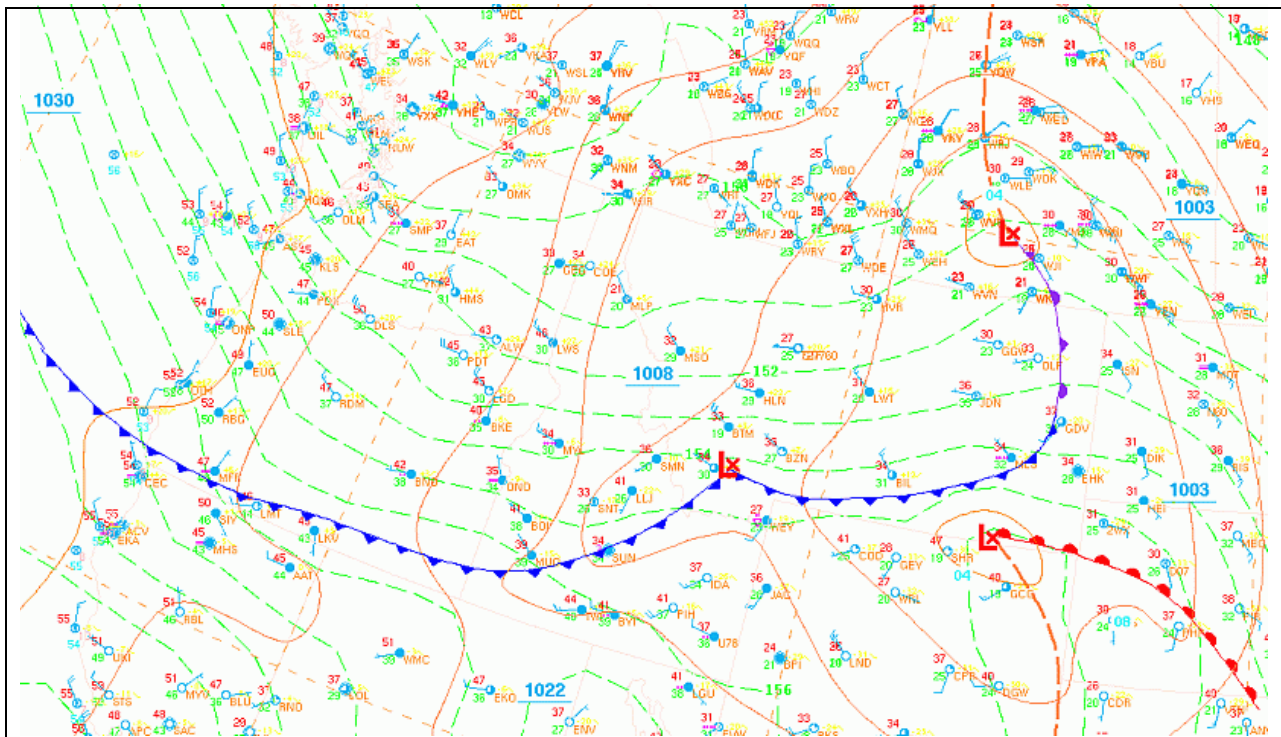
Figure 13. An example of 850-700 hPa thickness levels in the Northwest with surface observations included. Even in this textbook example, note how local winds in certain spots make the placement less than obvious.
