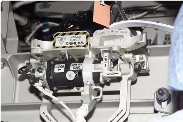
Engineering photo of the IUA with the TUS cable routed through mechanism before launch and installation on ISS.
