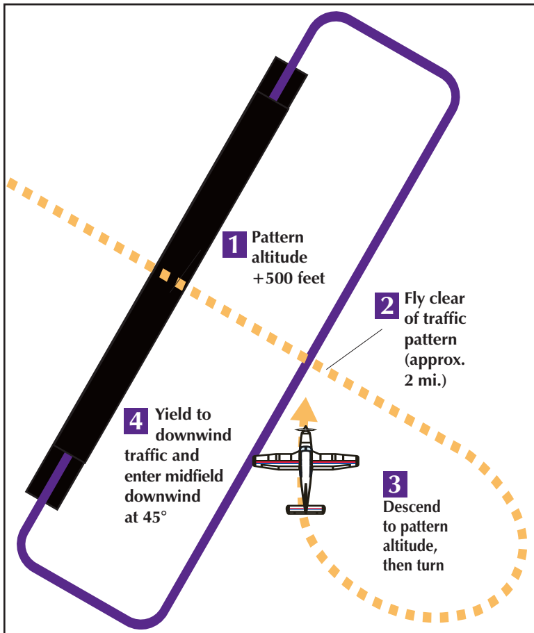
Figure 9. Preferred Entry from Upwind Side of Airport
