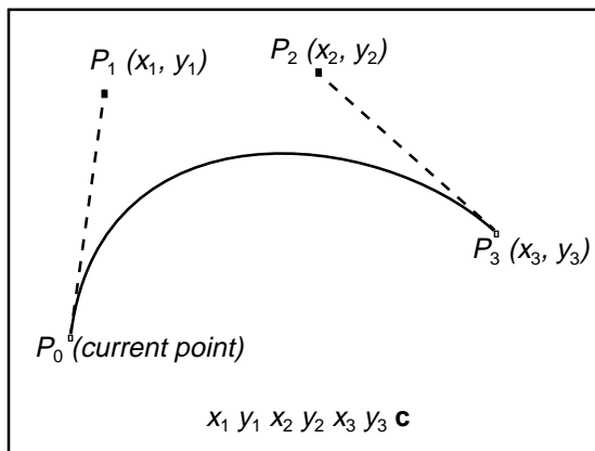
Figure 8.7 Bézier curve
