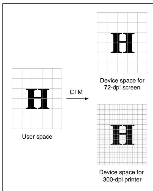
Figure 3.2 User space
