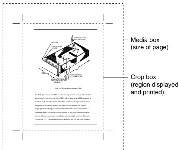
Figure 6.2 Page object's media box and crop box
