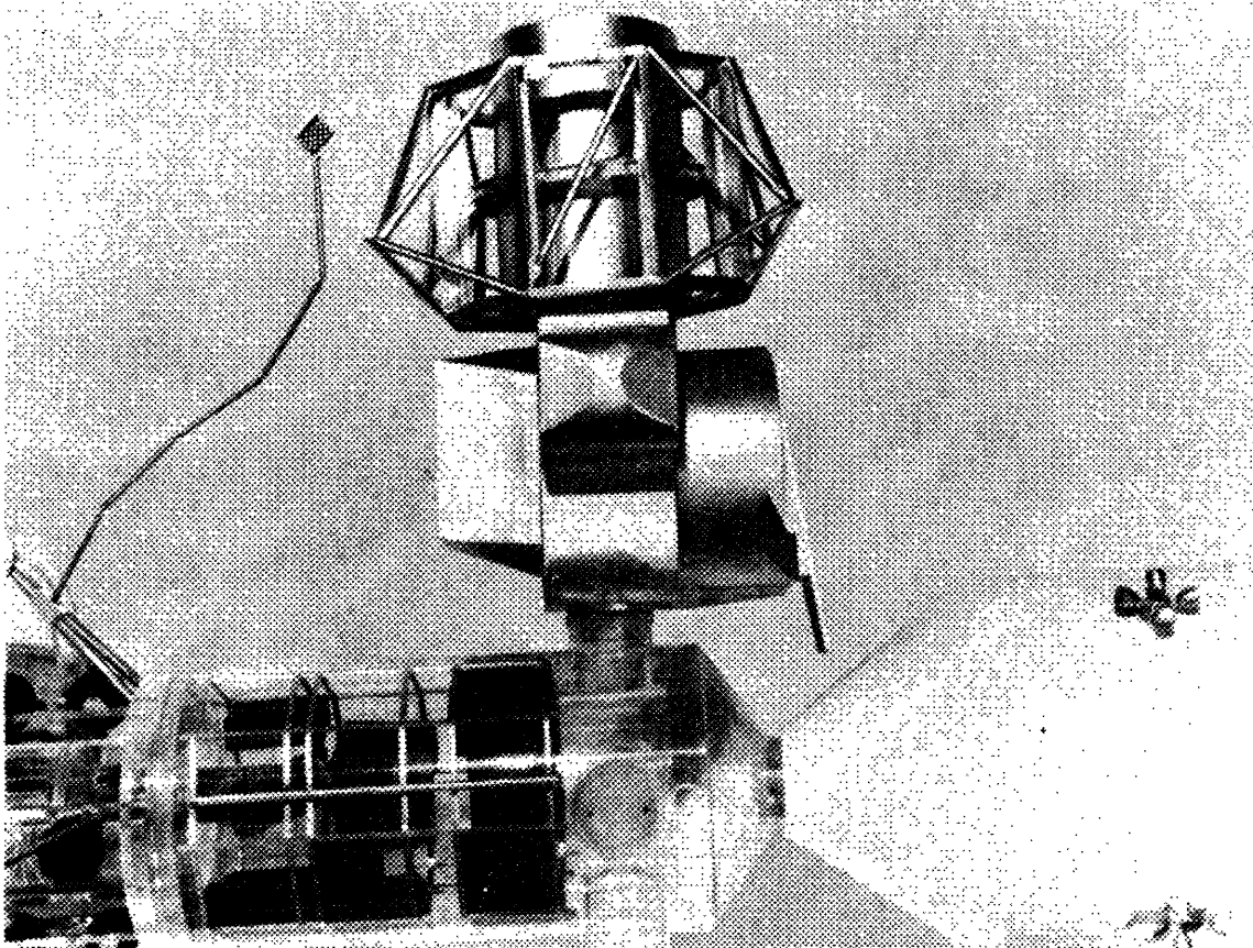
Figure 32. Serpentuator Concept Evaluation Model
