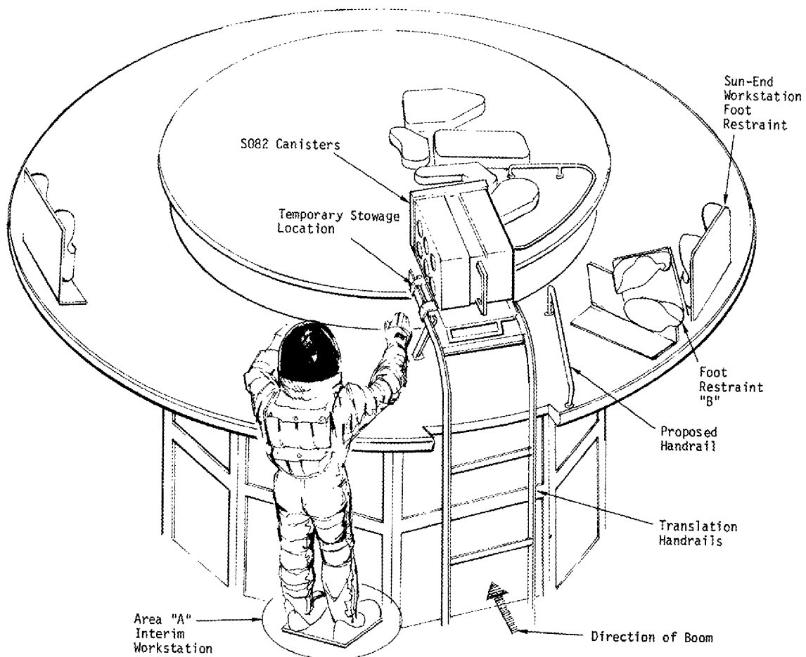
Figure 83. Proposed Sun End Changes for the Extendible Boom Film Transfer Concept
