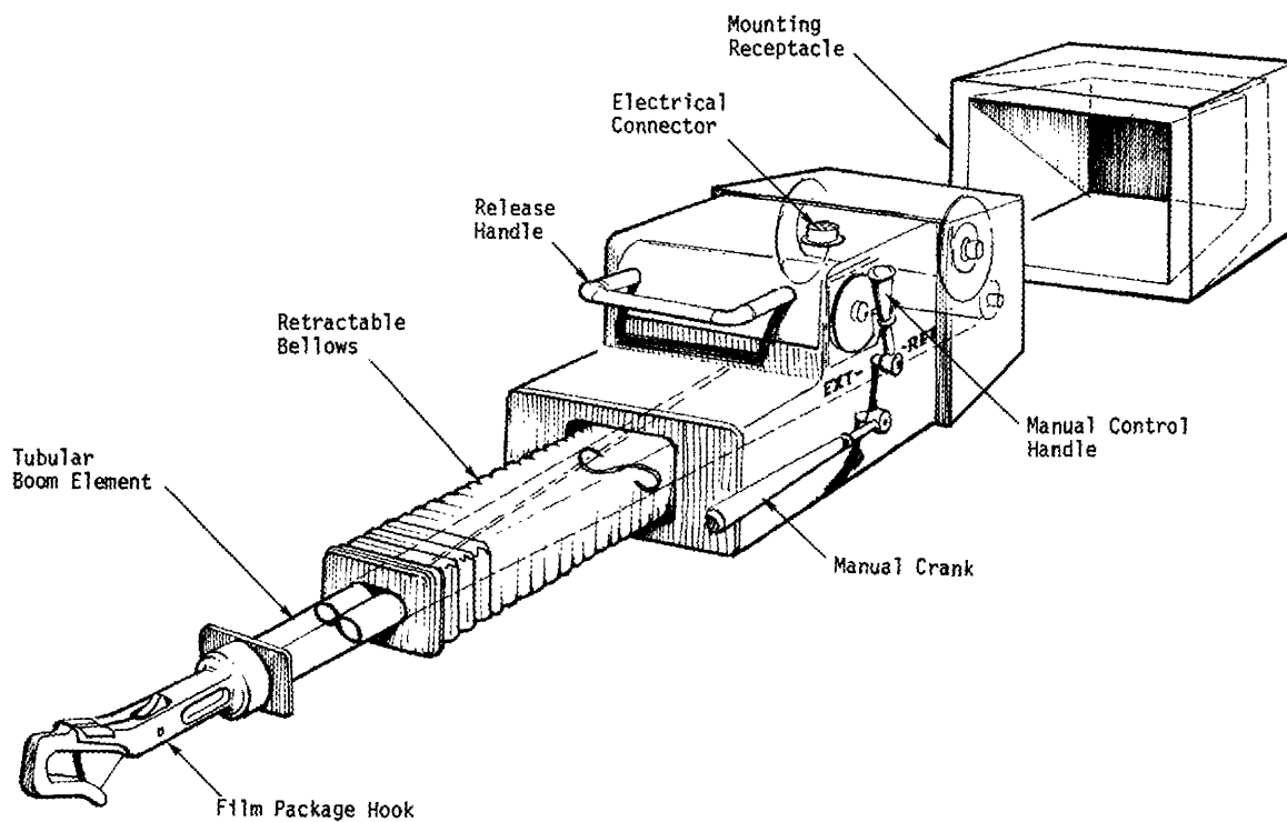
Figure 87. Film Transfer Boom and Hook
