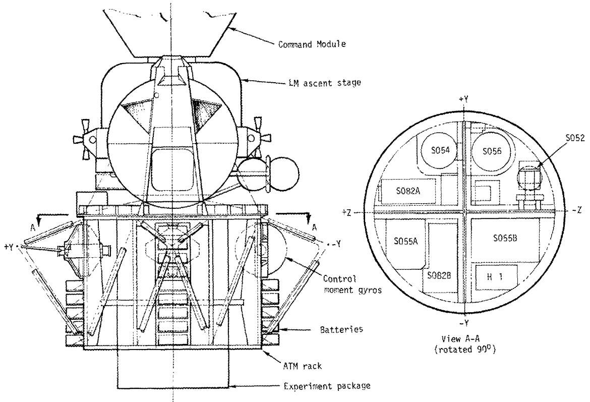
Figure 8. Early LM/ATM Configuration and Experiment Package Arrangement
