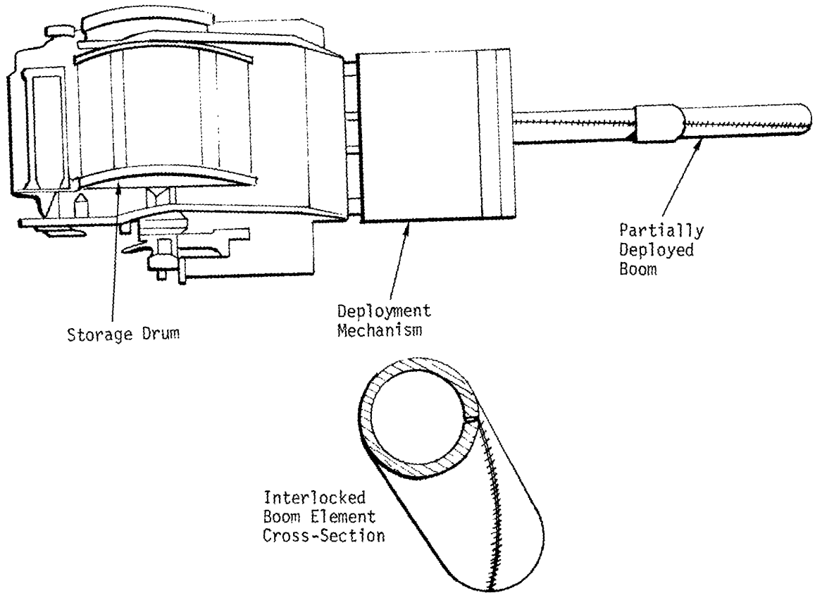
Figure 36. Application Technology Satellite (ATS) Boom Deployer
