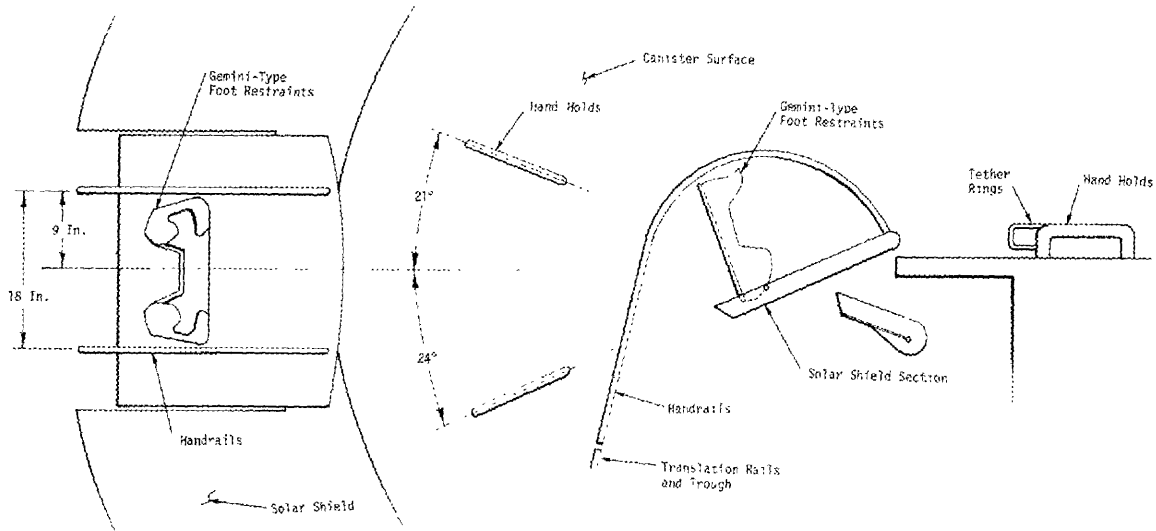
Figure 53. Deployable Sun-End Workstation with Canister Mounted Hand Holds
