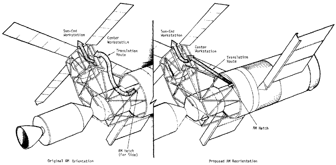
Figure 71. ATM Workstation and AM Hatch Orientation
