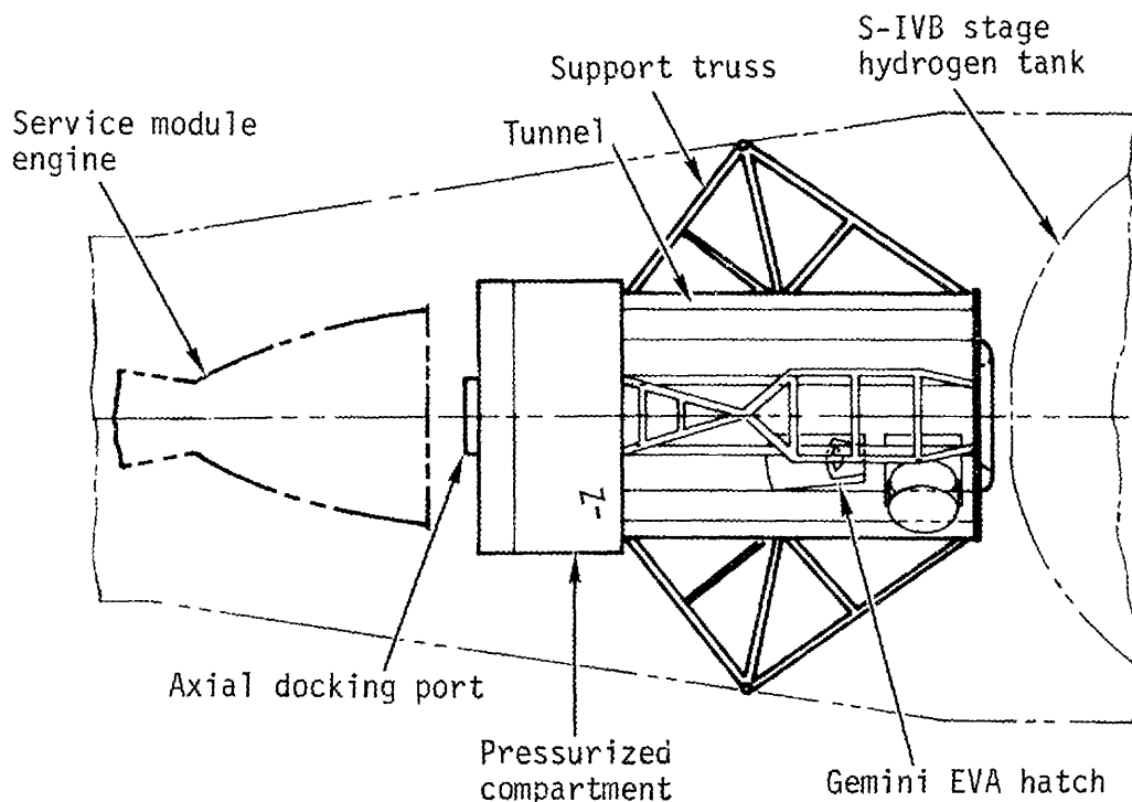
Figure 3. Airlock Module Launch Configuration
