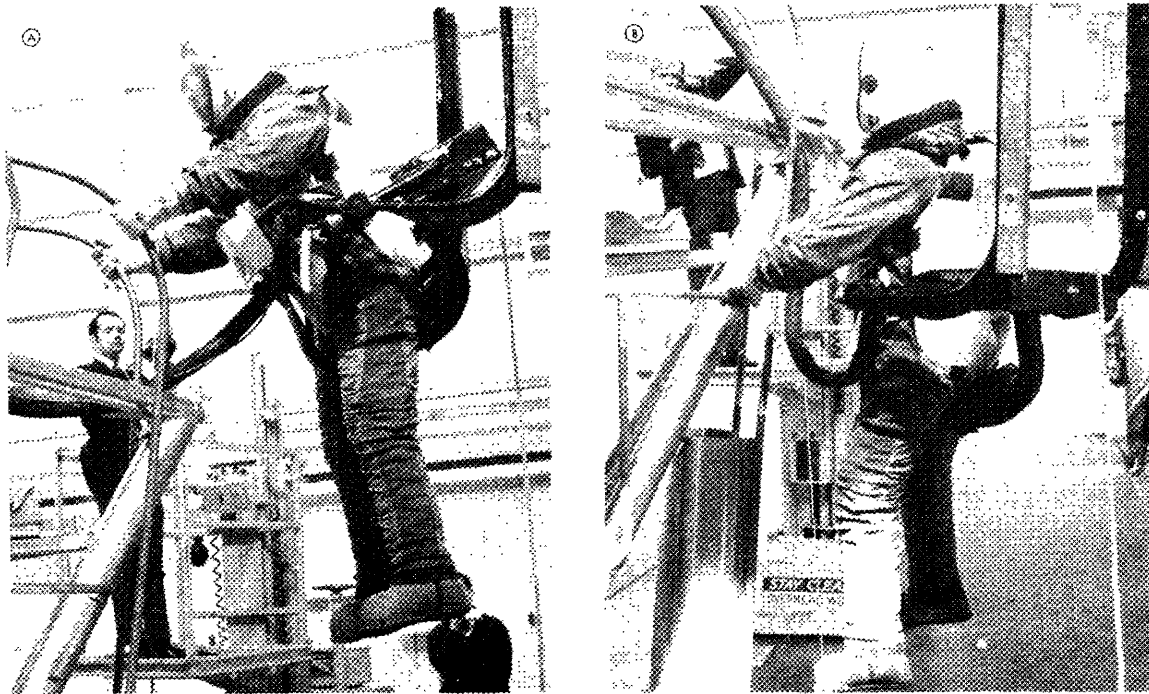
Translating Across Outrigger Truss Lateral Translation to LM End With T-Bar Handrail
