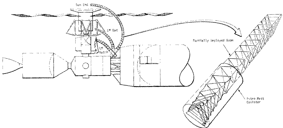
Figure 37. Astro Mast Lattice Boom Deployment Concept
