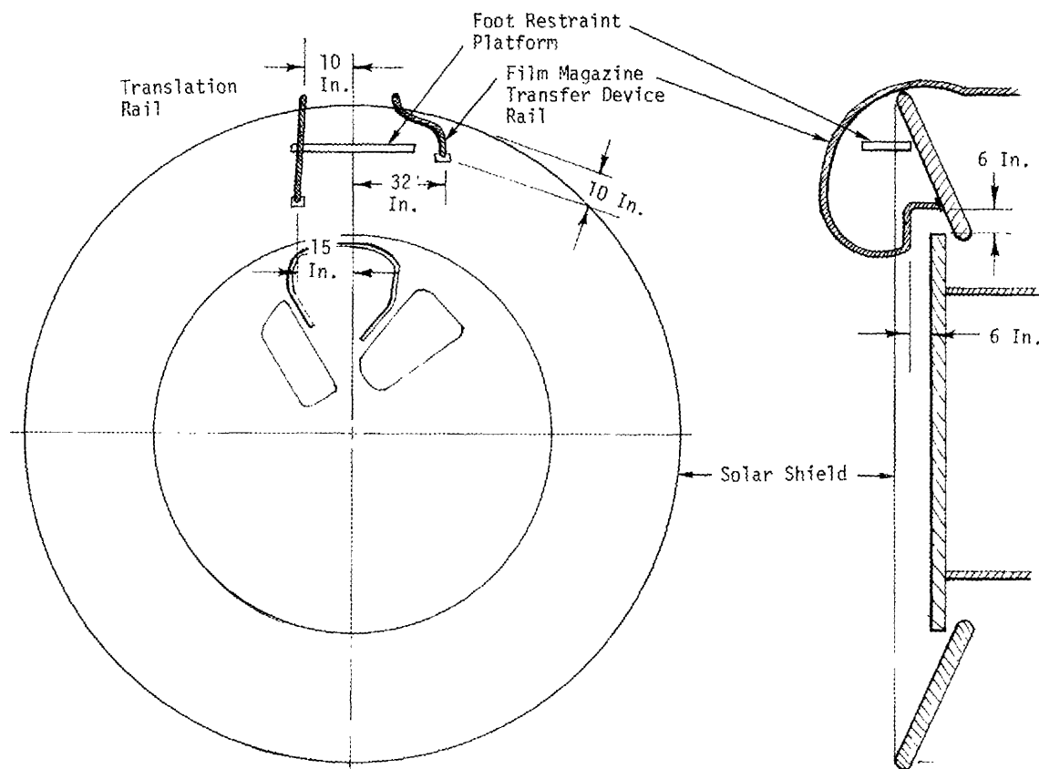
Figure 54. Permanently Mounted Sun-End Workstation
