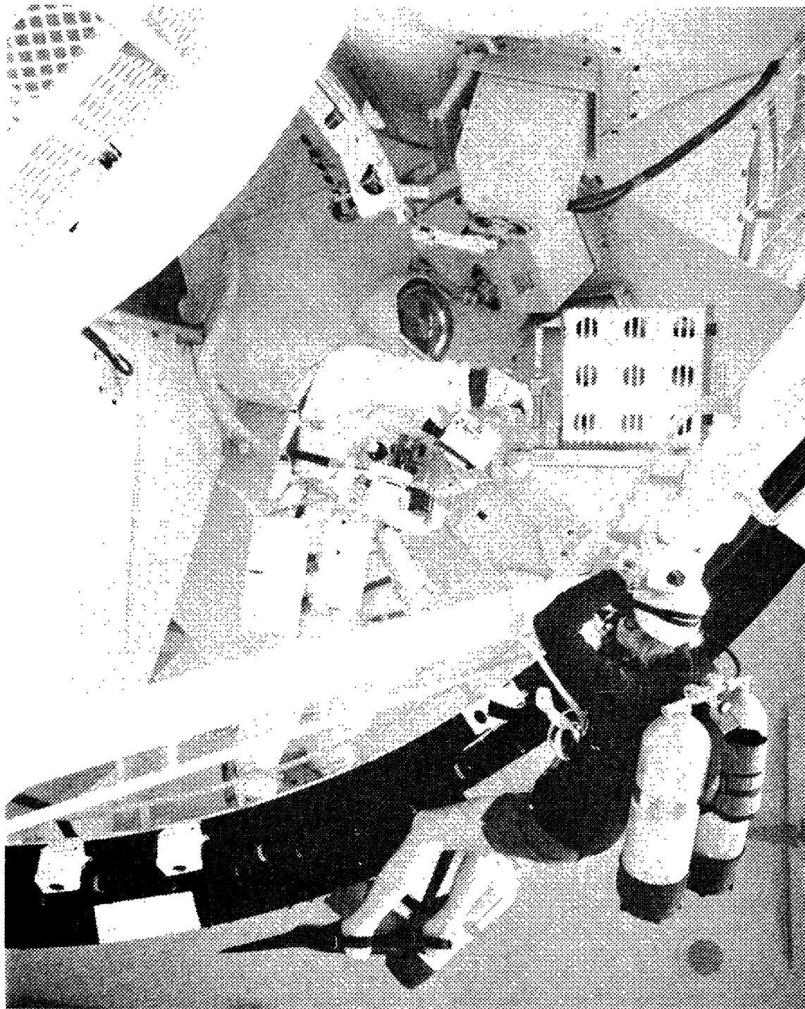
Figure 97. View of FAS workstation with crewman placing 16mm camera, used to photograph the EVA operations, in a stowage position adjacent to the sun-end film tree. The film transfer boom hooks are installed on the booms and folded to the standby position. At the crewman's right are the boom control panel and a temporary magazine stowage hook.
