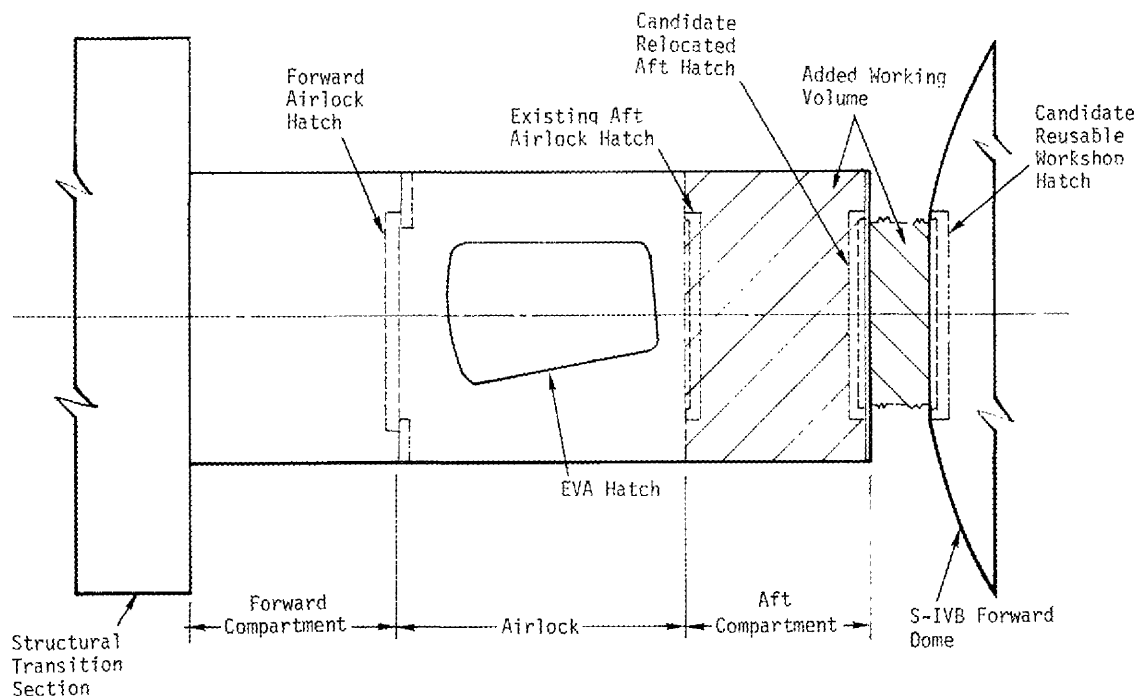
Figure 73. Proposed Methods of Expanding Airlock Working Volume
