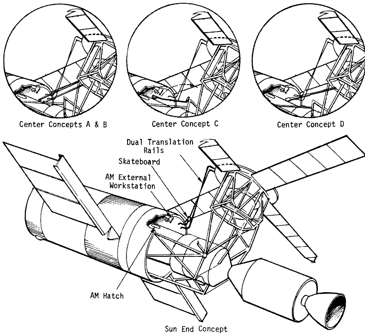
Figure 79. Dry Workshop Film Transfer and Translation Concepts
