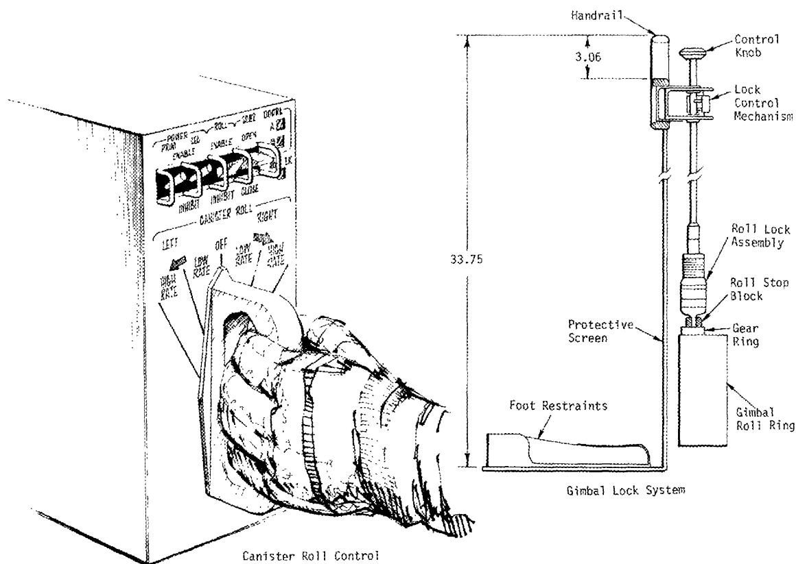
Figure 44. Canister Roll Control Panel and Gimbal Lock System
