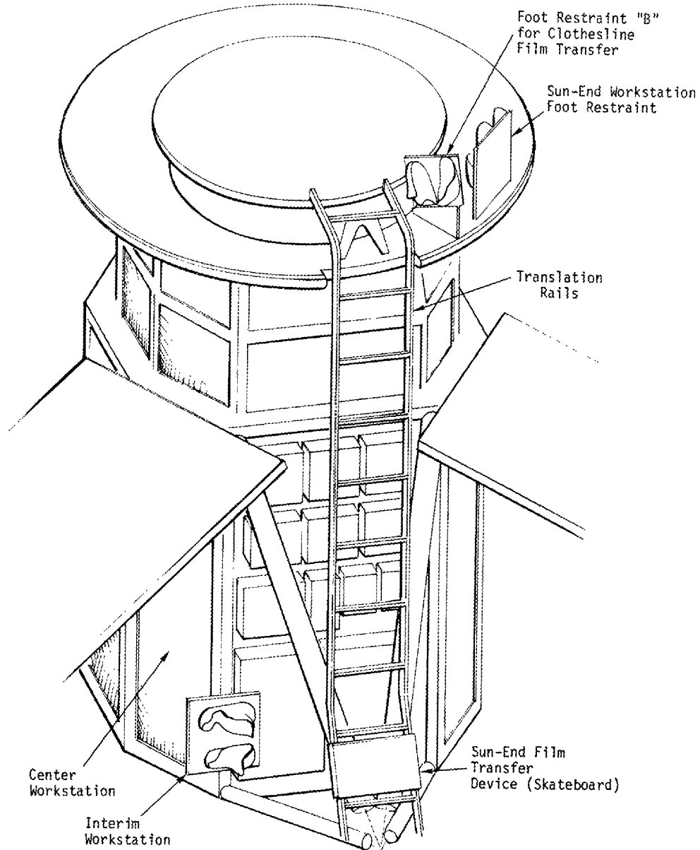
Figure 82. Sun-End Film Transfer Concepts
