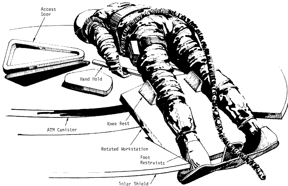
Figure 29. Concept for Sun-End Workstation On Rotating Solar Shield Section
