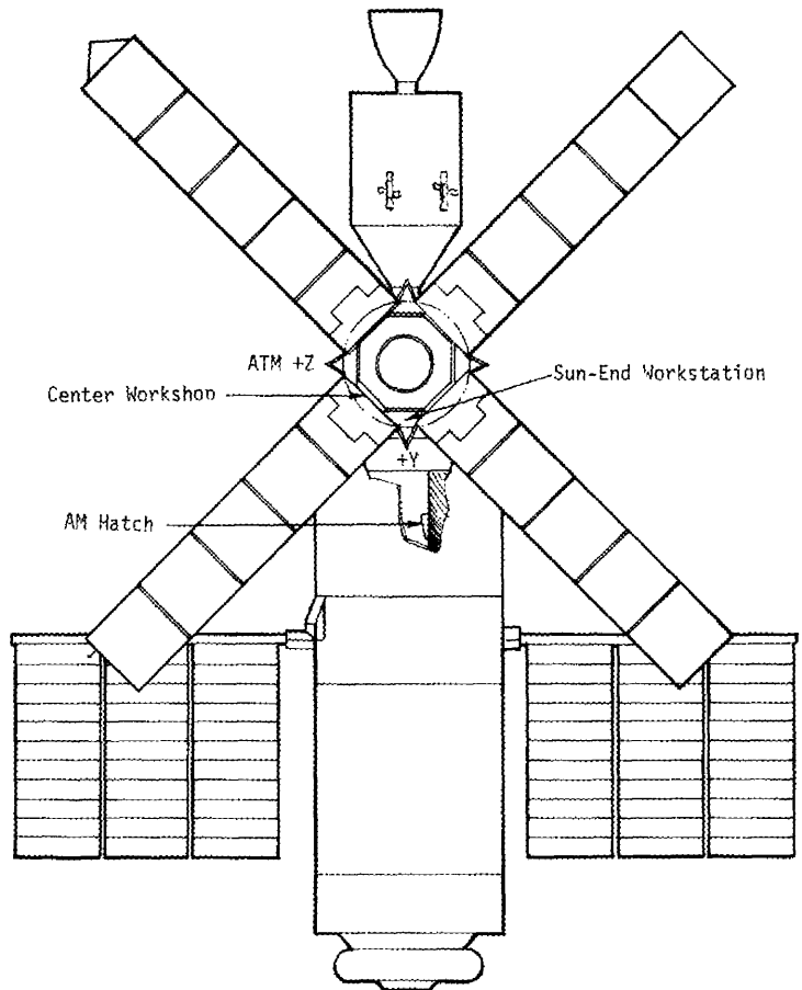
Figure 72. Skylab ATM Film Retrieval EVA Route
