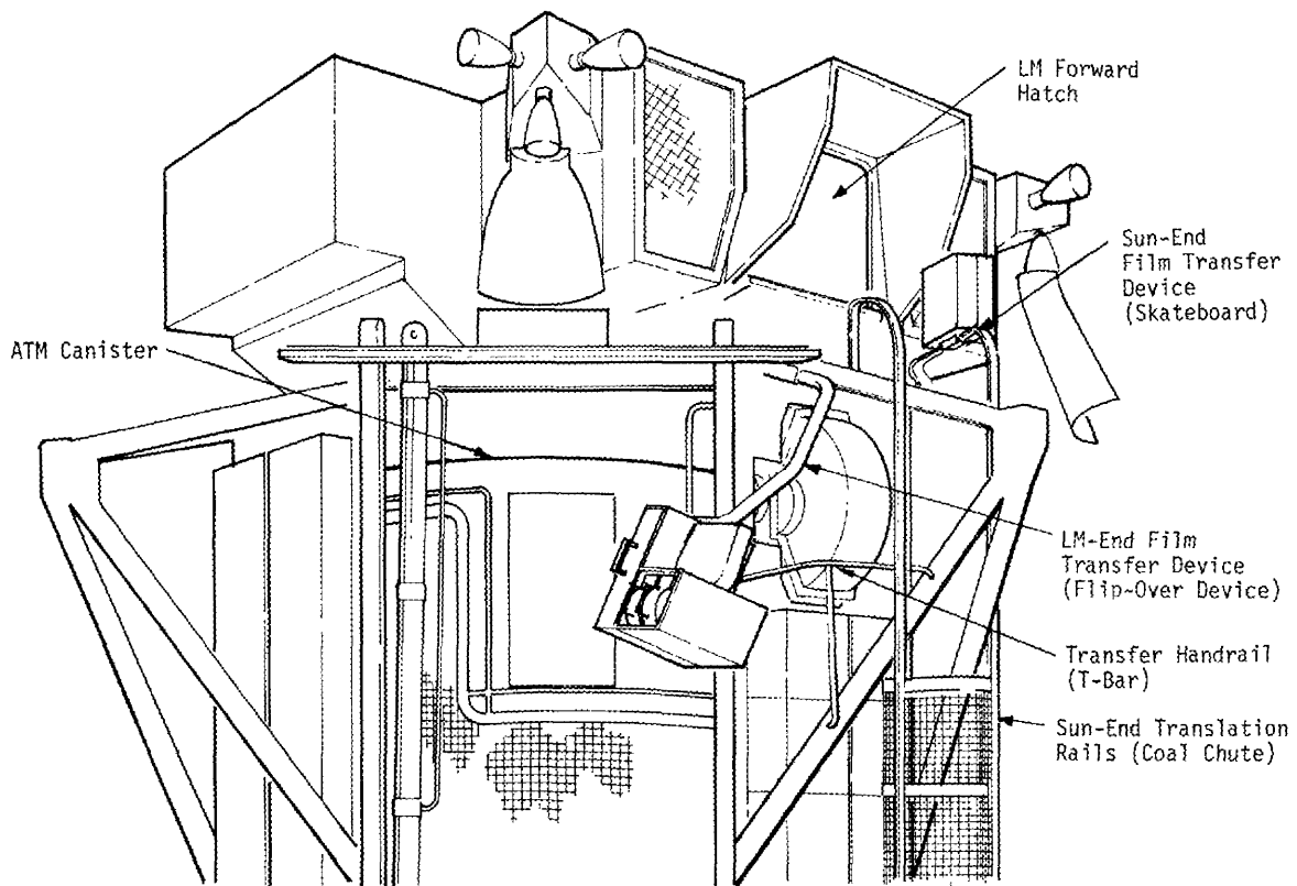
Figure 66. Parallel Rail Translation Concept and Film Transfer Devices
