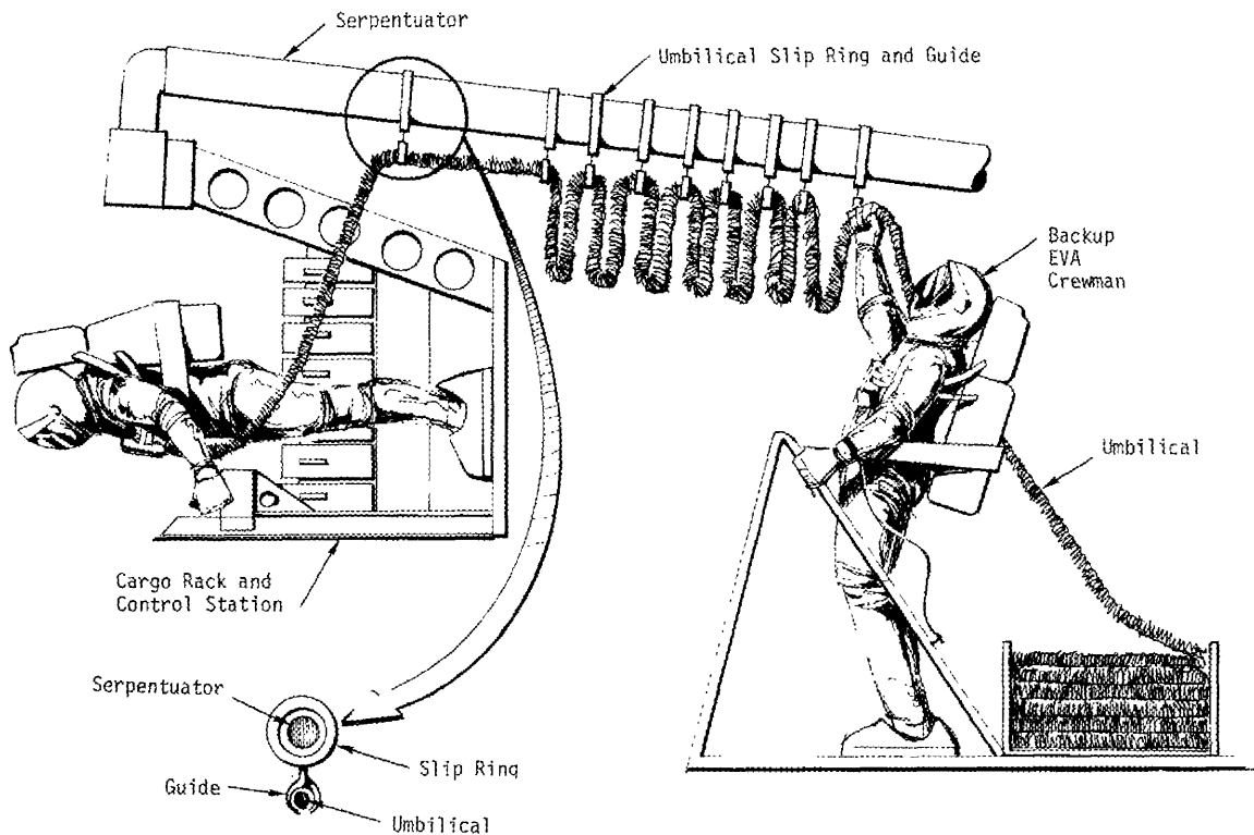
Figure 33. Serpentuator Umbilical Management and Cargo Carrier Concept
