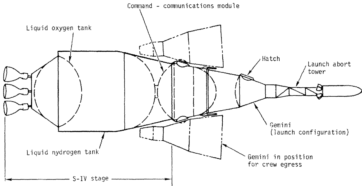
Figure 1. S-IV Stage - Gemini Space Laboratory Concept
