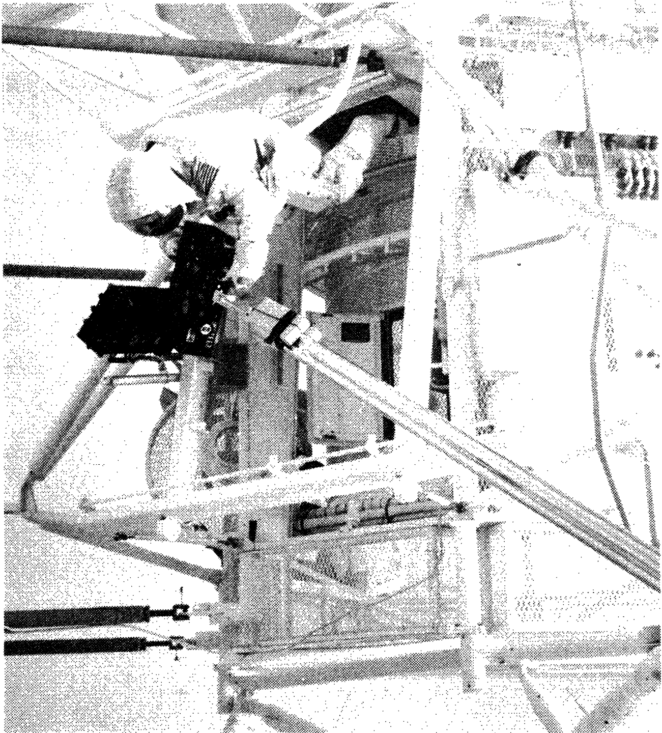
Figure 100. View of center workstation with crewman receiving replacement magazine on film transfer boom. The exposed magazine is secured to a temporary stowage hook on the clothesline bracket to the crewman's right.
