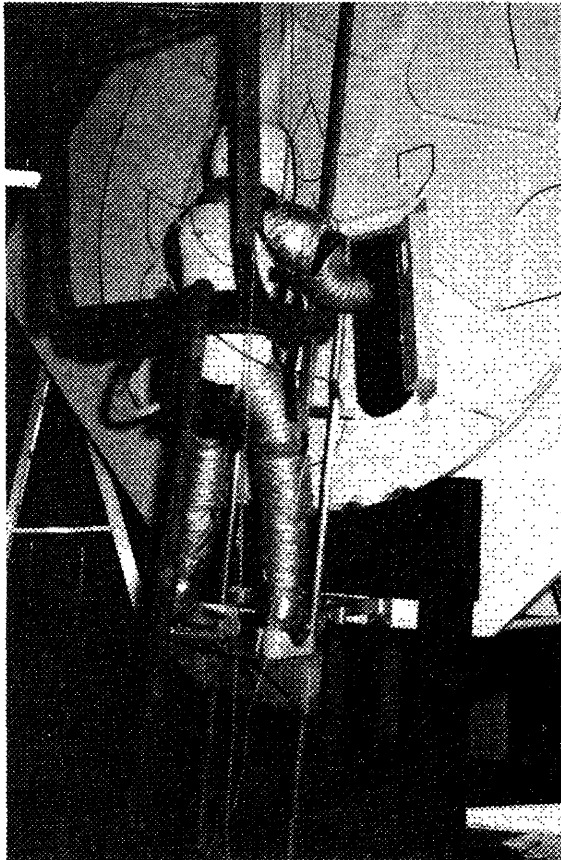
Figure 27. Dual-Rail Platform With Canister Rotated 95° Counterclockwise
