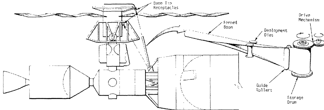
Figure 34. Roll-Up Extendible-Boom Deployment Concept
