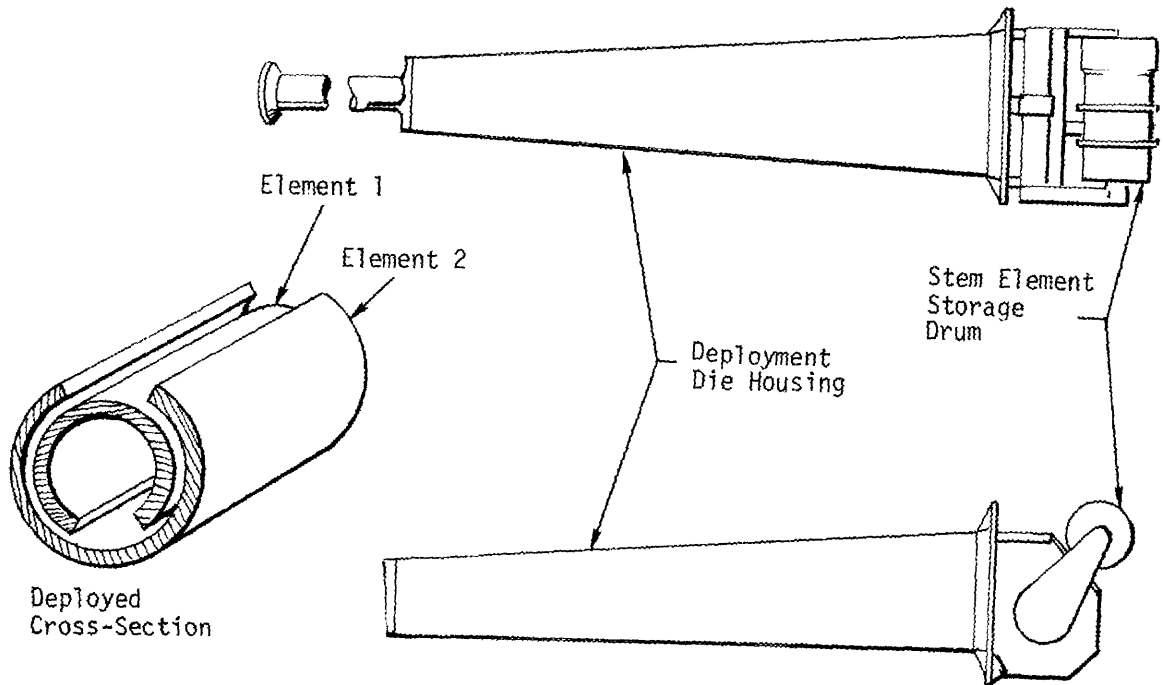
Figure 35. Bi-Storable, Tubular Extendible Member (STEM) Device
