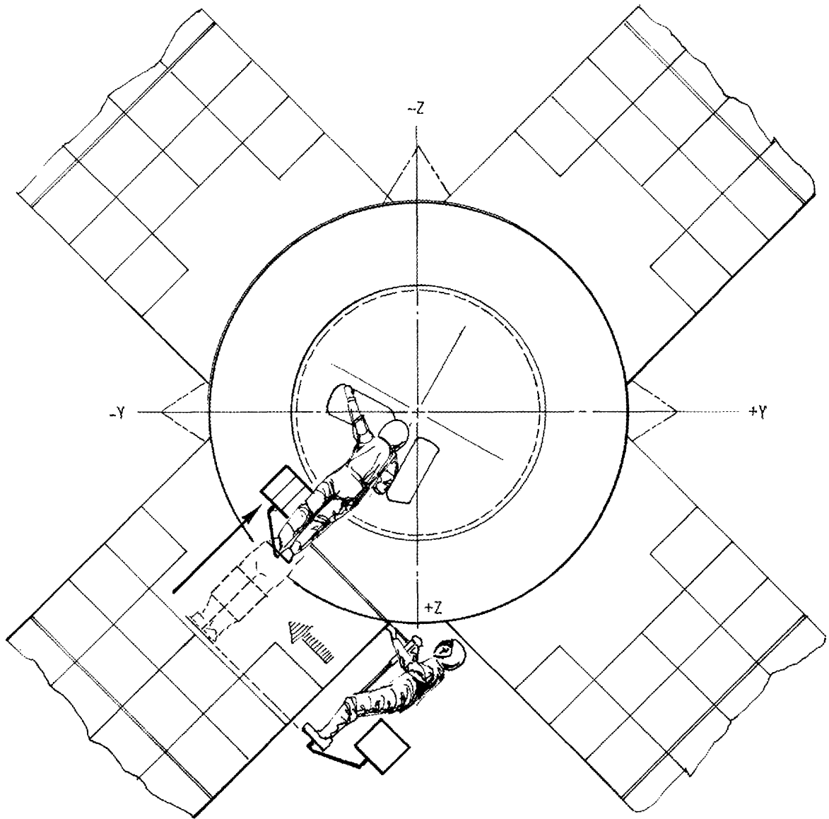
Figure 52. Trolley Sun-End Workstation Concept
