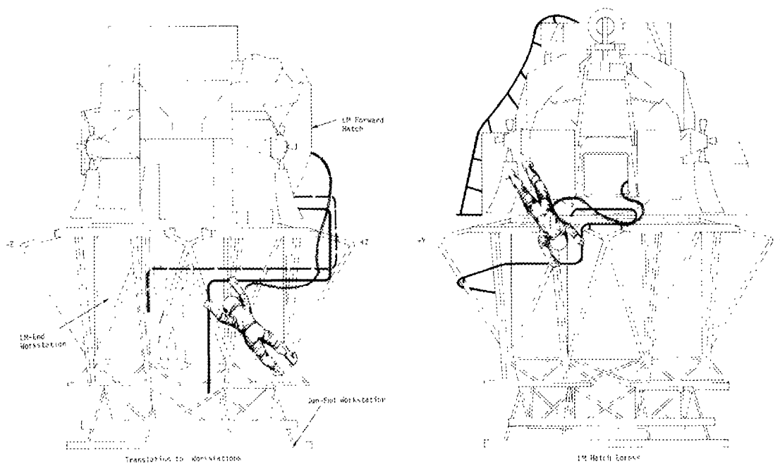
Figure 56. Single Rail Translation From LM Hatch
