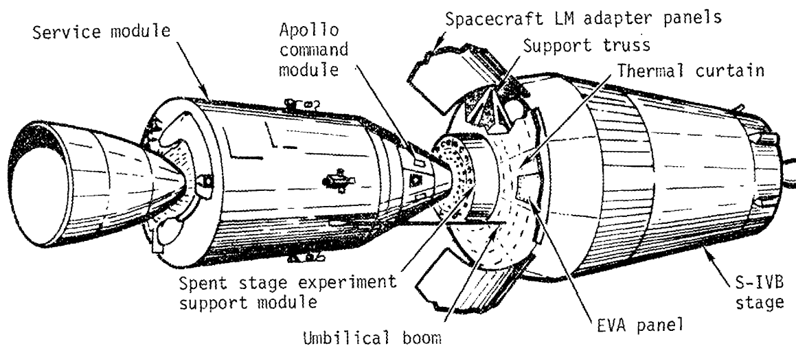
Figure 2. S-IVB Spent Stage Laboratory
