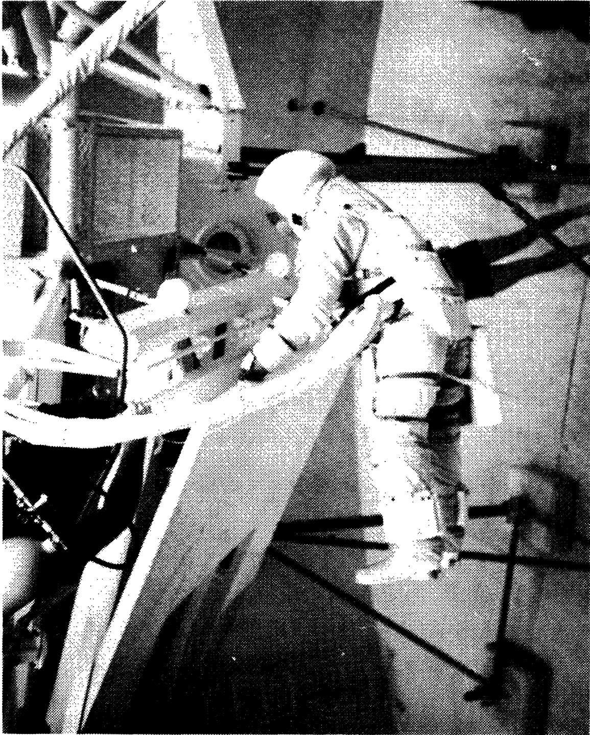
Figure 108. Crewman inspecting solar panel deployment hardware. After ascertaining that the mechanism is free of damage or jamming, he releases the panel launch lock by turning the torque tube with the socket wrench.
