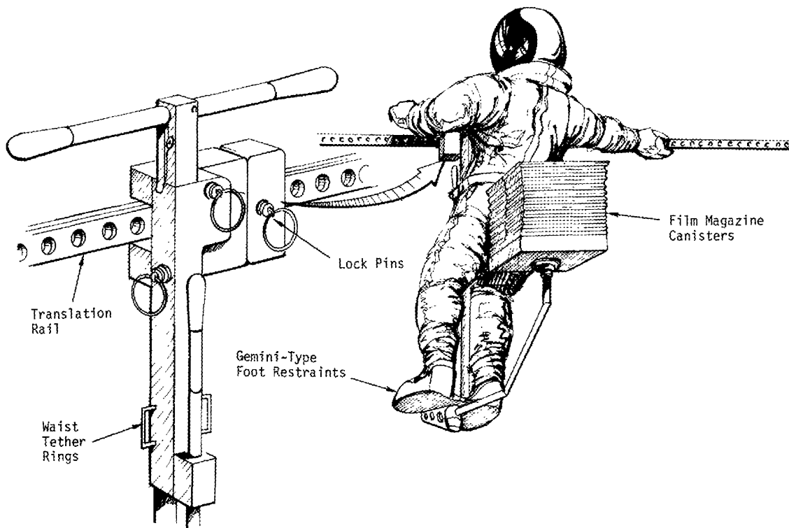
Figure 60. Translator or Trolley System
