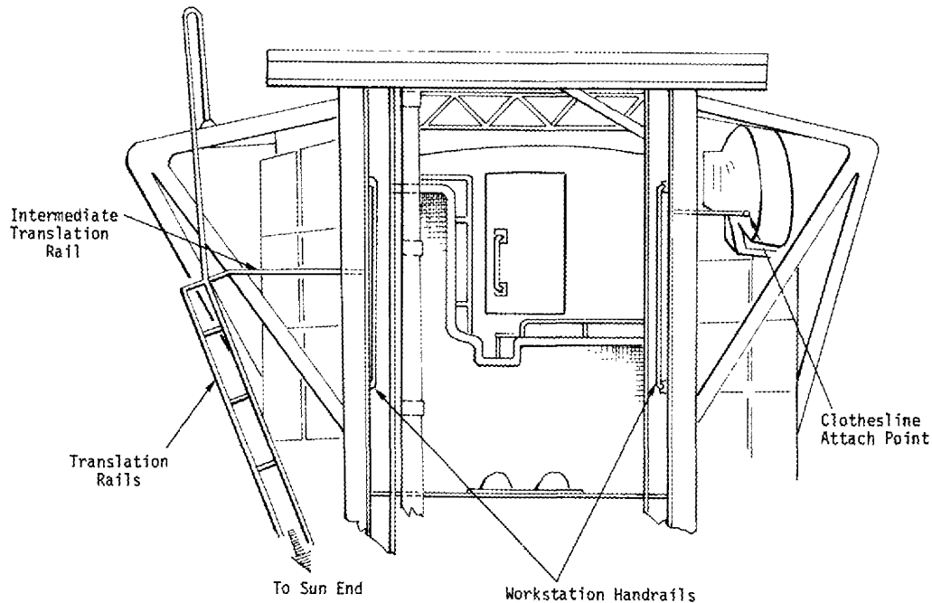
Figure 85. Center Workstation Mobility Aids and Film Transfer Provisions
