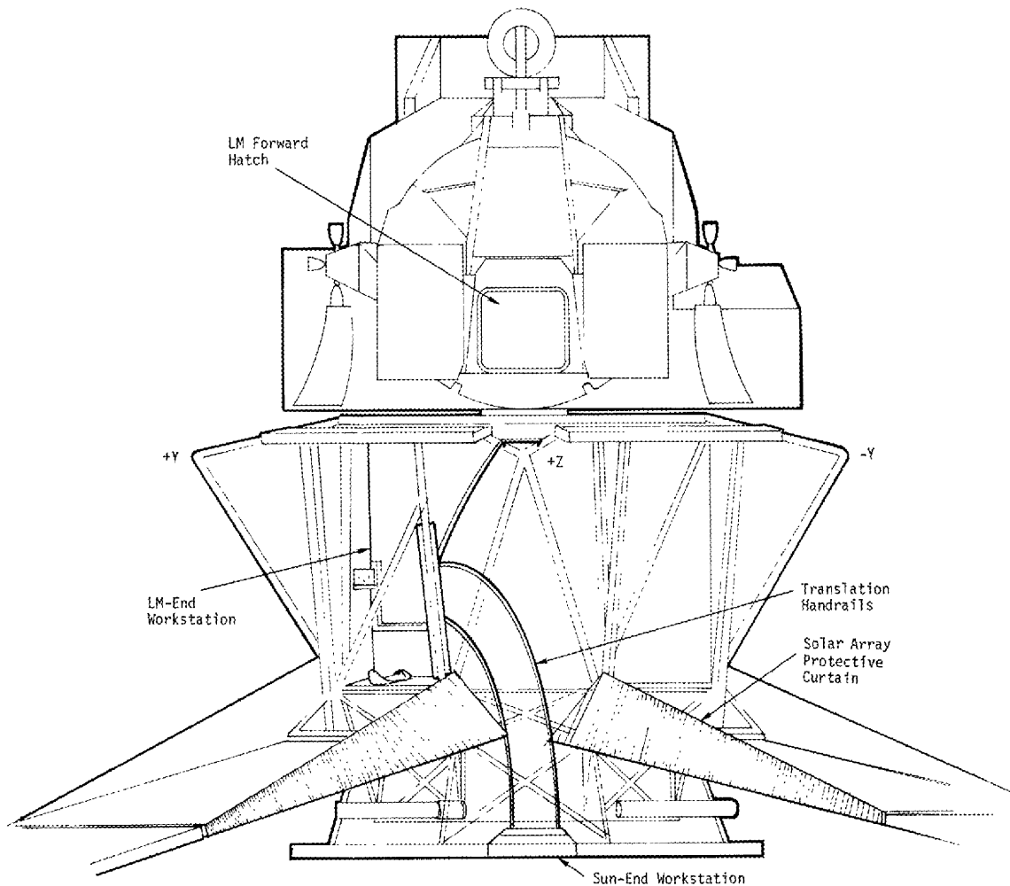
Figure 57. Proposed Workstation Relocation and Translation Rail Concept
