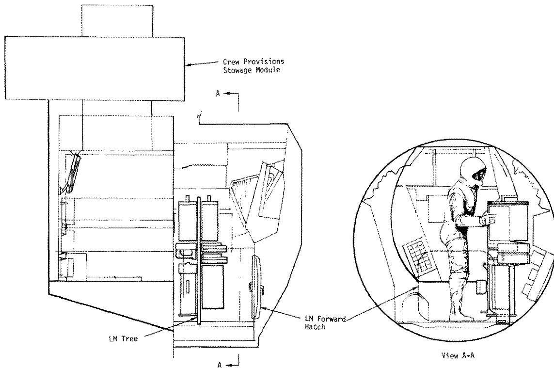
Figure 61. LM Interim Stowage Device in LM-A Forward Cabin Loading Position
