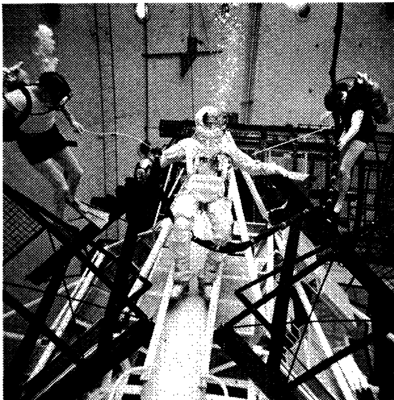
Figure 64. Neutral Buoyancy Stability Evaluation of the Trough Foot Restraint Concept
