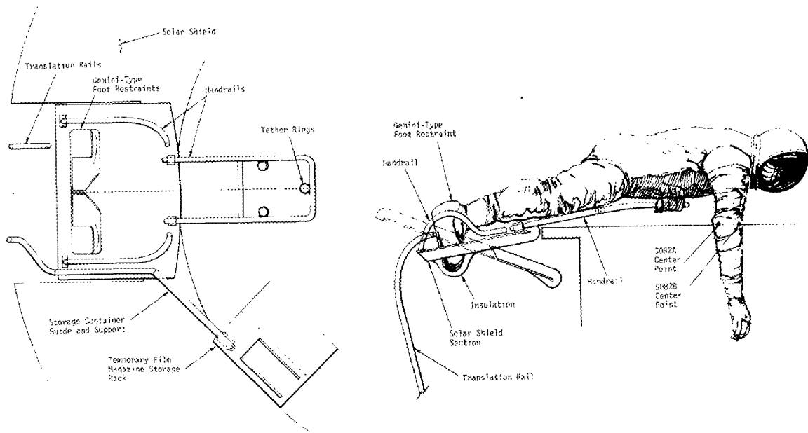
Figure 50. Deployable Sun-End Workstation Concept
