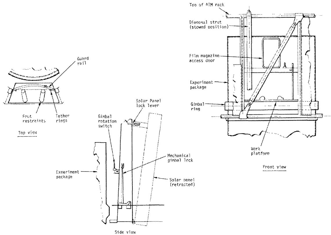
Figure 11. LM-End Workstation Configuration
