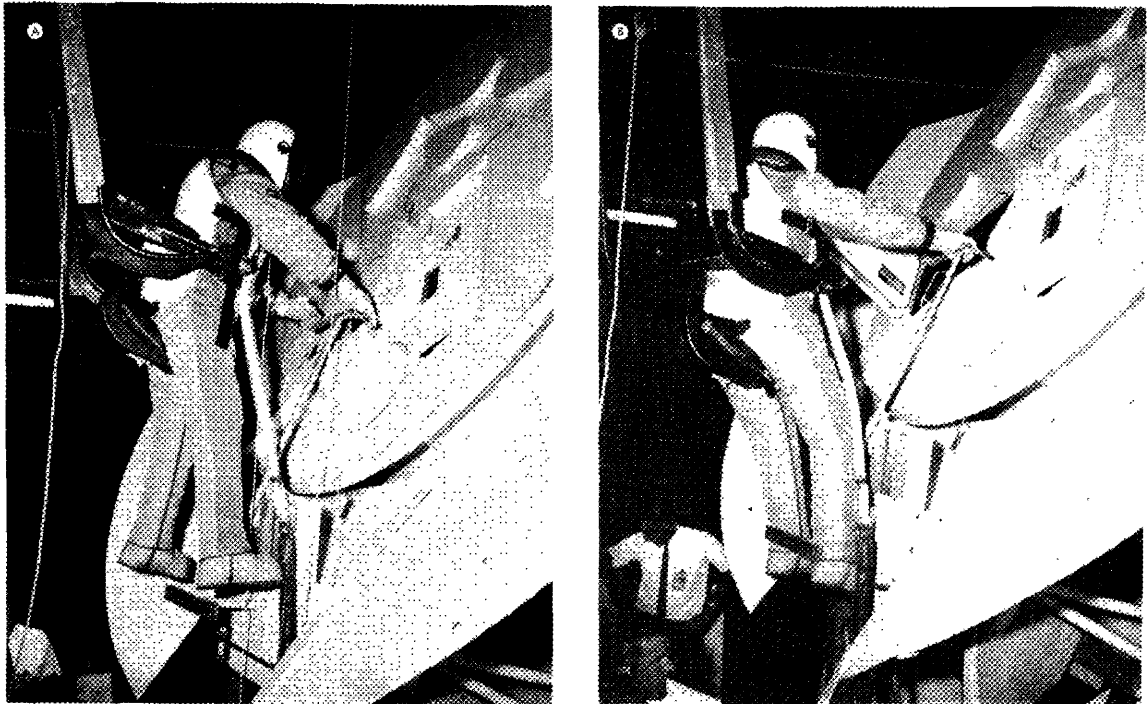
Figure 48. Workstation Foot Restraint and Stability Problems
