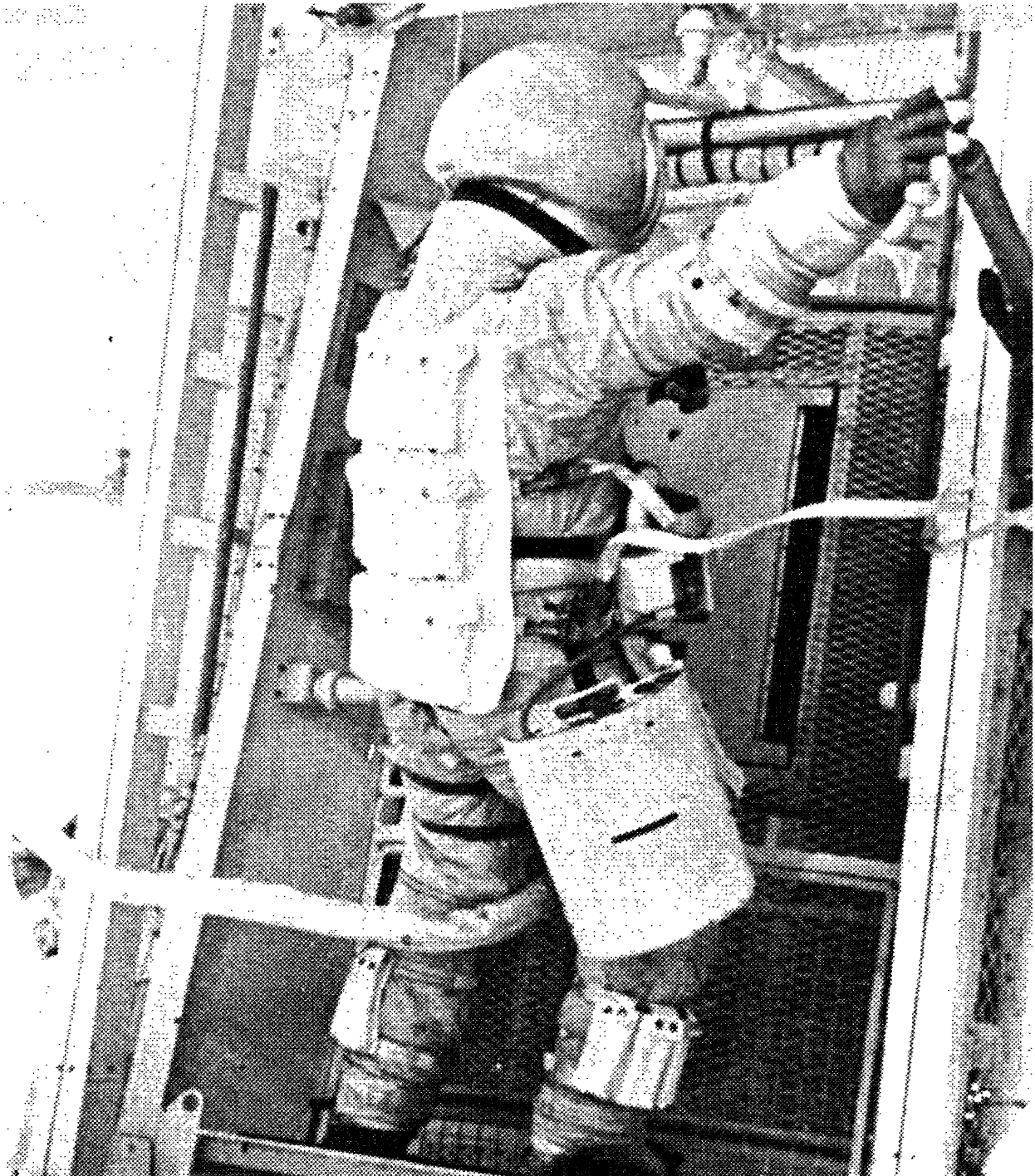
Figure 105. Crewman at center workstation attaching clothesline hook to deployed clothesline bracket.
