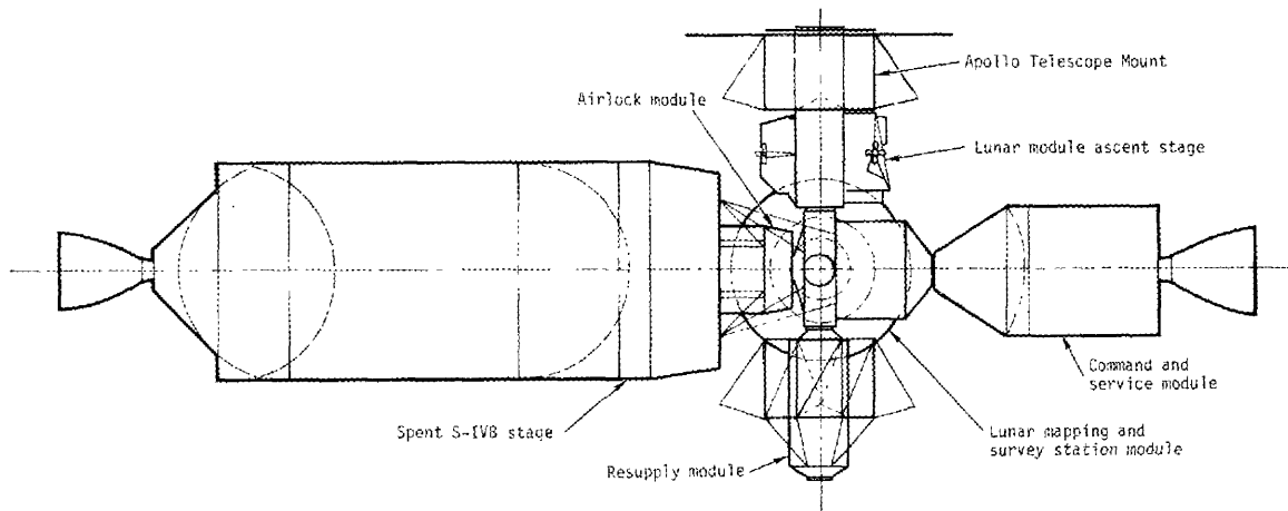
Figure 4. Early Clustered Workshop Concept
