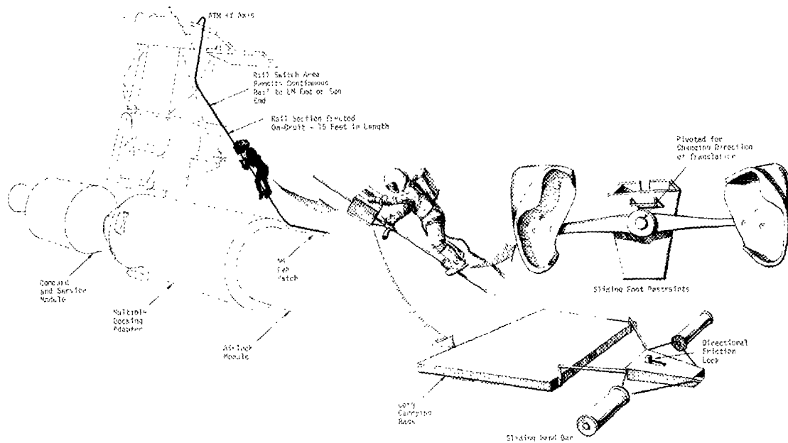
Figure 39. Continuous Rail Translation System
