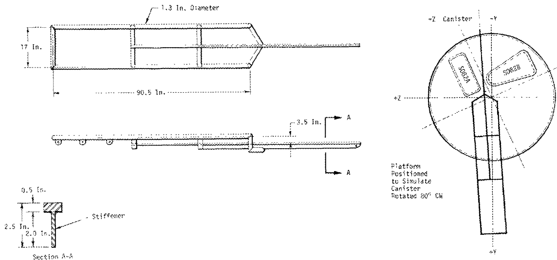
Figure 24, Dual Rail Workstation Platform Test Configuration
