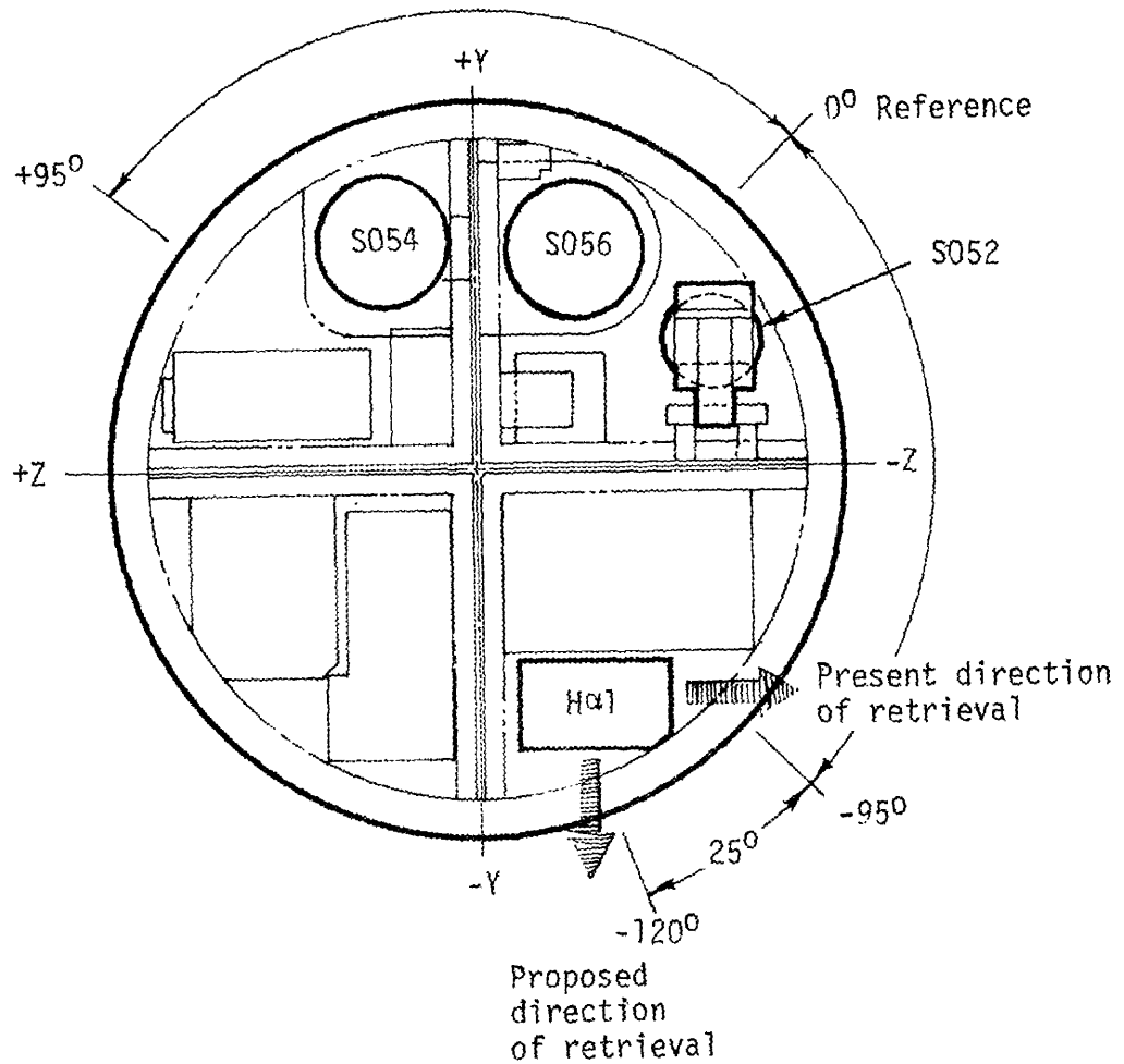
Figure 12. Canister Rotation Requirement for H-Alpha 1 Film Magazine Retrieval
