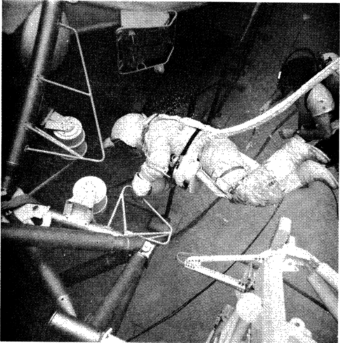
Figure 99. Crewman translating along deployment assembly handrails on the EVA route. The single handrail, shown below the crewman, leads to the ATM workstations.
