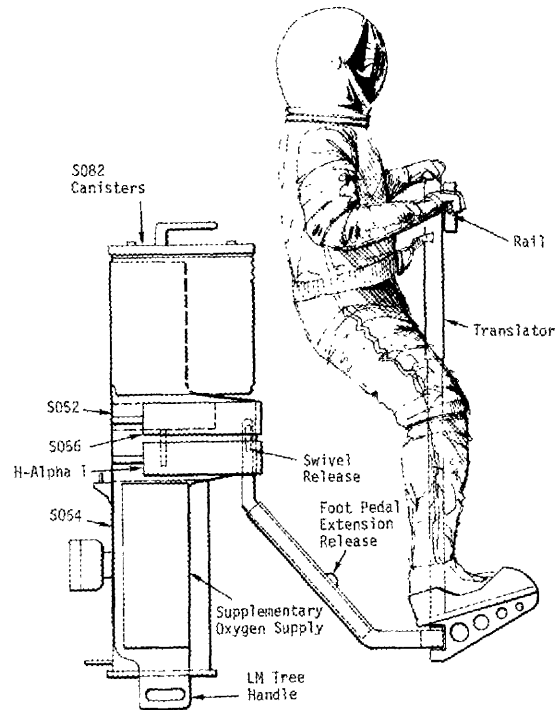
Figure 62. LM Interim Stowage Tree Attached to Trolley Translator
