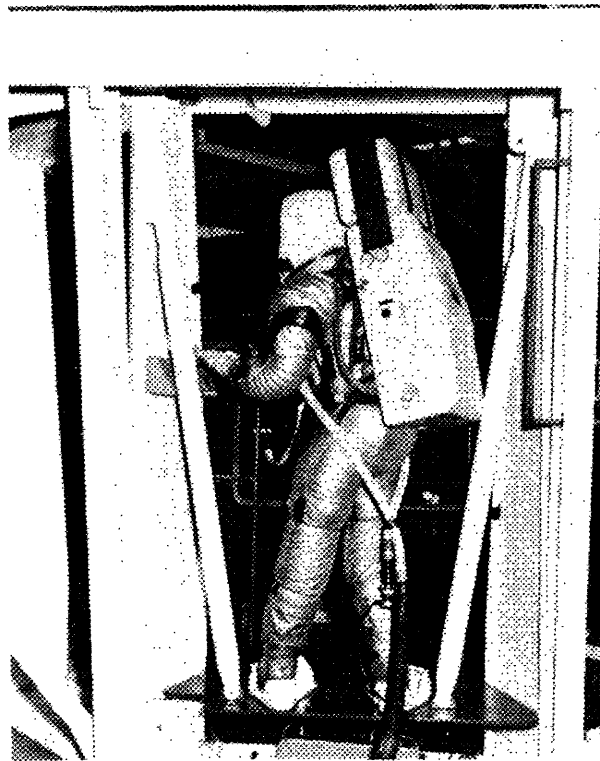
Figure 17. LM-End Workstation with Two Diagonal Struts
