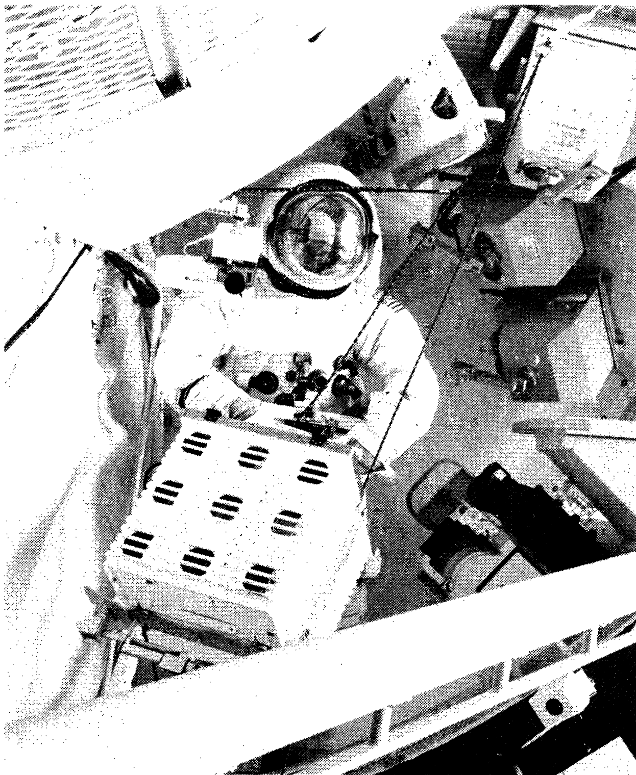
Figure 104. View of FAS workstation with deployed clotheslines. The crewman is attaching the sun-end clothesline hook to the film tree for transfer. The center workstation clothesline is kept out of the way with clips. The 16mm camera is shown in position to photograph the EVA.
