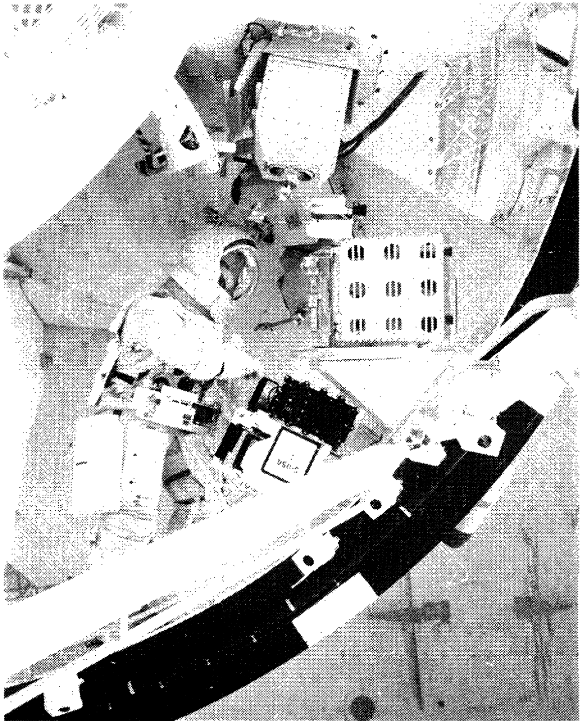
Figure 98. Crewman transferring center workstation film tree to temporary stowage receptacle. The 16mm camera is shown in a temporary stowage position.
