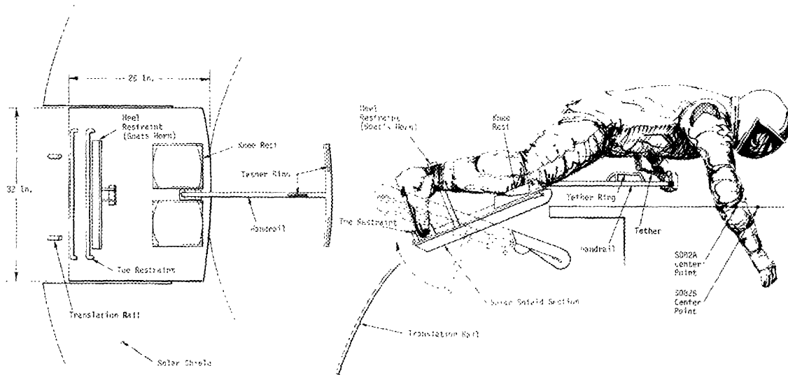
Figure 46. Sun-End Workstation Mounted on Rotating Solar Shield Section
