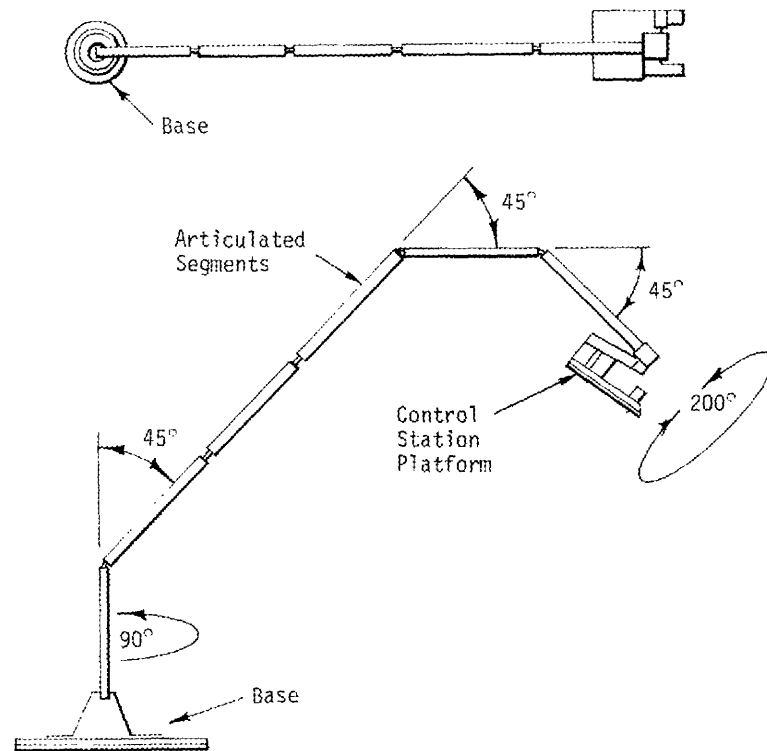
Figure 31. Serpentuator Concept
