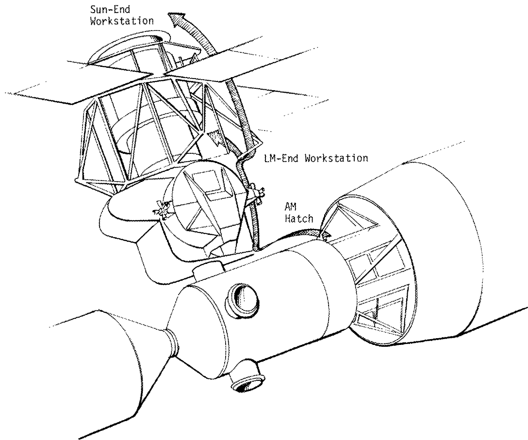
Figure 30. ATM Film Retrieval EVA Routes
