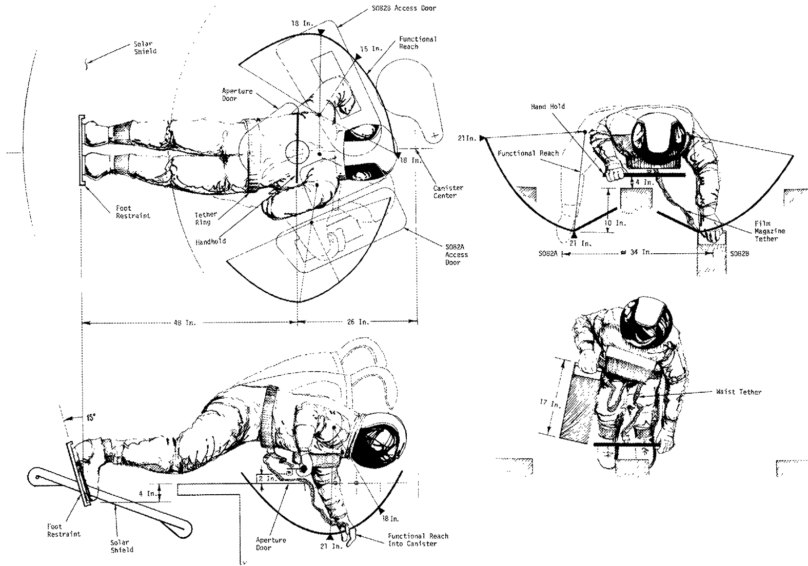
Figure 49. Sun-End Workstation Location Design Requirements
