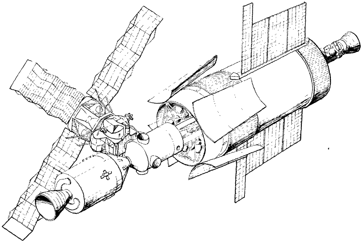
Figure 7. ATM Cruciform Solar Array and S-IVB Stage Solar Array
