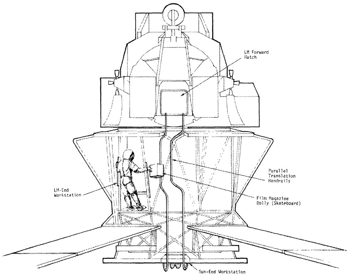
Figure 59. Parallel Translation Rails and Film Magazine Dolly Concept
