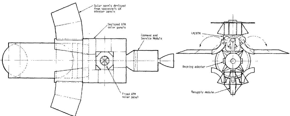
Figure 6. Early Cluster Solar Array Configuration
