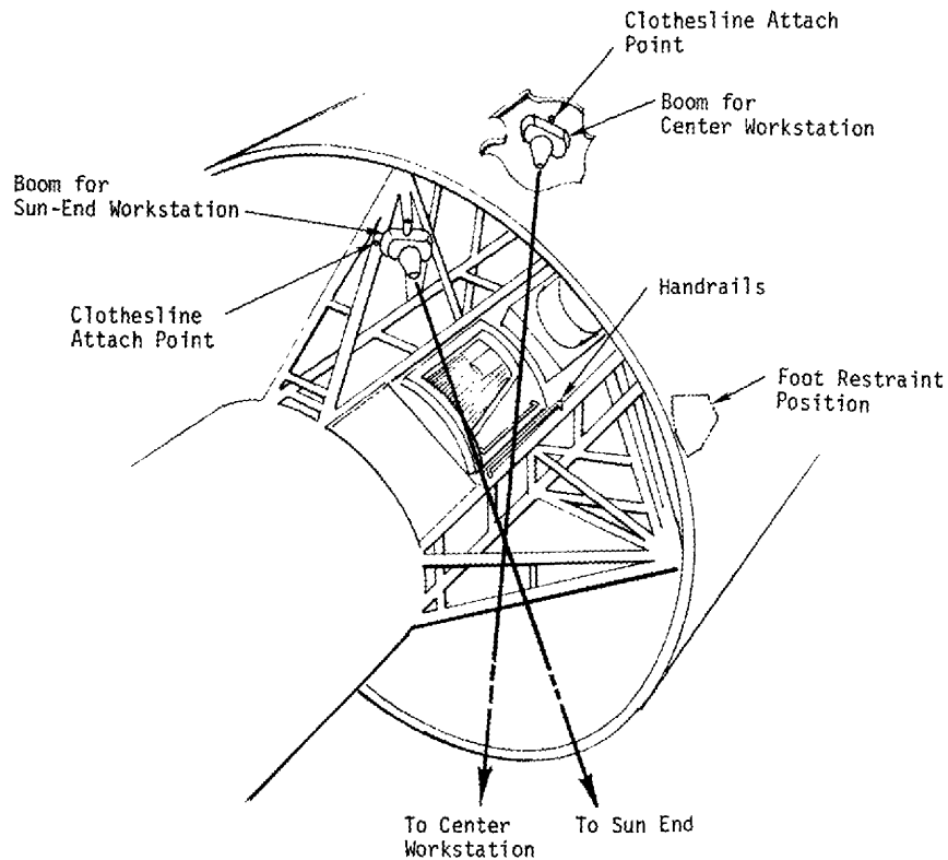
Figure 84. FAS Workstation Arrangement for Film Transfer Devices
