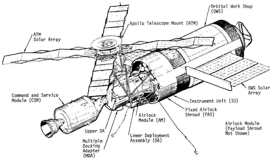
Figure 70. Skylab Cluster Configuration
