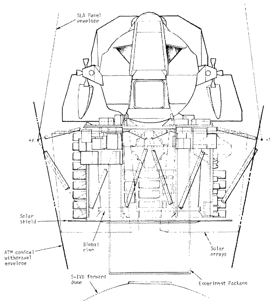
Figure 10. LM/ATM Configuration (June 1967)
