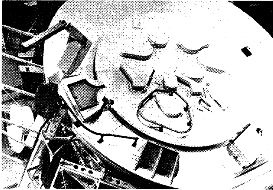
Figure 89. ATM Sun End Film Retrieval Components
