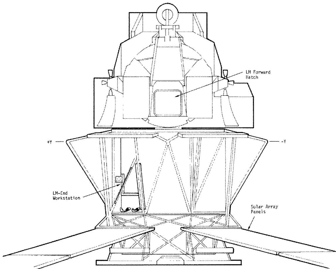
Figure 42. Proposed Workstation Relocation Concept
