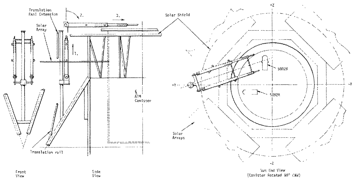
Figure 19. Ladder-Type, Telescoping Workstation (Concept IV)
