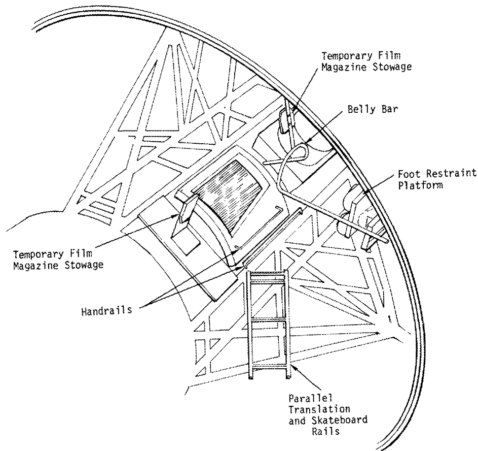
Figure 80. AM External or FAS Workstation Concept
