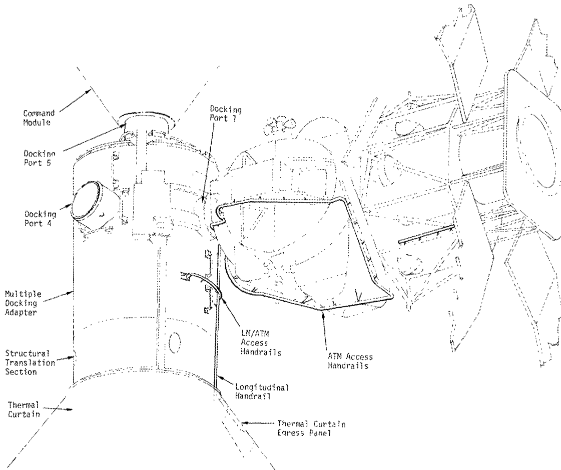
Figure 40. Cluster EVA Translation Handrail Locations
