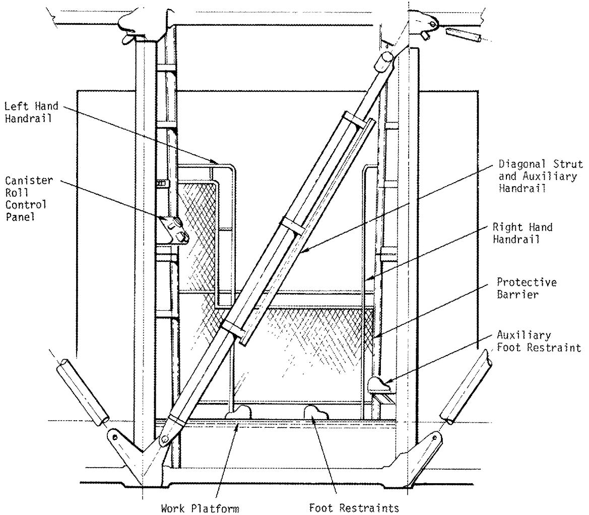
Figure 14. LM-End Workstation Evolution
