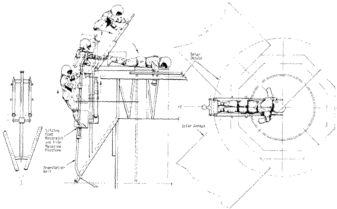
Figure 20. Combined Translation Rail and Ladder-Type Workstation (Concept IV)
