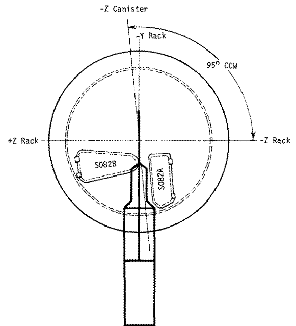
Figure 27. Dual-Rail Platform With Canister Rotated 95° Counterclockwise
