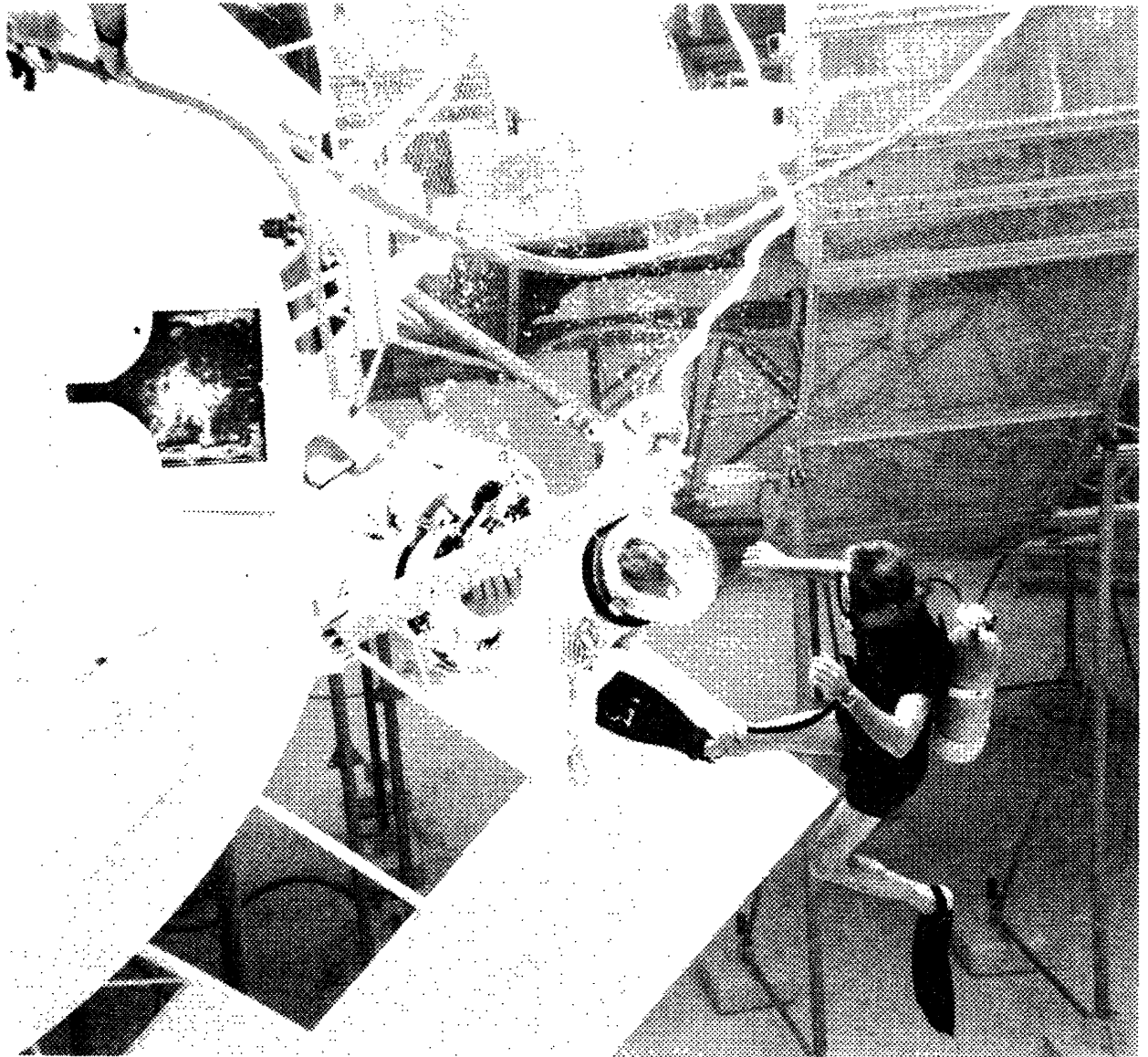
Figure 106. Crewman at transfer workstation has deployed the sun-end clothesline bracket and is attaching the clothesline hook.
