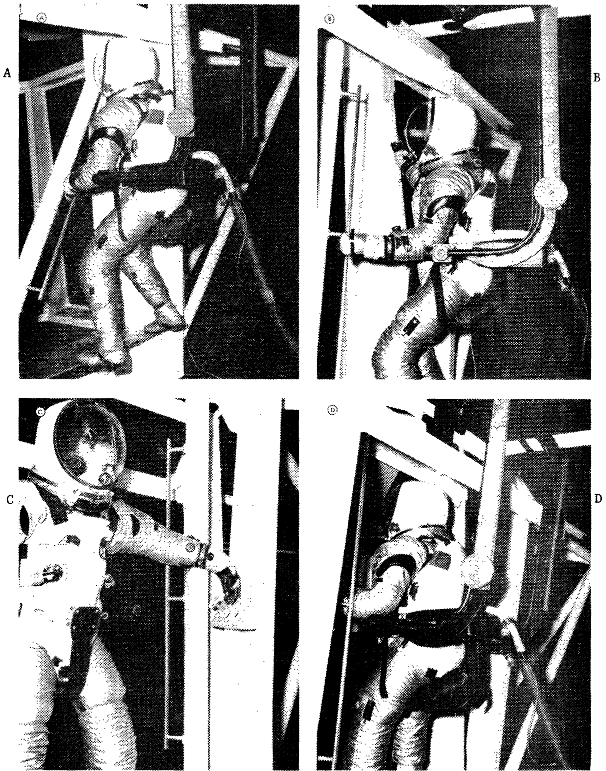
Figure 13. LM-End Workstation Simulation Showing Structural Interference
