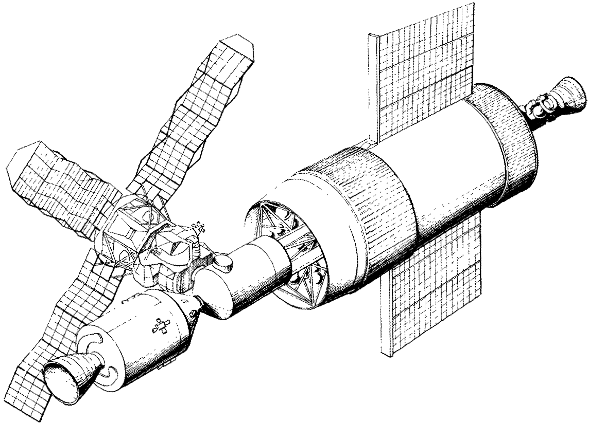
Figure 41. Final Wet Workshop Orbital Configuration
