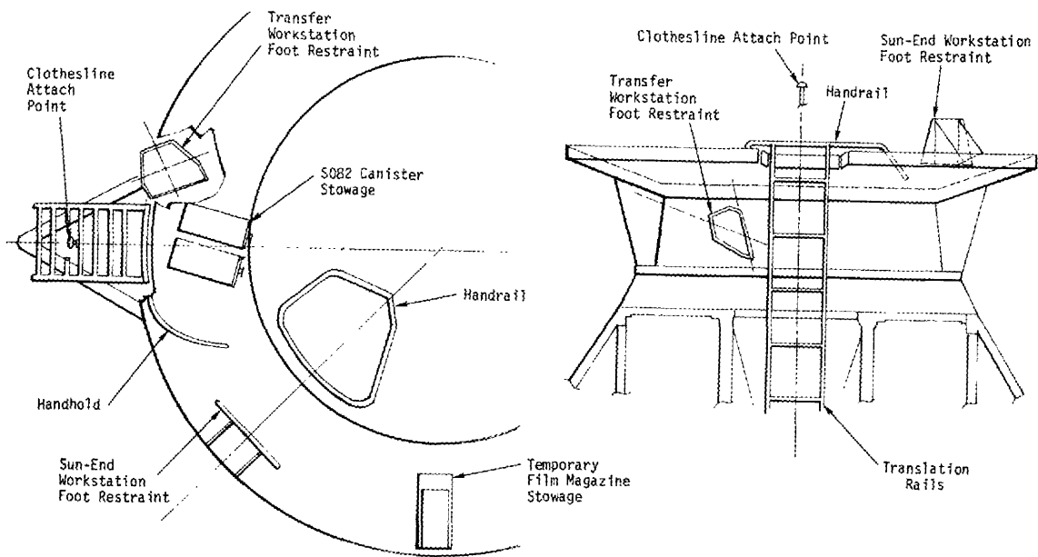
Figure 86. Transfer and Sun-End Workstation Arrangement
