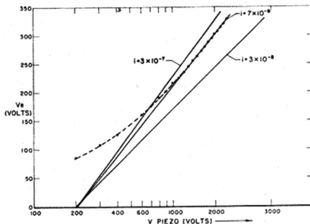
FIG. 16. Experimental curves corresponding to Fig. 15 for three different currents. Since solutions of Laplace's equation are independent of current density, all three curves extrapolate to the same piezo voltage, corresponding to an emitter radius of 8100 Å. Emitter radius = R_e ; R_e = 3 \times 208 \times 13.0 = 8100 Å.
