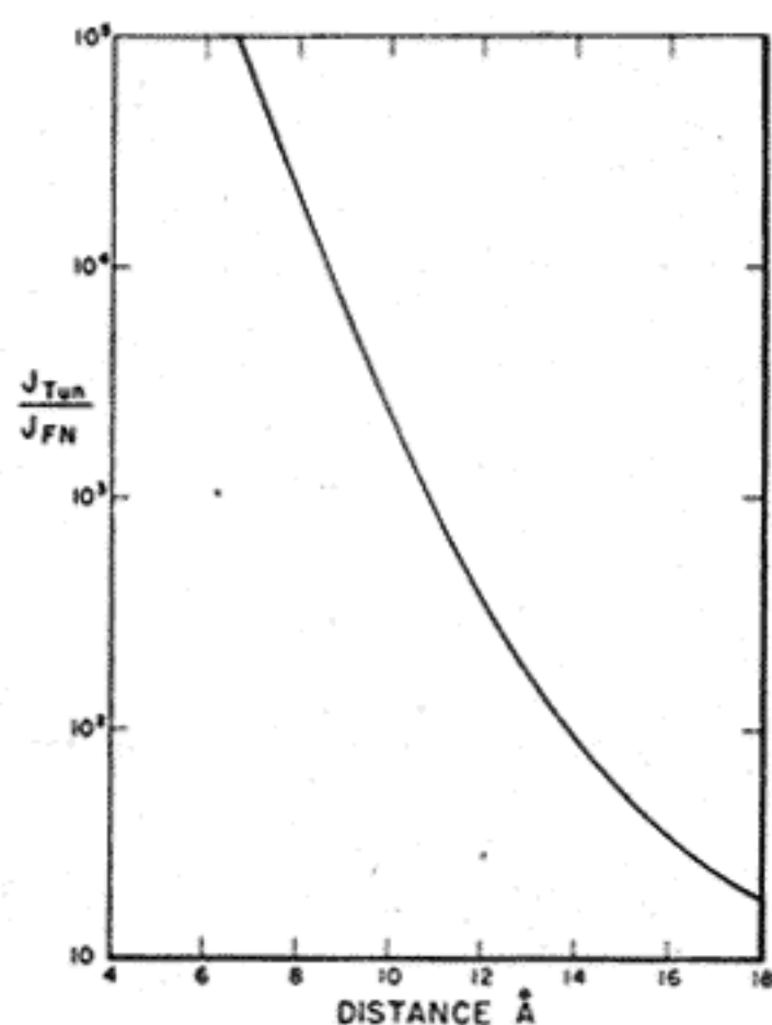
FIG. 21. Calculated ratio of tunneling current density to Fowler-Nordheim predicted current for a fixed field at the emitter of 0.3 \text{ V/\AA} .
