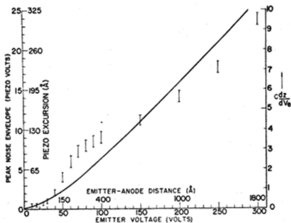
FIG. 8. Comparison of peak noise voltage (solid curve) with reciprocal of servo loop gain [ =CdZ/dV_e (data points—error bars)] as the emitter voltage (emitter spacing) is varied. The ordinate on the left is also labeled in terms of the peak piezo excursion associated with the noise. As expected, the noise increases approximately as the reciprocal of the servo loop gain. The deviation at about 100 V is not understood.
