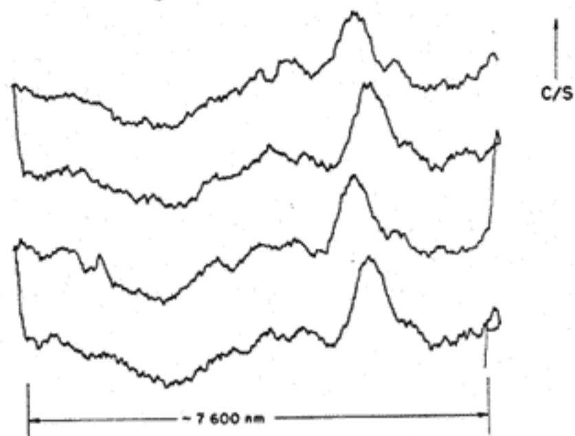
FIG. 13. Secondary electron profiles as emitter is scanned over the surface of a thermally etched Ta strip. The main features are quite reproducible. V_e = 160 V; V_{mult} = 2800 V; V_{horn} = 100 V; \sim 10^3 counts/sec.
