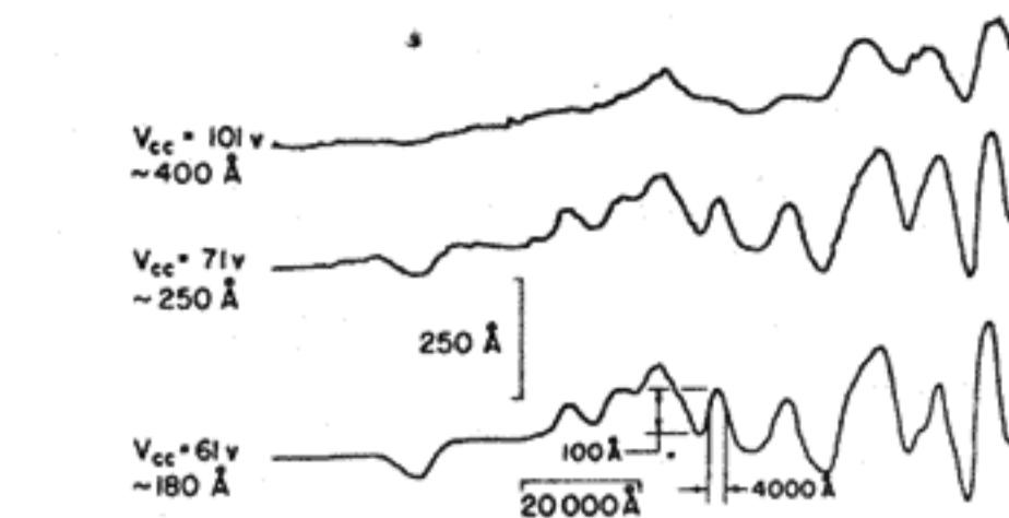
FIG. 11. Magnified profile of a defective region on the same surface as Fig. 10. Note the strong influence of emitter spacing (indicated just below emitter voltage V_{cc} ) on the noise and the detail resolved in the surface structure. Topographic maps are usually taken at about 50–60 V. R_e \sim 1300 Å.
