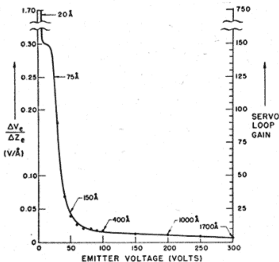
FIG. 6. Dependence of servo loop gain on emitter voltage. The gain of the servo loop depends on the slope of the emitter voltage vs emitter spacing curve ( \Delta V_e/\Delta Z_e ). The emitter spacing is indicated at several points along the curve. The drastic increase in servo loop gain at very low emitter voltages will be discussed in the section on MVM tunneling.
