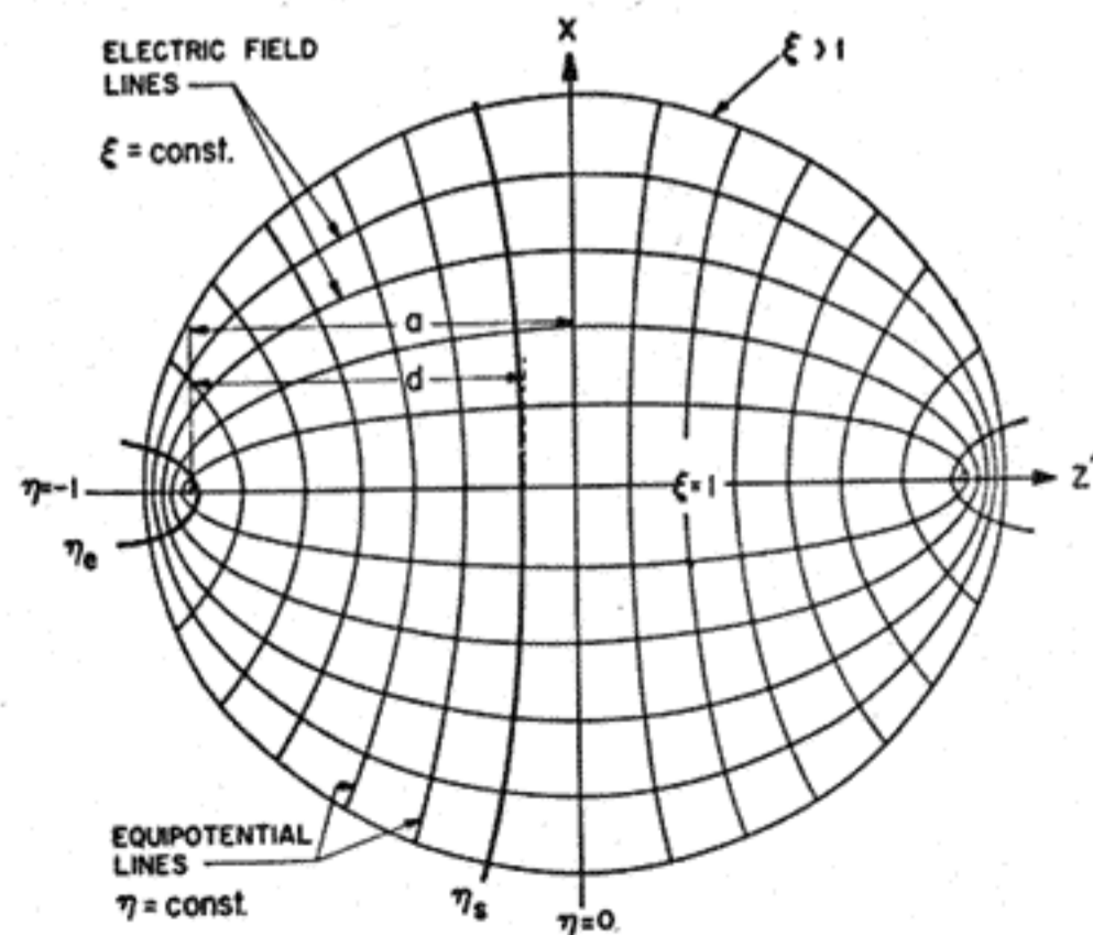
FIG. 14. Prolate spheroidal coordinate system. \eta_e is the equipotential contour corresponding to the emitter surface, \eta = 0 corresponds to the specimen or anode.
