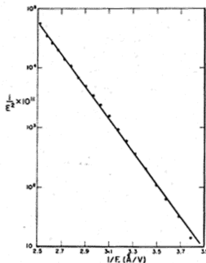
FIG. 18. Fowler-Nordheim plot taken with emitter spacing of about 1000 \text{ \AA} . The field strength was determined from Fig. 17.
