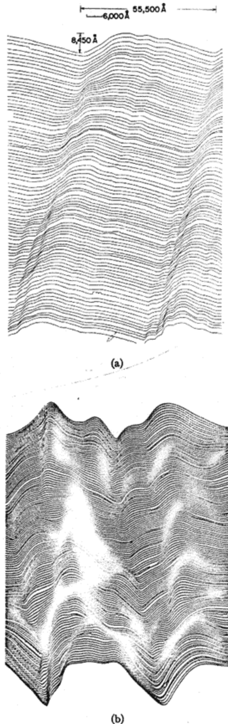
FIG. 3. (a) Topographic map of a 180 line/mm diffraction grating replica. This map was made with the instrument in Fig. 1 using an X-Y recorder. Note the rippled surface at the base of the groove which may have been caused by ruling instrument chatter or replica removal. Details of the diamond tool used in the ruling engine are evident. The emitter was kept about 200 \text{ \AA} above the surface during these runs. (b) Topographic map recorded on a memory oscilloscope of a disturbed region of the same grating as (a). The vertical magnification is about twice the horizontal magnification. The contrast is reversed for easy comparison with (a). The close spaced profiles give a highly desirable pictorial representation of the surface topography. Mapping time—9 min.
