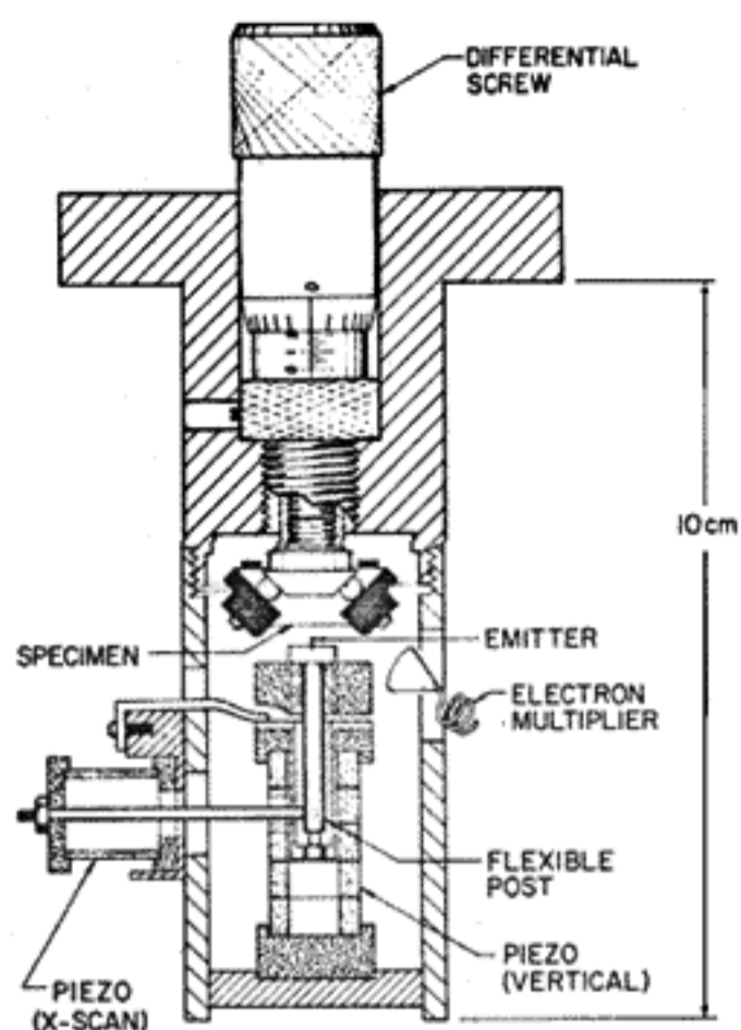
FIG. 1. Present realization of the Topografiner. The differential screw is used as a coarse adjustment to bring the specimen close enough to the emitter so that it is within the range of the vertical ( Z ) piezo. The X -scan piezo deflects the emitter support post so as to scan the emitter in one direction. The orthogonal ( Y ) piezo is not shown. The specimen is clamped between copper blocks to permit heating. An electron multiplier permits detection of secondary electrons.
