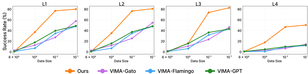
Figure A.21: Data scaling when baseline variants’ ViT is trained from scratch. In settings with reasonable amounts of in-domain data (i.e., the 1%, 10%, and 100% scenarios), our recommended recipe always outperforms other variants.
