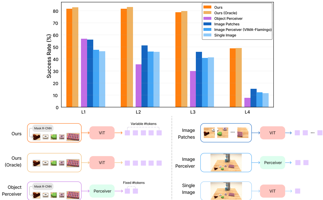
Figure 6: Ablation on visual tokenizers. We compare the performance of VIMA-200M model across different visual tokenizers. Our proposed object tokens outperform all methods that learn directly from raw pixels, and Object Perceiver that downsamples the object sequence to a fixed number of tokens.
