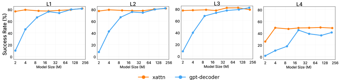
Figure 7: Ablation on prompt conditioning. We compare our method ( xattn : cross-attention prompt conditioning) with a vanilla transformer decoder ( gpt-decoder ) across different model sizes. Cross-attention is especially helpful in low-parameter regime and for harder generalization tasks.
