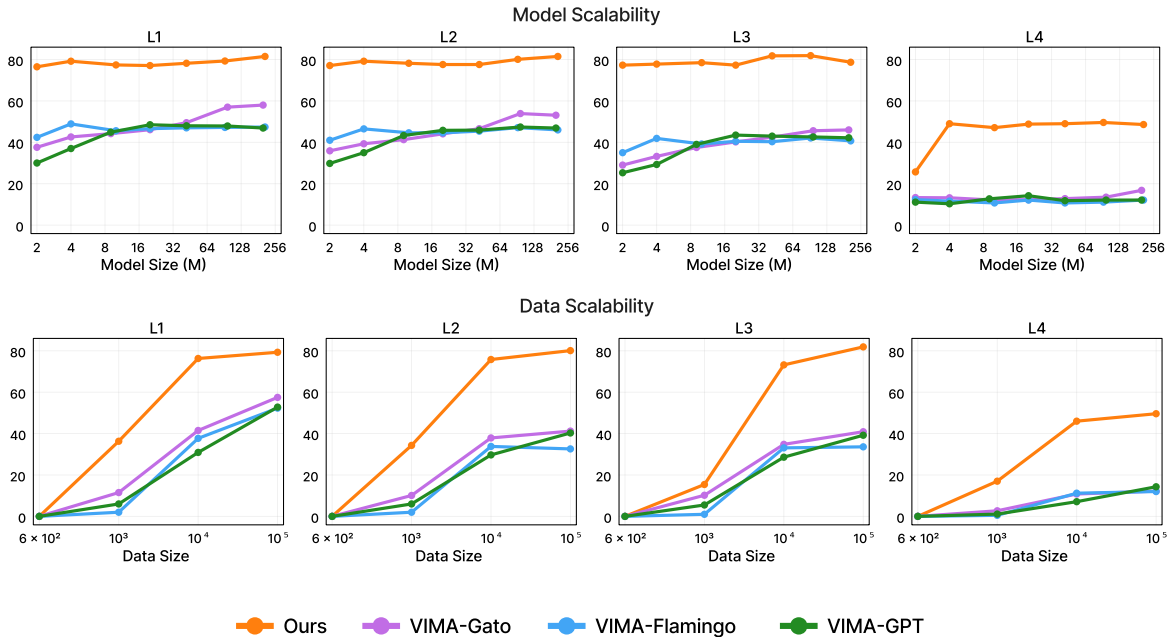
Figure 4: Scaling model and data. Top: We compare performance of different methods with model sizes ranging from 2M to 200M parameters. Across all model sizes and generalization levels, VIMA outperforms baseline variants. Bottom: For a fixed model size of 92M parameters we compare the effect of imitation learning dataset size with 0.1%, 1%, 10%, and full data. VIMA is extremely sample efficient and can achieve performance comparable to other methods with 10× less data.
