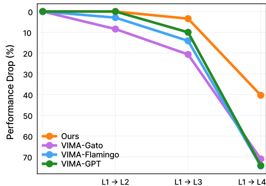
Figure 5: VIMA incurs much less performance drop than baselines as we evaluate on progressively harder settings.
