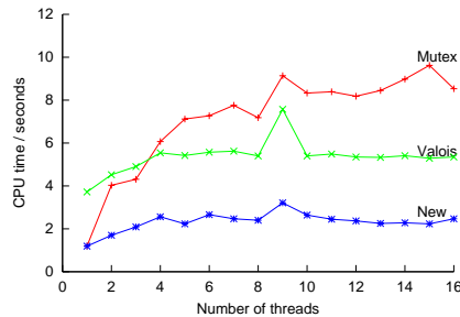
(b) Non-reference-counted algorithms with keys 0...255.
