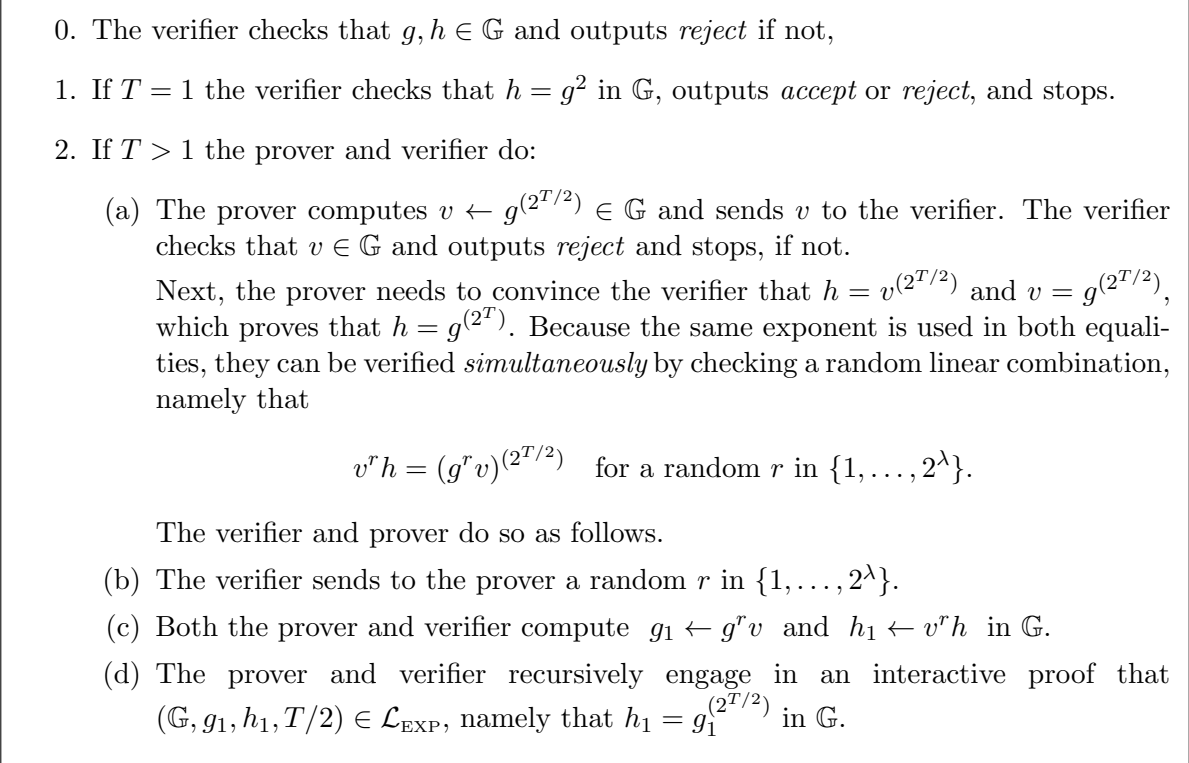
Figure 1: Pietrzak’s succinct argument for (\mathbb{G}, g, h, T) \in \mathcal{L}_{\text{EXP}}
