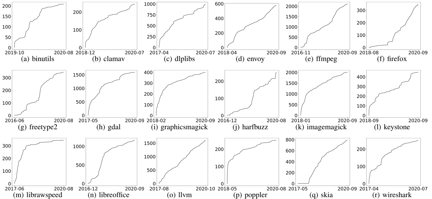
Fig. 9: Cumulative numbers of bugs found in projects with >200 bugs. The numbers of bugs found over time often exhibit punctuated equilibria, a common phenomenon in genetic algorithms such as those used in coverage-guided fuzzers.
