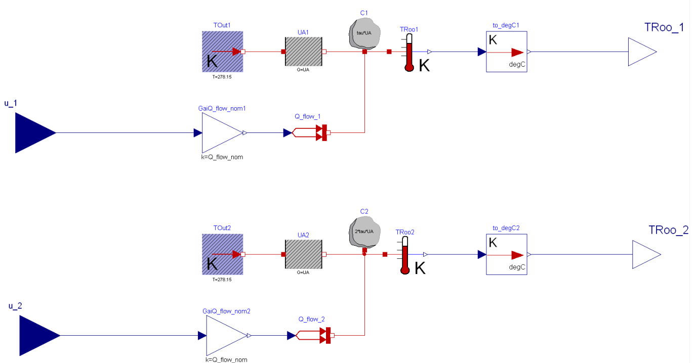
Figure 5.25: Graphical view of the Modelica model that is exported as an FMU for co-simulation.
