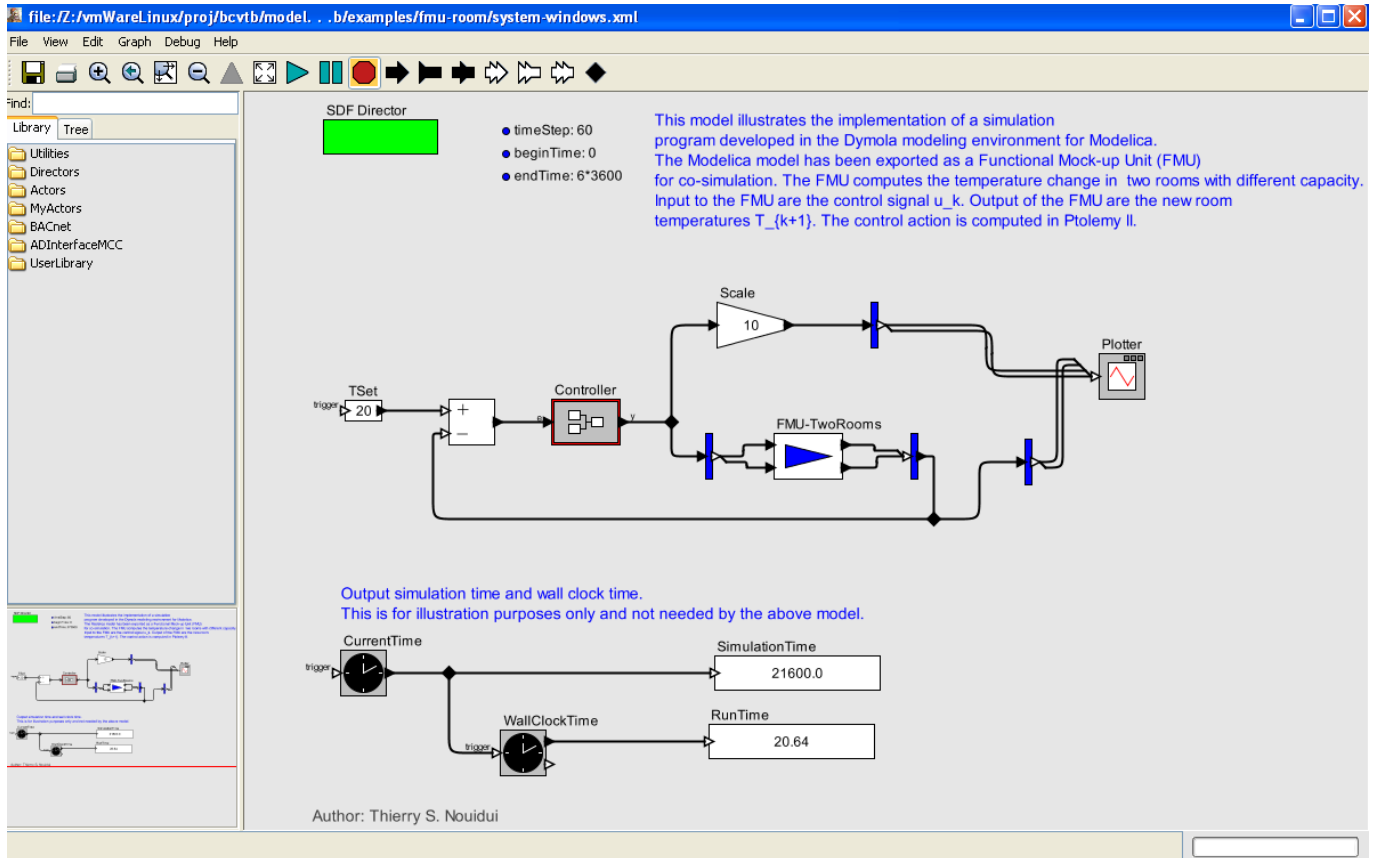
Figure 5.26: Ptolemy II system model that links a model of a controller with the FMU for co-simulation.
