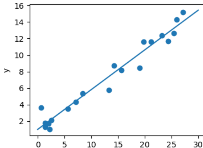
Fig. 4: A plot of a simple linear regression.
