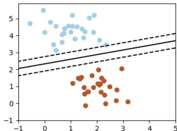
Fig. 1: A classification problem
