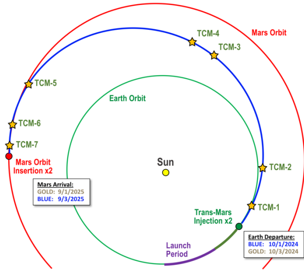
Figure 2. ESCAPADE's Interplanetary Cruise
