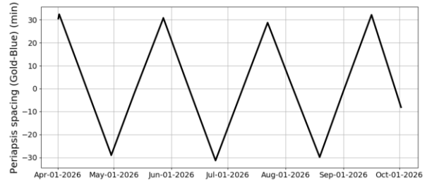
Figure 9. The relative spacing between Blue and Gold during Science Campaign A.
