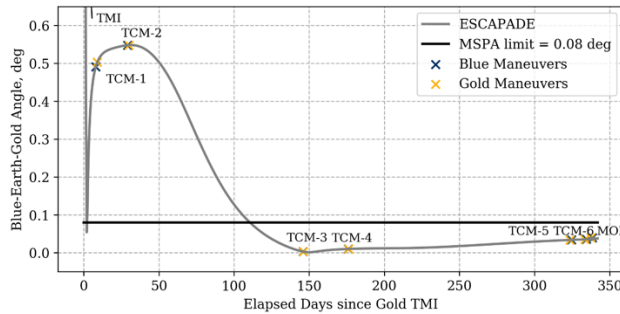
Figure 3. The angle between each ESCAPADE spacecraft and the Earth, to evaluate the timeline when MSPA is available with the DSN.
