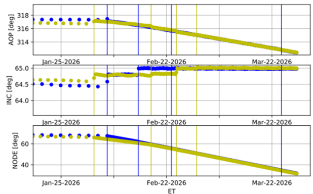
Figure 6. The TSF Phase’s nominal time profile for the argument of periapse, inclination, and longitude of node, all in the IAU Mars Pole coordinate frame,
