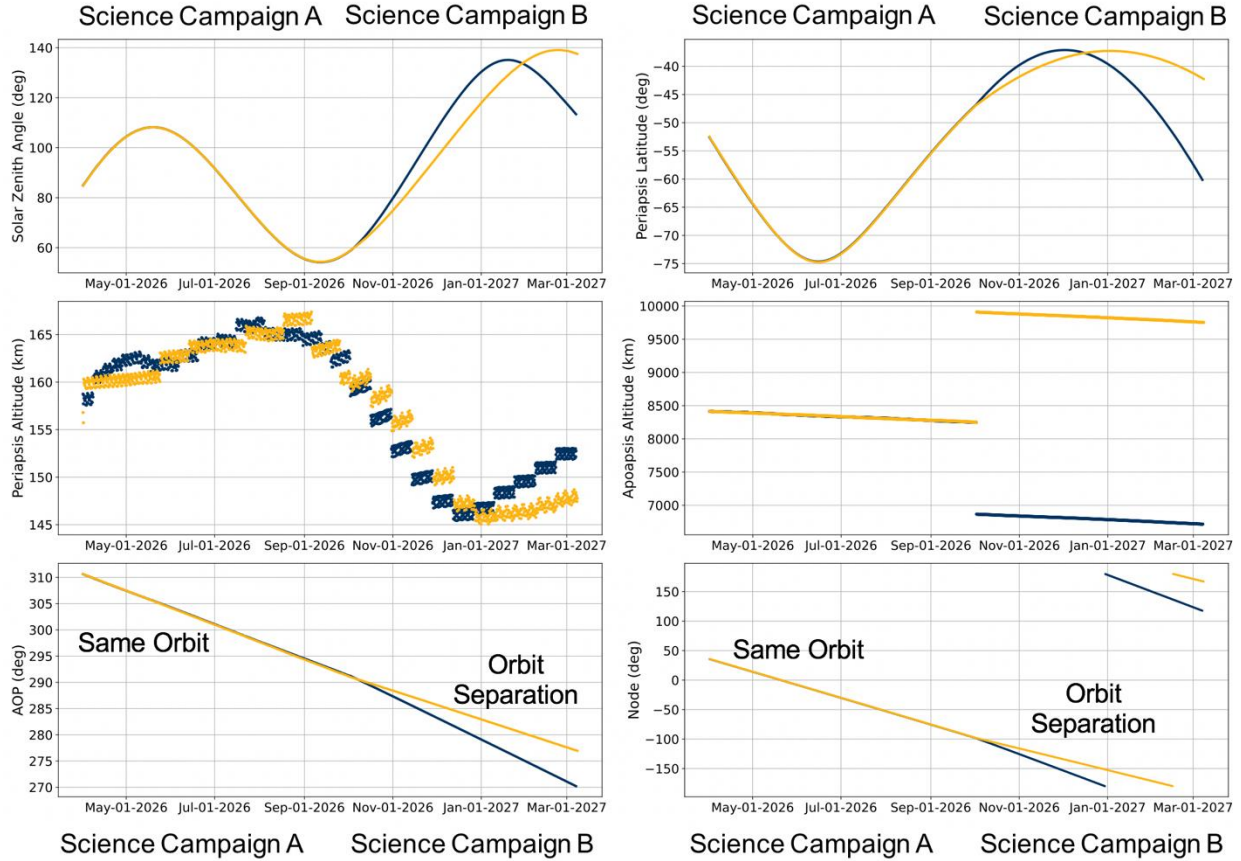
Figure 10. ESCAPEDE's orbit profile for the primary science mission.
