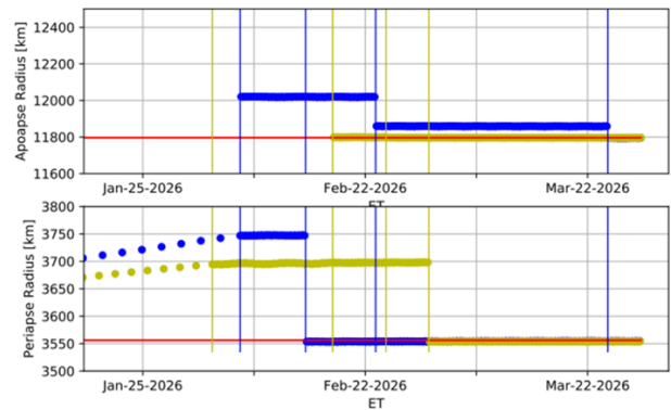
Figure 5. The TSF Phase’s nominal timeline for periapse and apoapse radii. The red lines are the science orbit targets; blue and gold correspond with the appropriate spacecraft.
