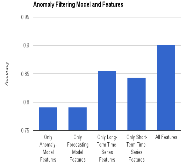
Figure 6: Accuracy of the filtering stage using different types of features.
