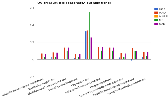
(a) Model performance on TimeSeries with trend.
