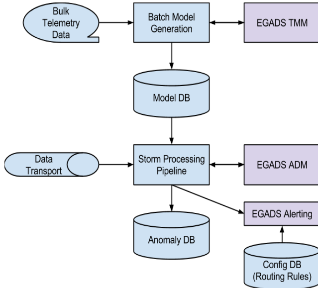
Figure 1: EGADS-YMS Architecture
