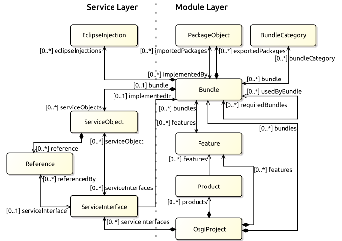
Fig. 1. Class structure of our OSGi model abstraction.
