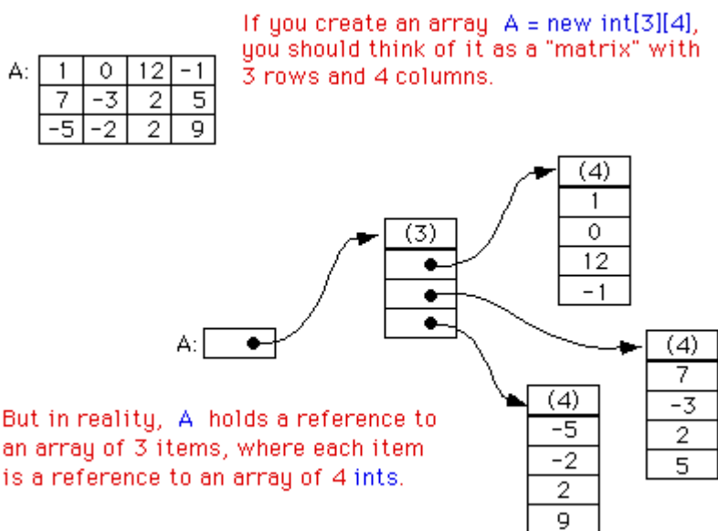
Image source: http://math.hws.edu/eck/cs124/javanotes3/c8/s5.html
