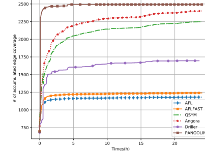
(h) jhead, p_1 = 0.01578, p_2 = 0.03216
