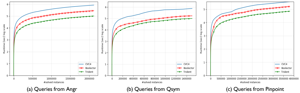
Figure 5: Results of CVC4, BOOLECTOR, and TRIDENT on all solved instances.
