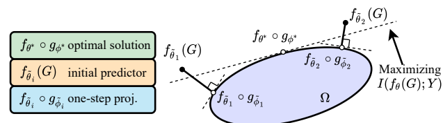
Figure 4. Post-hoc methods just perform one-step projection to the information-constrained space, which is always suboptimal and the interpretation performance is sensitive to the pre-trained model.
