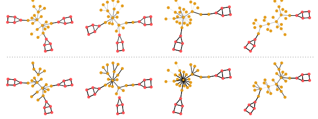
Figure 3. Visualizing attention (normalized to [0, 1] ) of GSAT (first row) and masks of GraphMask (Schlichtkrull et al., 2021) (second row) on a motif example, where graphs with three house motifs and graphs with two house motifs represent two classes. Samples may contain disconnected interpretable subgraphs, while GSAT detects them accurately. More details can be found in Appendix C.4.
