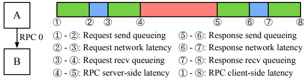
Figure 2: RPC latency breakdown. Red bars: RPC server-side latency, blue bars: network latency, green bars: application queuing.
