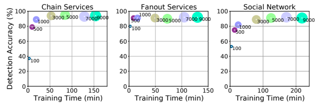
Figure 15: Sensitivity to training set size (samples) for the two synthetic services and the Social Network.
