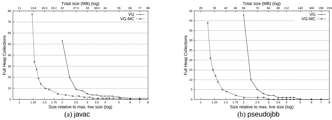
Figure 7: Number of full heap collections performed for javac and pseudobjb
