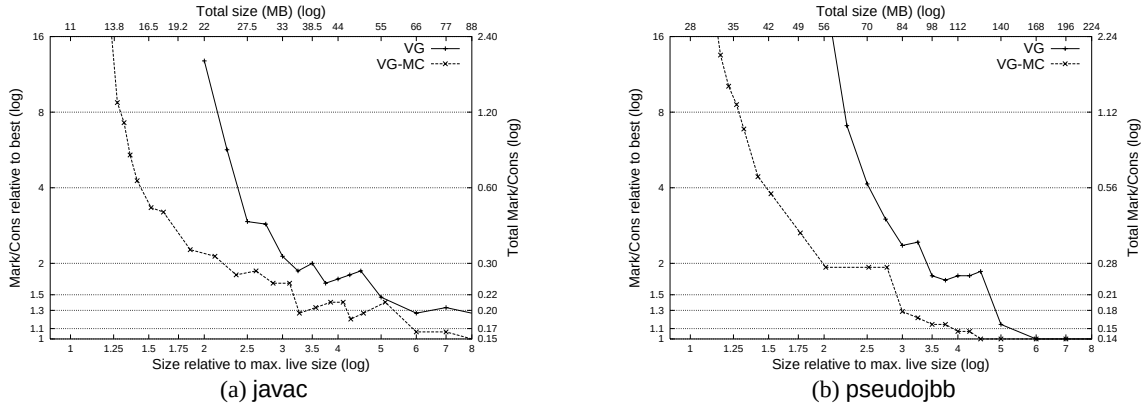
Figure 8: Relative Mark/Cons ratio for javac and pseudobjb
