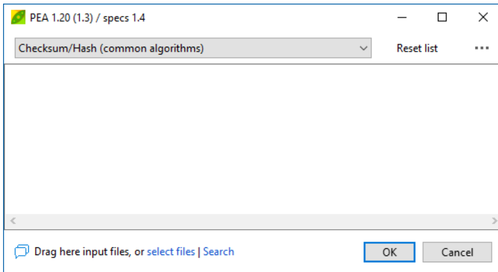
Image 29: PeaUtils
