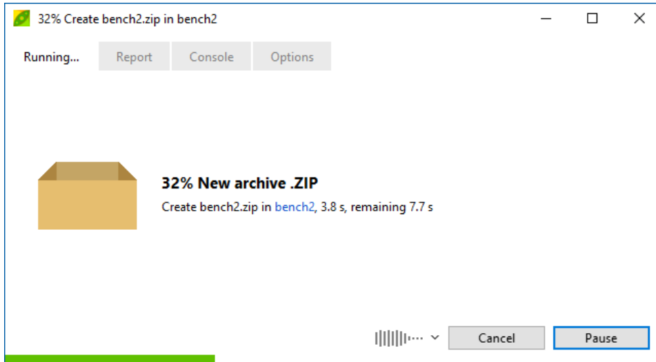
Image 27: PeaLauncher instance
