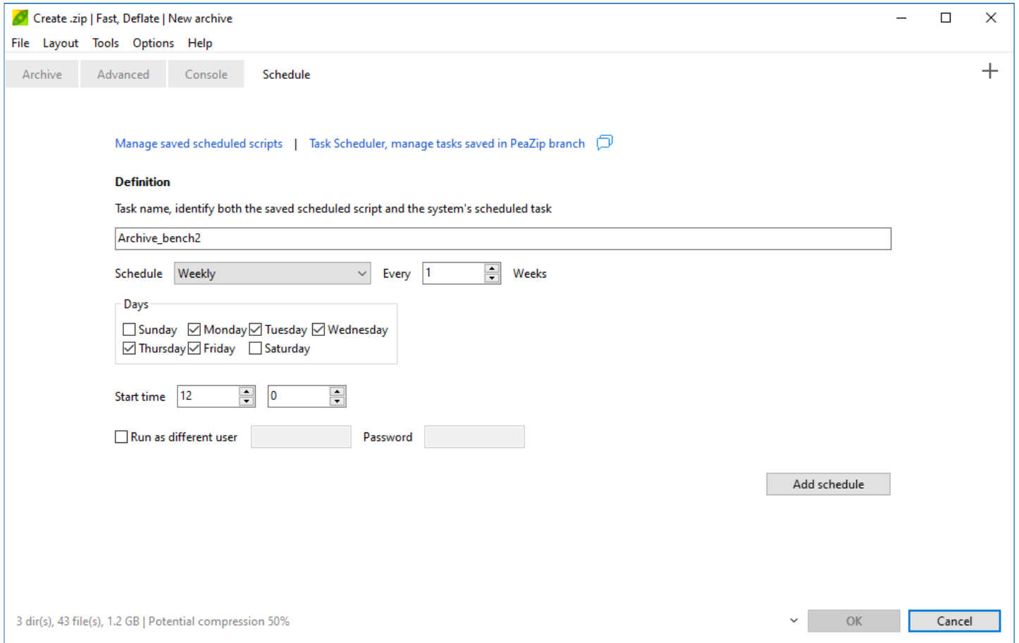
Image 26: Schedule tab
