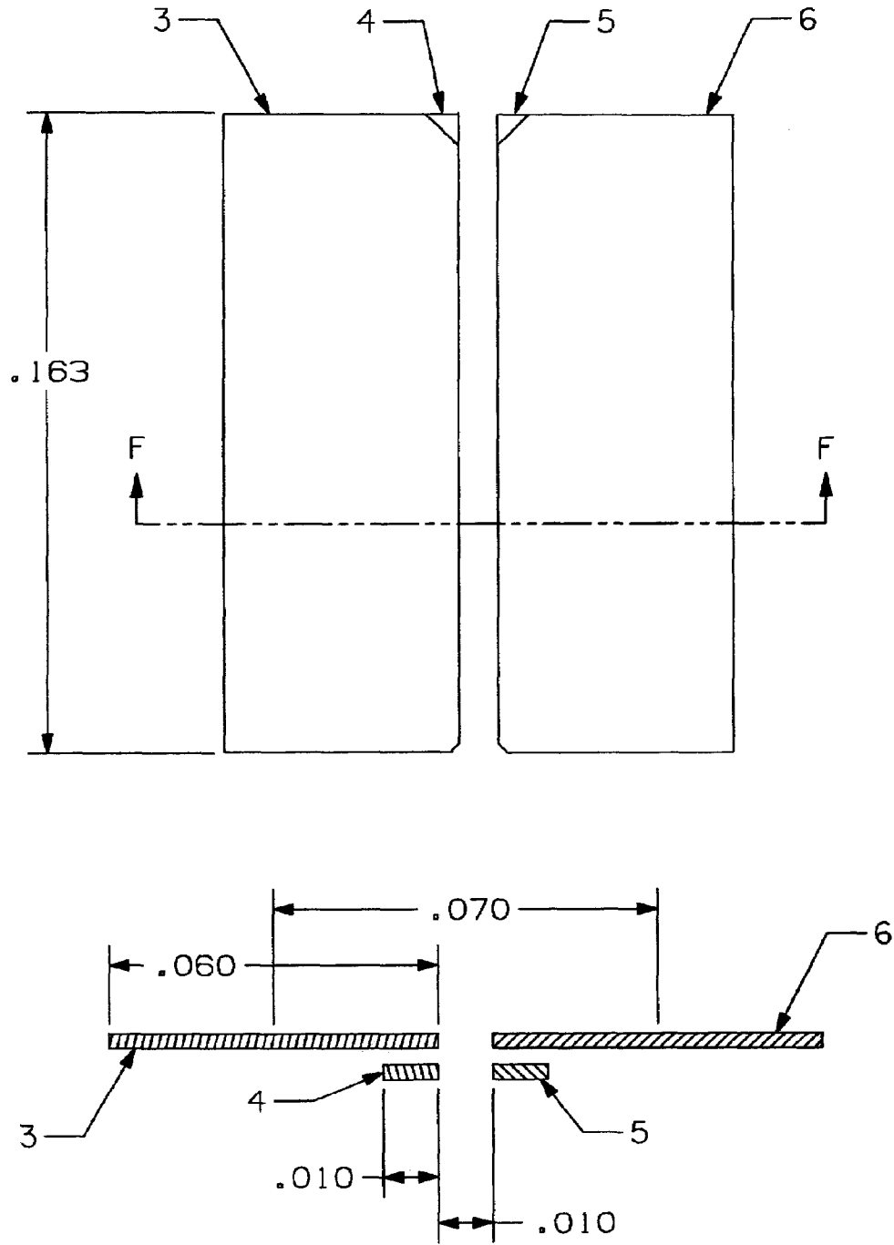
SECTION F-F
