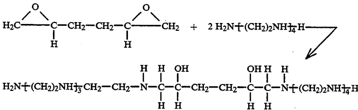
Eq.1
