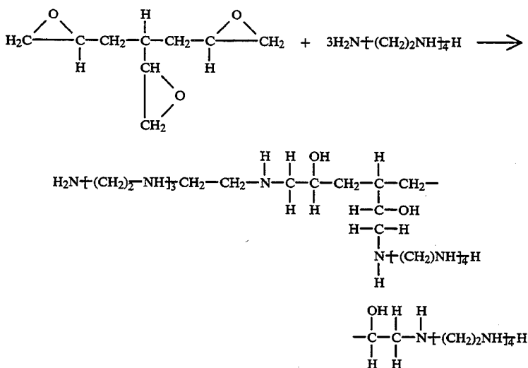
Equation 2
