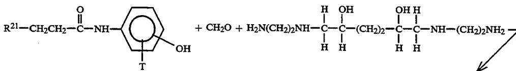
Equation B
