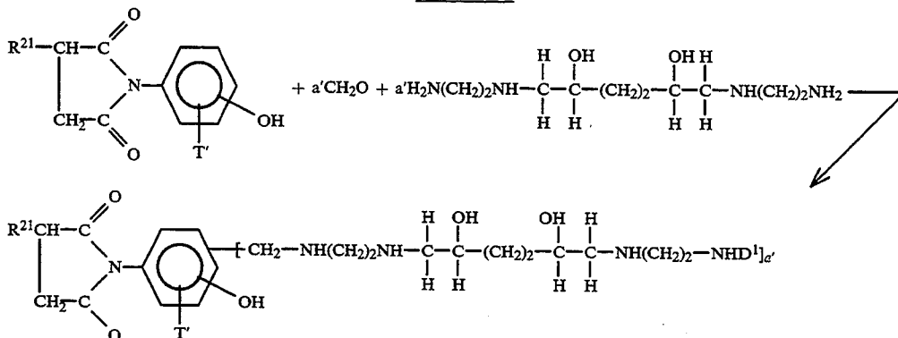
Equation A
