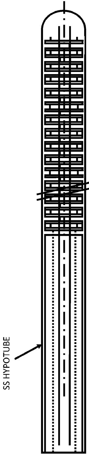
HOLLOW TUBE GUIDEWIRE WITH CORE WIRE AND INTERSPERSED ELASTOMER FILLING AND HYPOTUBE PROXIMAL.
