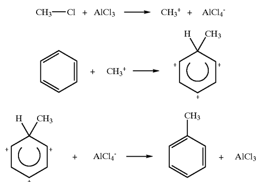
FIG. 3- Reaction Mechanism for Friedel-Crafts Alkylation
