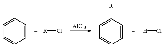
FIG. 2-Net Reaction For Friedel-Crafts Alkylation
