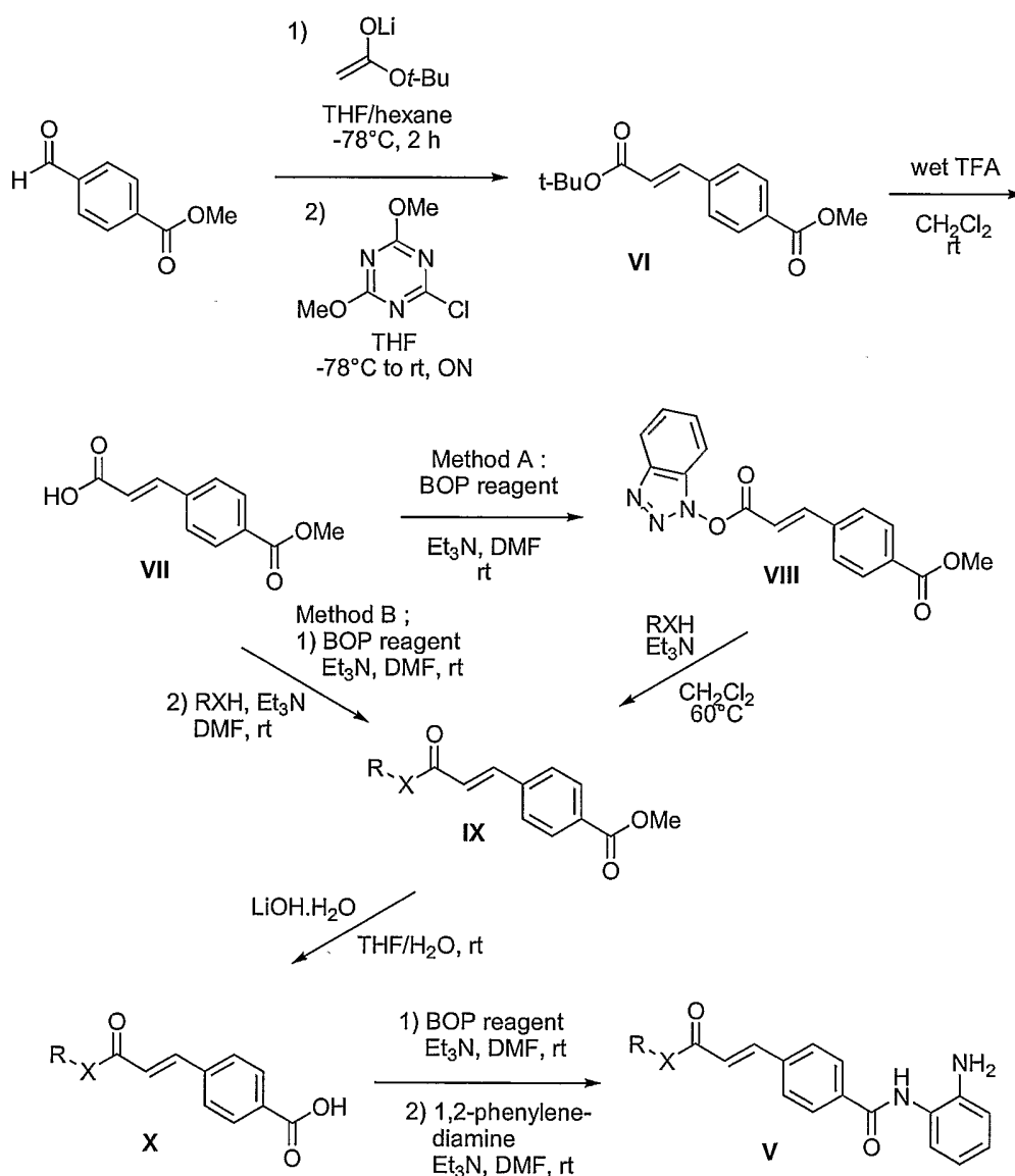
Scheme 3
