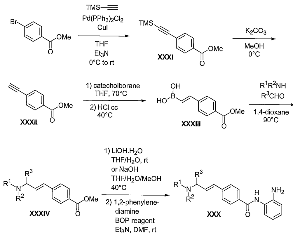
Scheme 11
