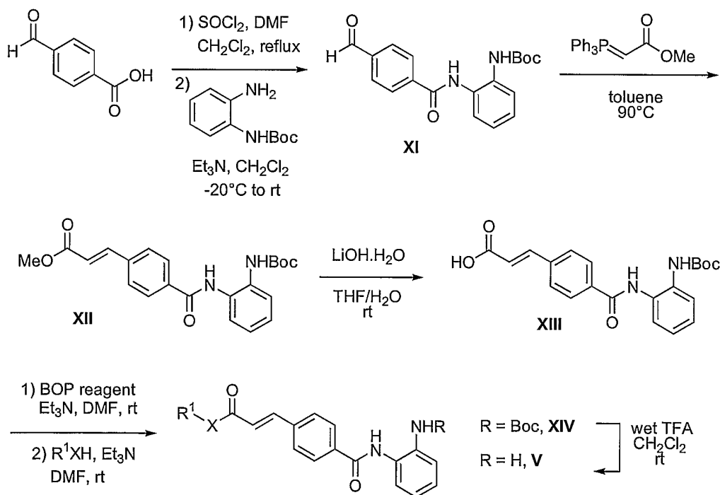
Scheme 4
