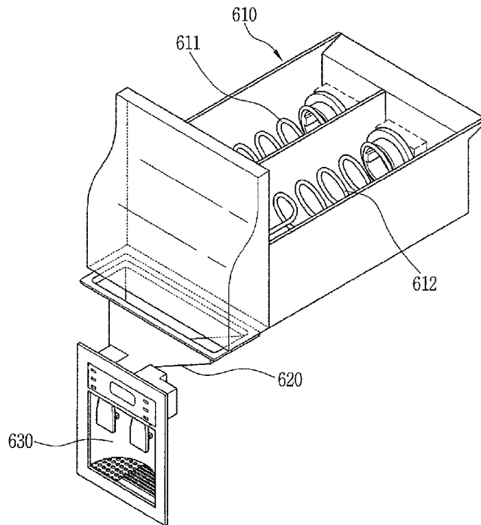
Figure 7 PRIOR ART
