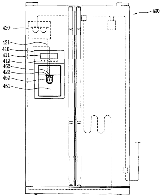
Figure 4 Prior Art
