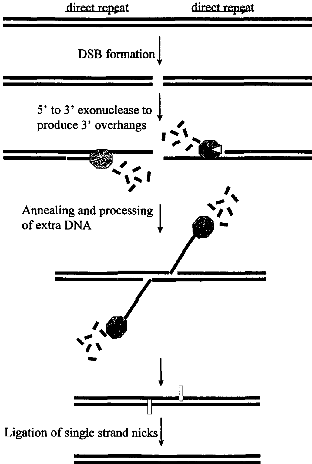
Figure 3. Single strand annealing model
