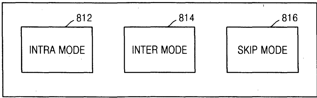
'PREDICTION MODE'-INFORMATION (810)
