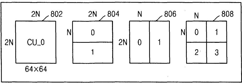
'PARTITION TYPE'-INFORMATION (800)
