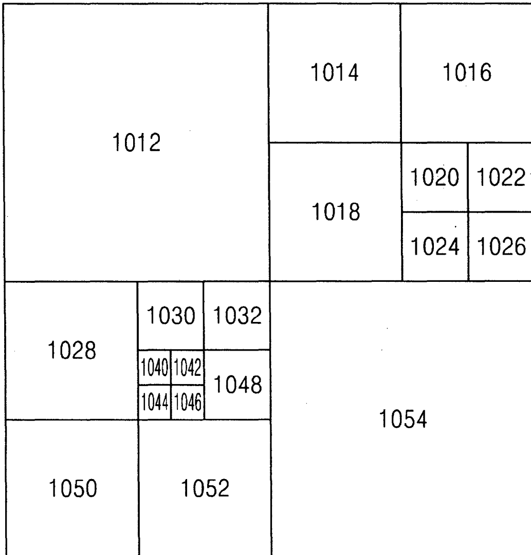
CODING UNITS (1010)
