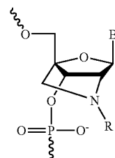
Amino-LNA R = -H, -CH 3
