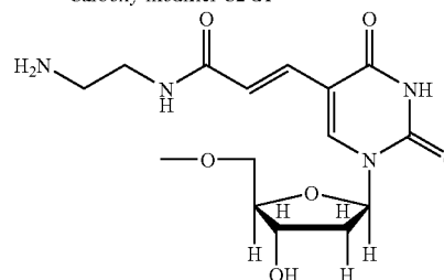
Amino modifier C2 dT
