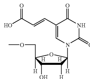
Carboxy-modifier C2 dT
