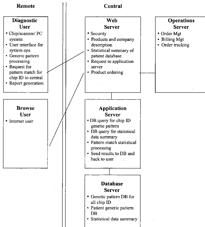
System Architecture
