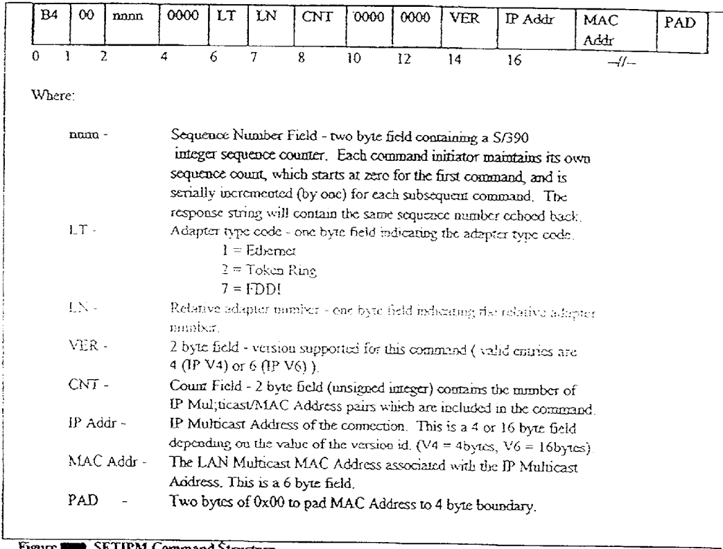
Figure 6A SETIPM Command Structure
