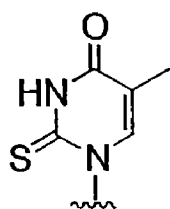
2-thio-T
