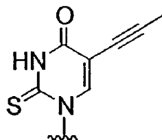
2-thio-5-propynyl-U
