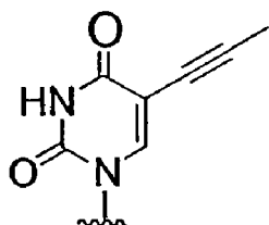
5-propynyl-U
