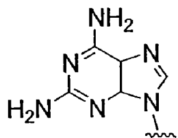
N9-(2,6,-diaminopurine)
