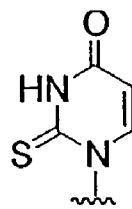
2-thio-U
