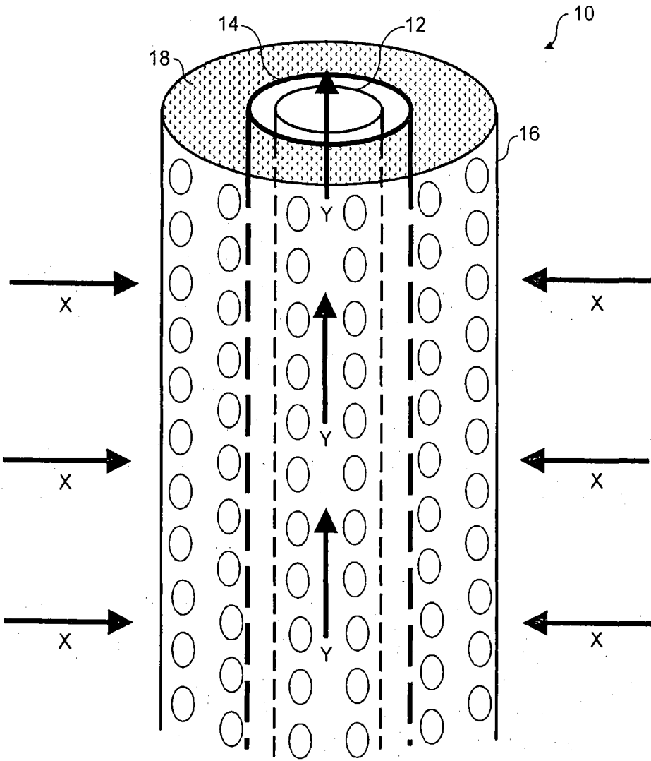
FIG. 1 PRIOR ART
