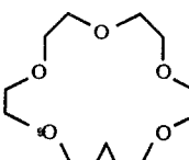
(5) Dibenzo-18-crown-6
