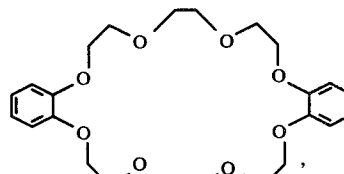
(8) Dibenzo-30-crown-10
