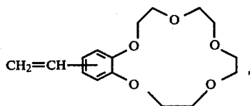
(22) 1,2-Vinylbenzo-18-crown-6
