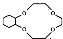
(15) 1,2-Decalyl-15-crown-5
