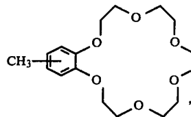
(19) 1,2-Methylbenzo-5,6-methylbenzo-18-crown-6
