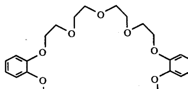
(8) Dibenzo-30-crown-10
