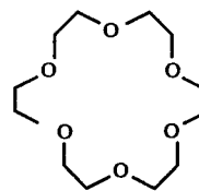
(1) 18-Crown-6
