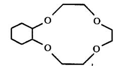
(15) 1,2-Decalyl-15-crown-5
