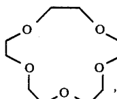
(4) 18-Crown-5
