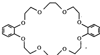
(8) Dibenzo-30-crown-10
