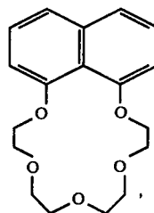
(18) 1,2-Methylbenzo-18-crown-6
