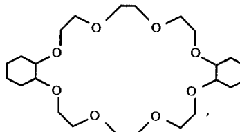
(14) Cyclohexyl-12-crown-4
