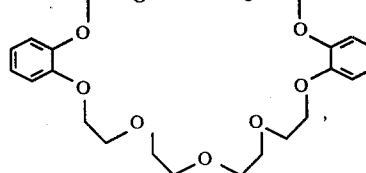
(9) Tribenzo-18-crown-6
