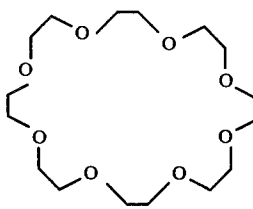
and (36) 24-Crown-8
