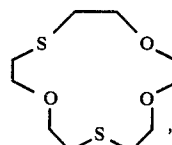
(3) 15-Crown-5
