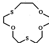
(2) Dithia-15-crown-5
