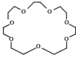
and (36) 24-Crown-8
