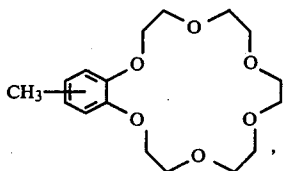
(19) 1,2-Methylbenzo-5,6-methylbenzo-18-crown-6
