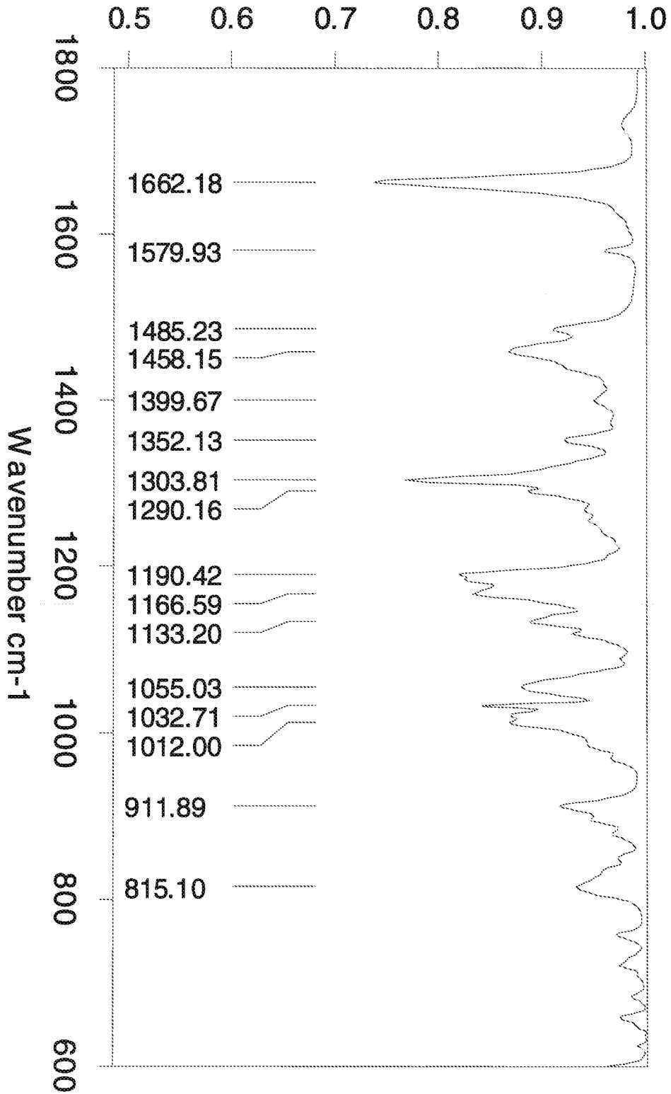
Figure 2. FT-IR of Crystalline Form A
