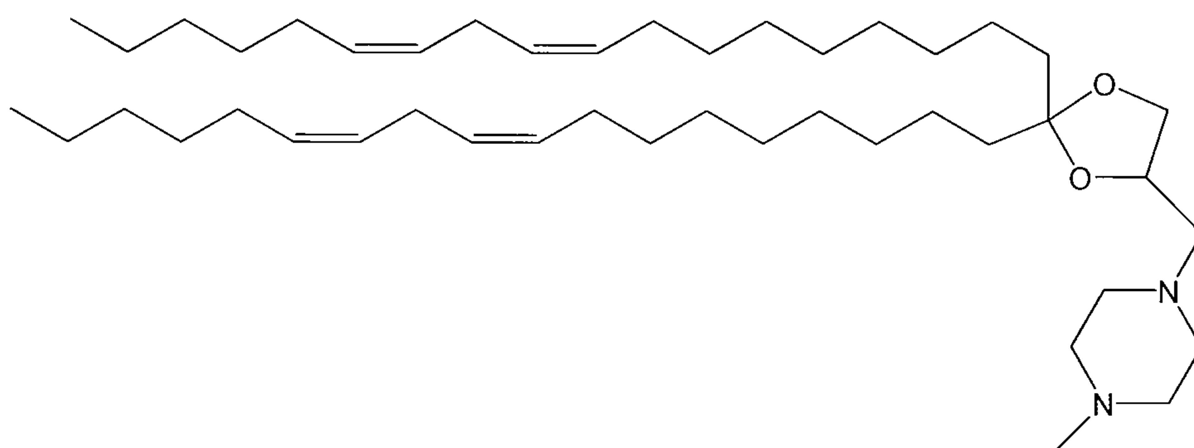
D-Lin-K-N-methylpiperzine;
