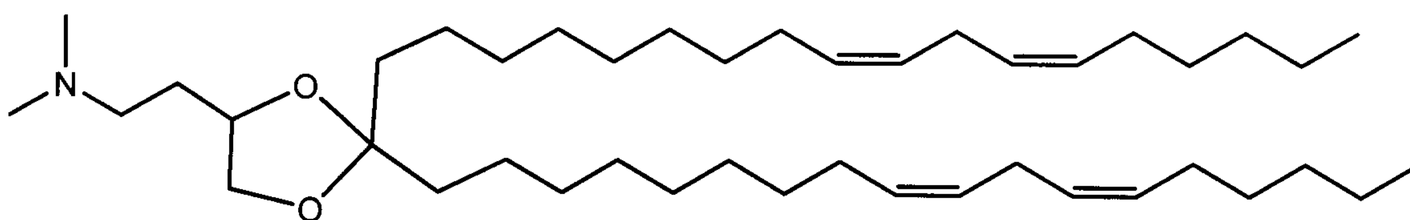
DLin-K-C2-DMA.
