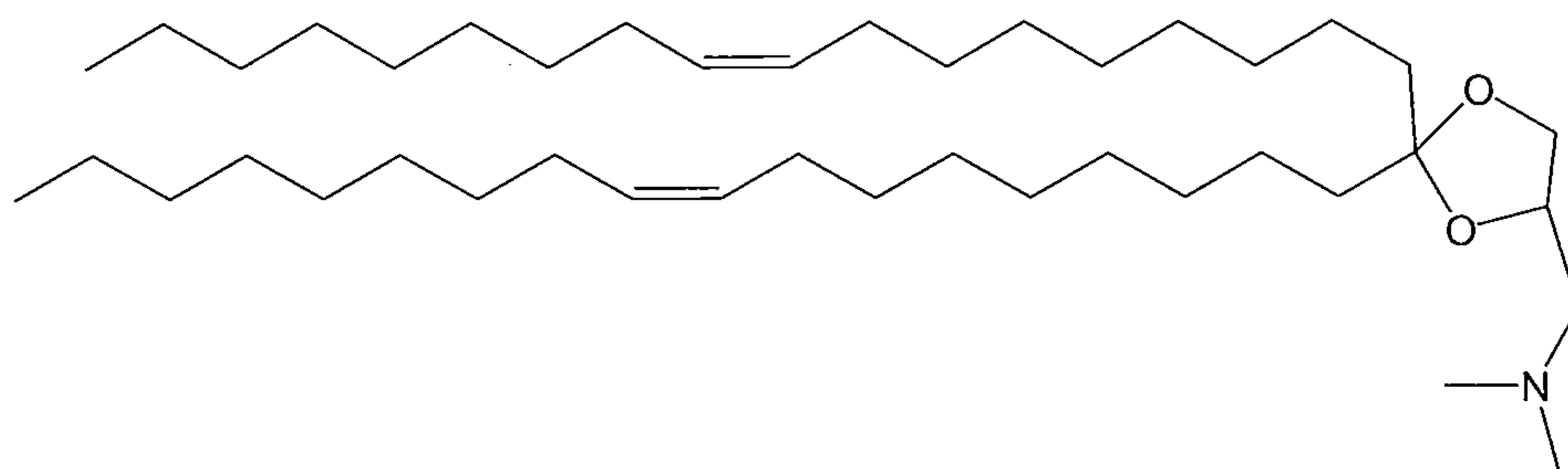
DO-K-DMA
