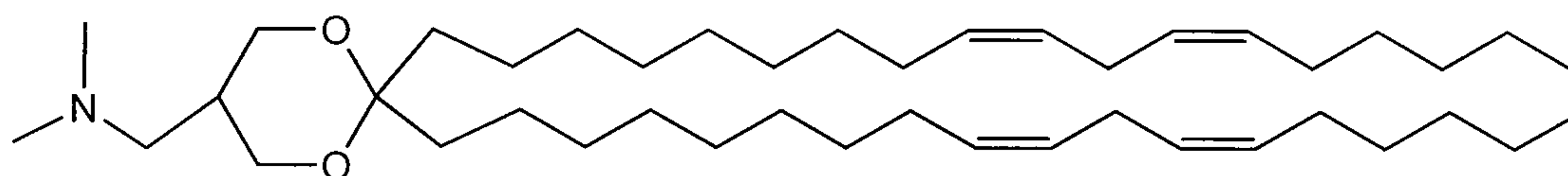
DLin-K6-DMA;
