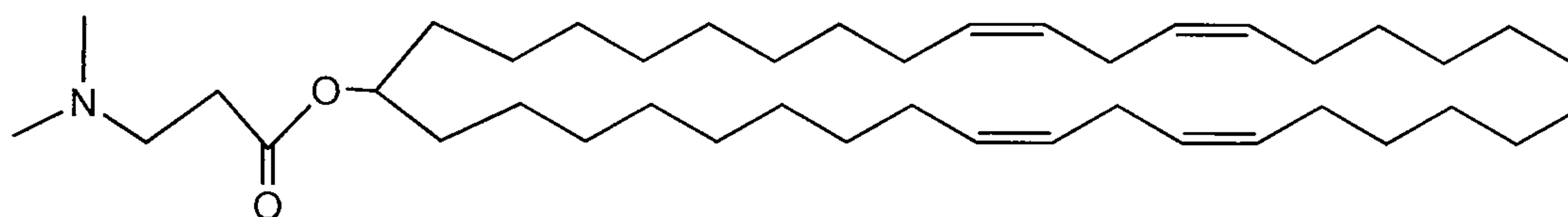
DLin-M-K-DMA; or
