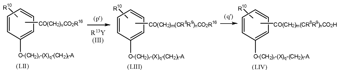
Reaction Scheme 7
