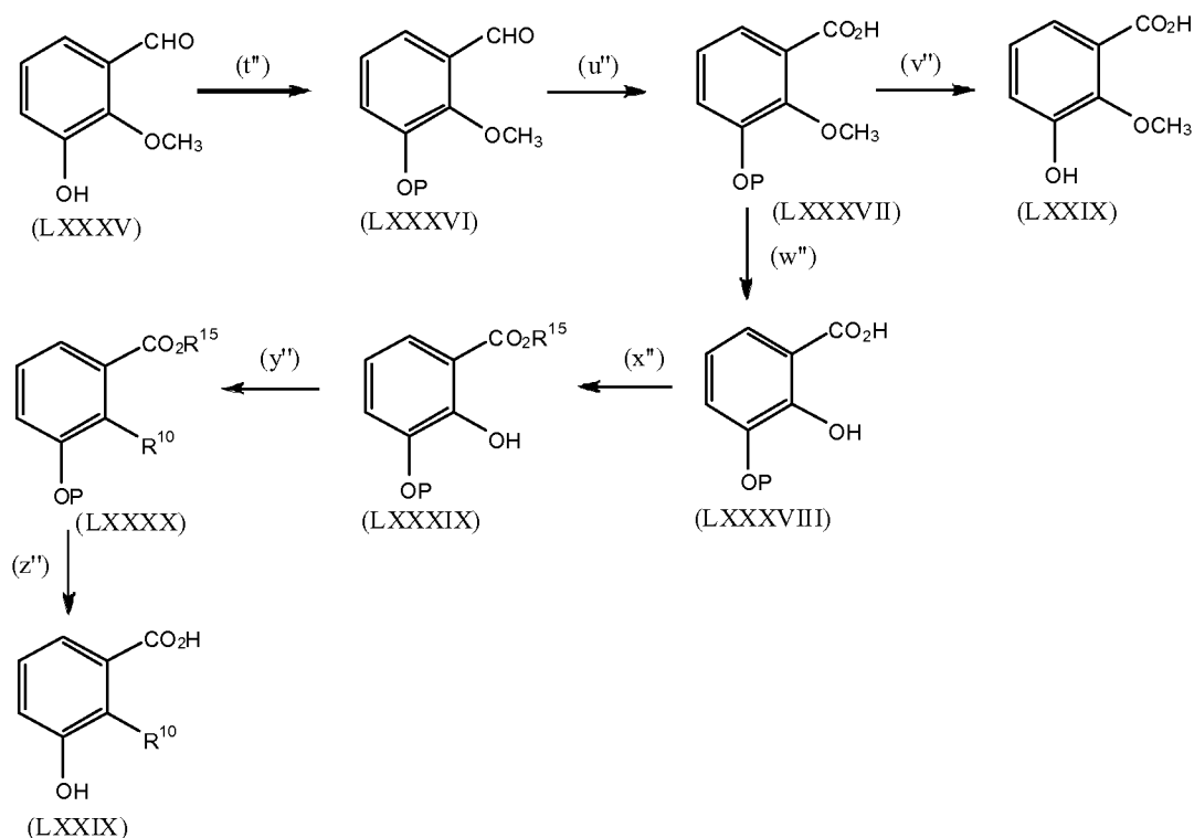
Reaction Scheme 18
