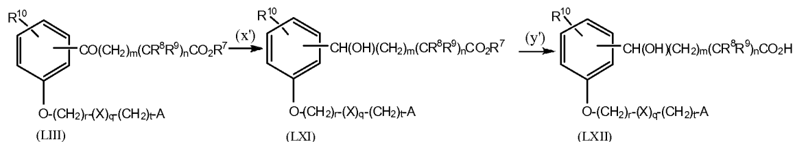
Reaction Scheme 11
