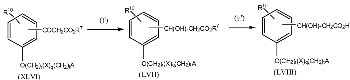
Reaction Scheme 9
