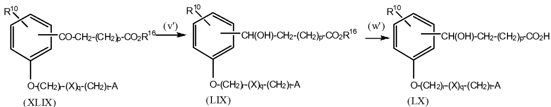
Reaction Scheme 10
