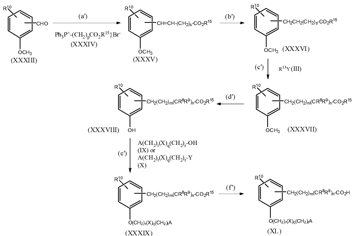
Reaction Scheme 3
