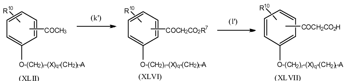
Reaction Scheme 5
