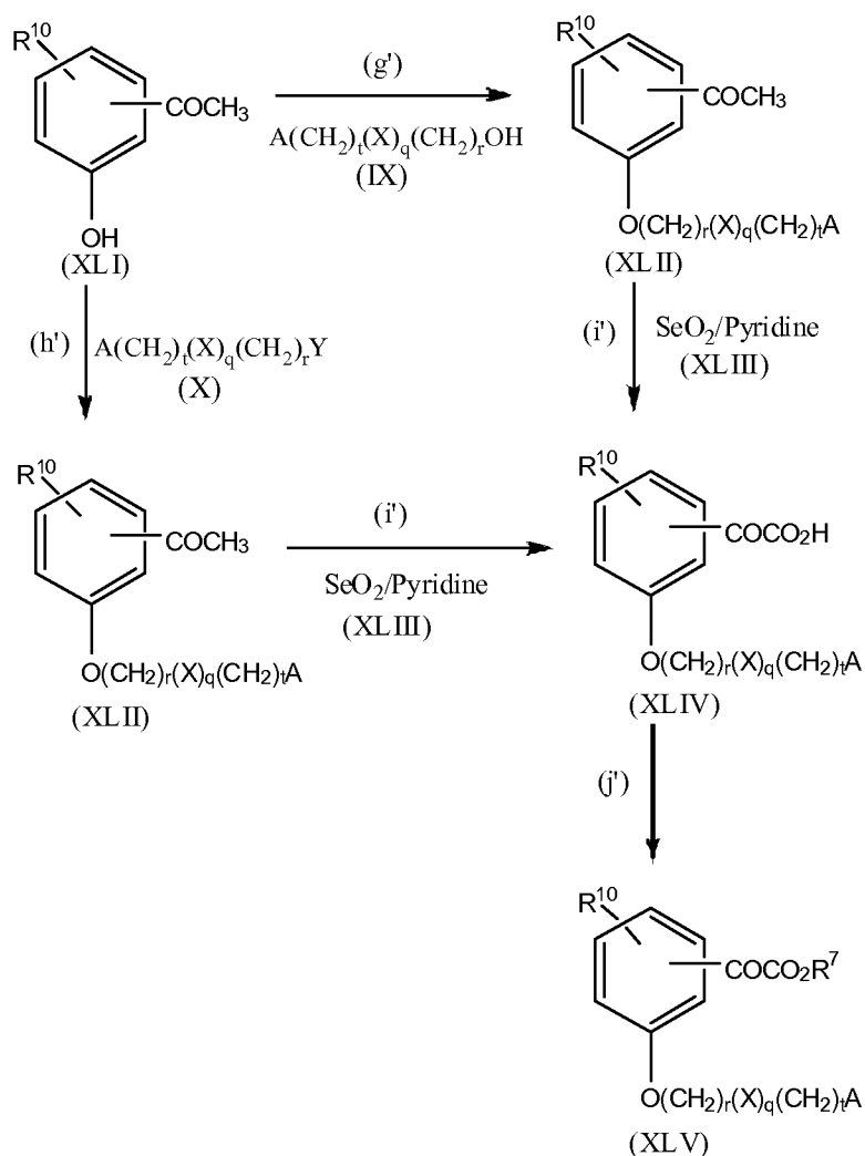
Reaction Scheme 4
