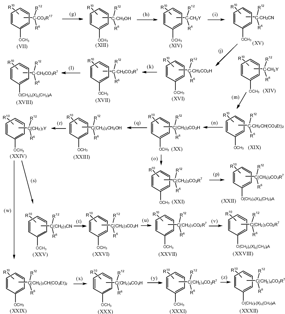
Reaction Scheme 2
