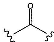
carbonyl
