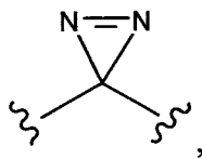
diazirine
