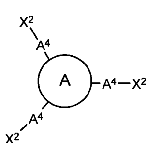
(XIII)
