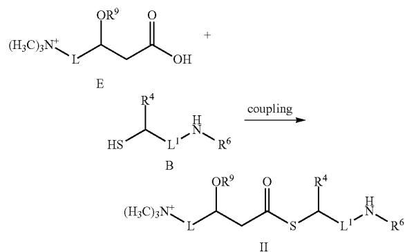
Scheme 3: Coupling of Intermediate acid E and thiol B
