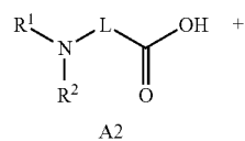
Scheme 1a: Synthesis of intermediates of Formula A
